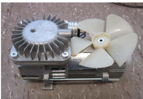
New compressor
