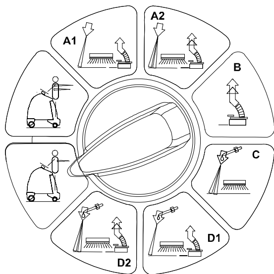
ROTARY SWITCH
