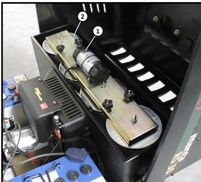
FIG. 16 ELECTRIC FILTER SHAKER
