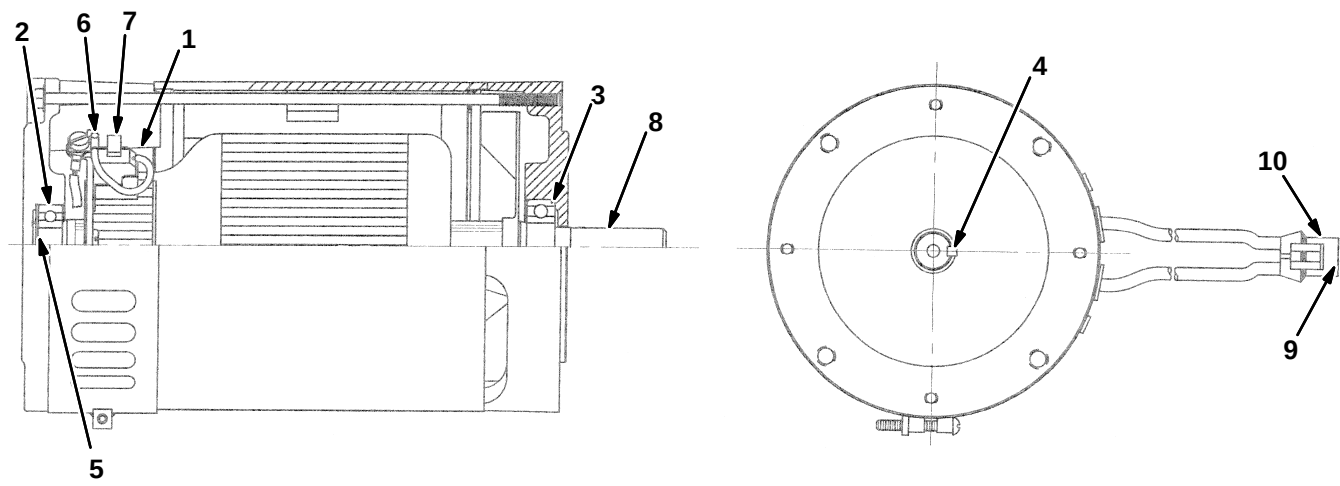
Fig. 4 – Electric Motor Breakdown, 386050
