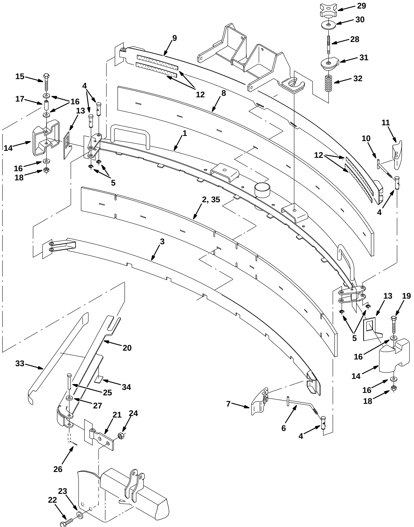
Fig. 34 – Max Pro 1000 Rear Squeegee Group (005000– )
