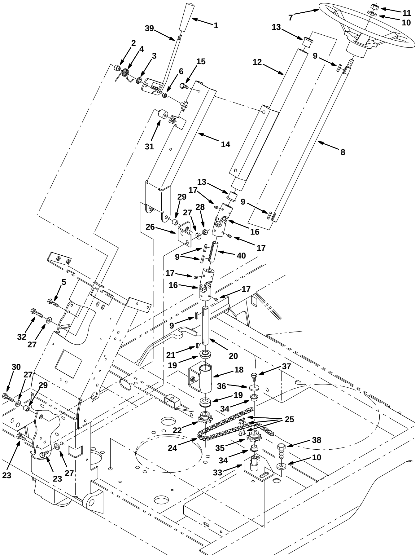
Fig. 8 - Steering Group
