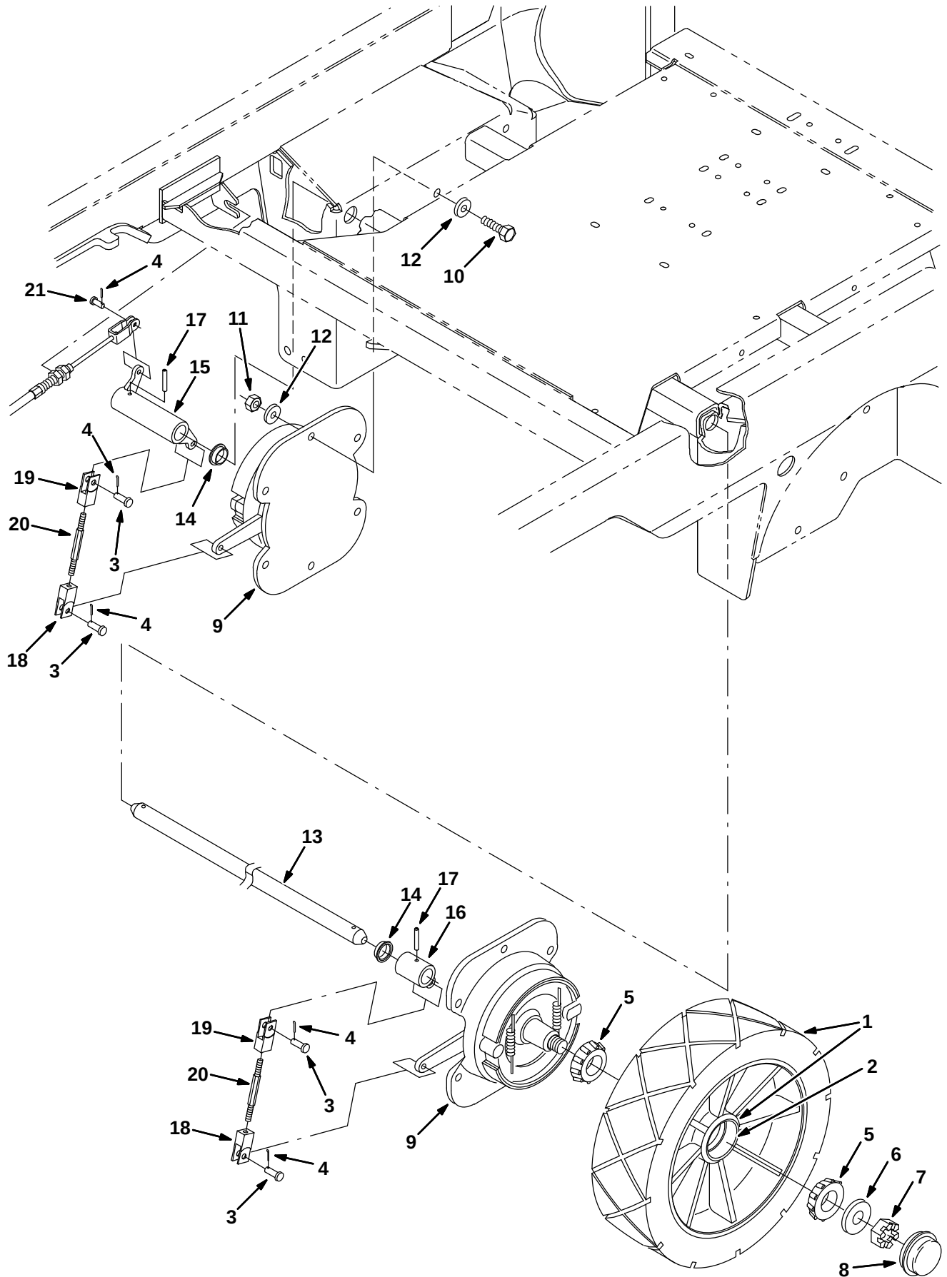
Fig. 13 – Wheel And Brake Group, Rear
