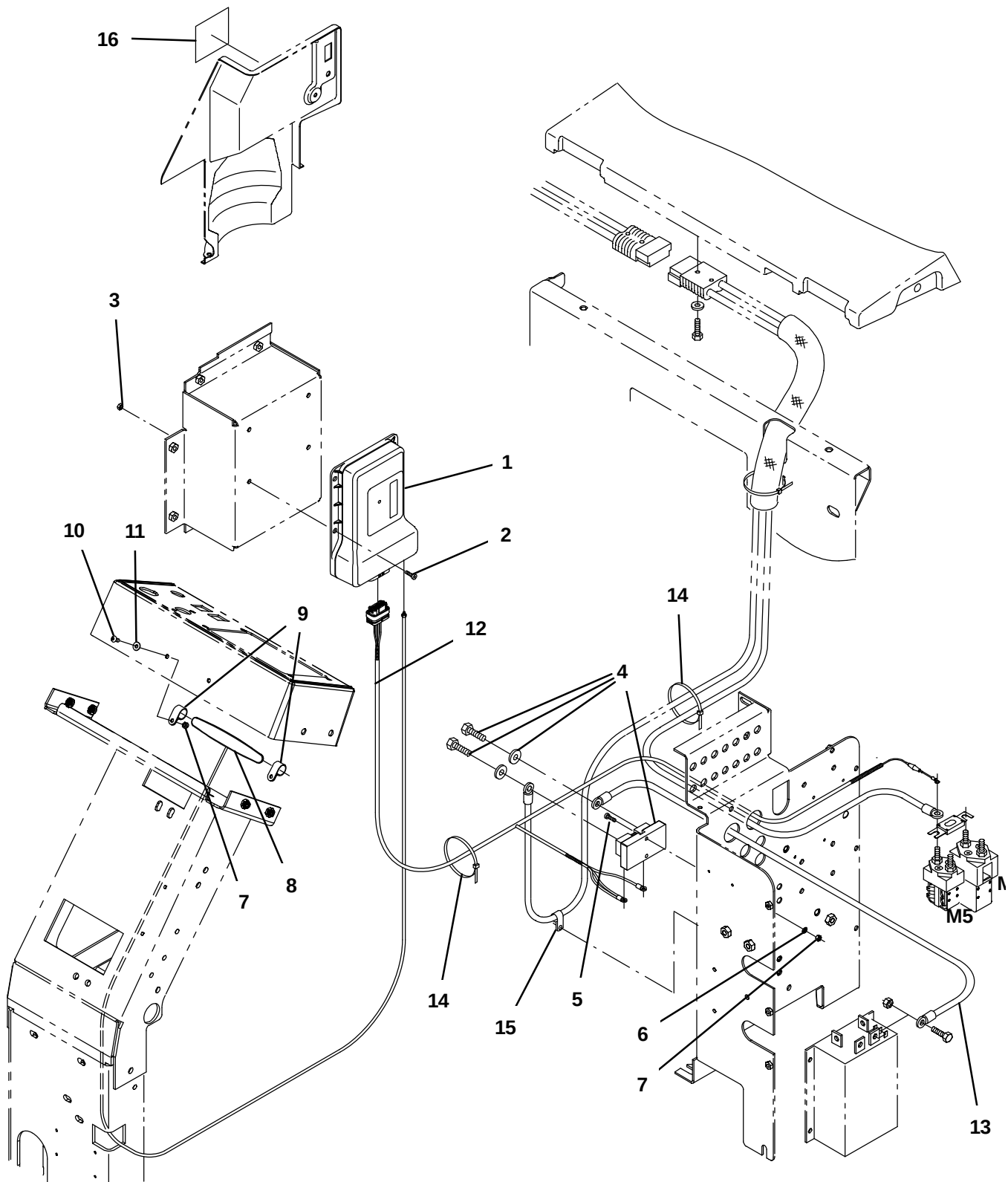
Fig. 74 – Telemetry Group (005974- )
