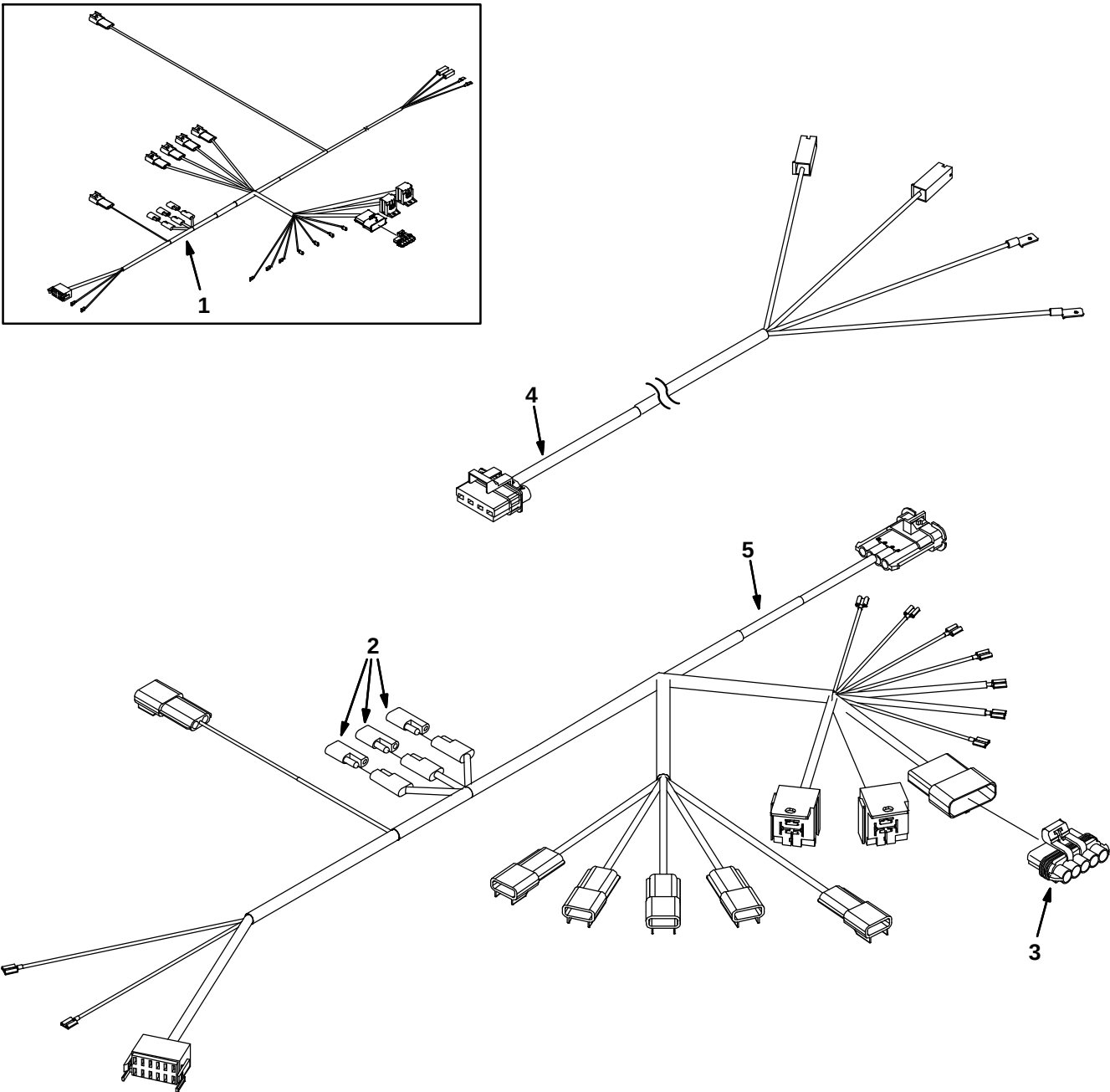
Fig. 46 – Electrical Wire Harness Group, FaST (000000–003746)
