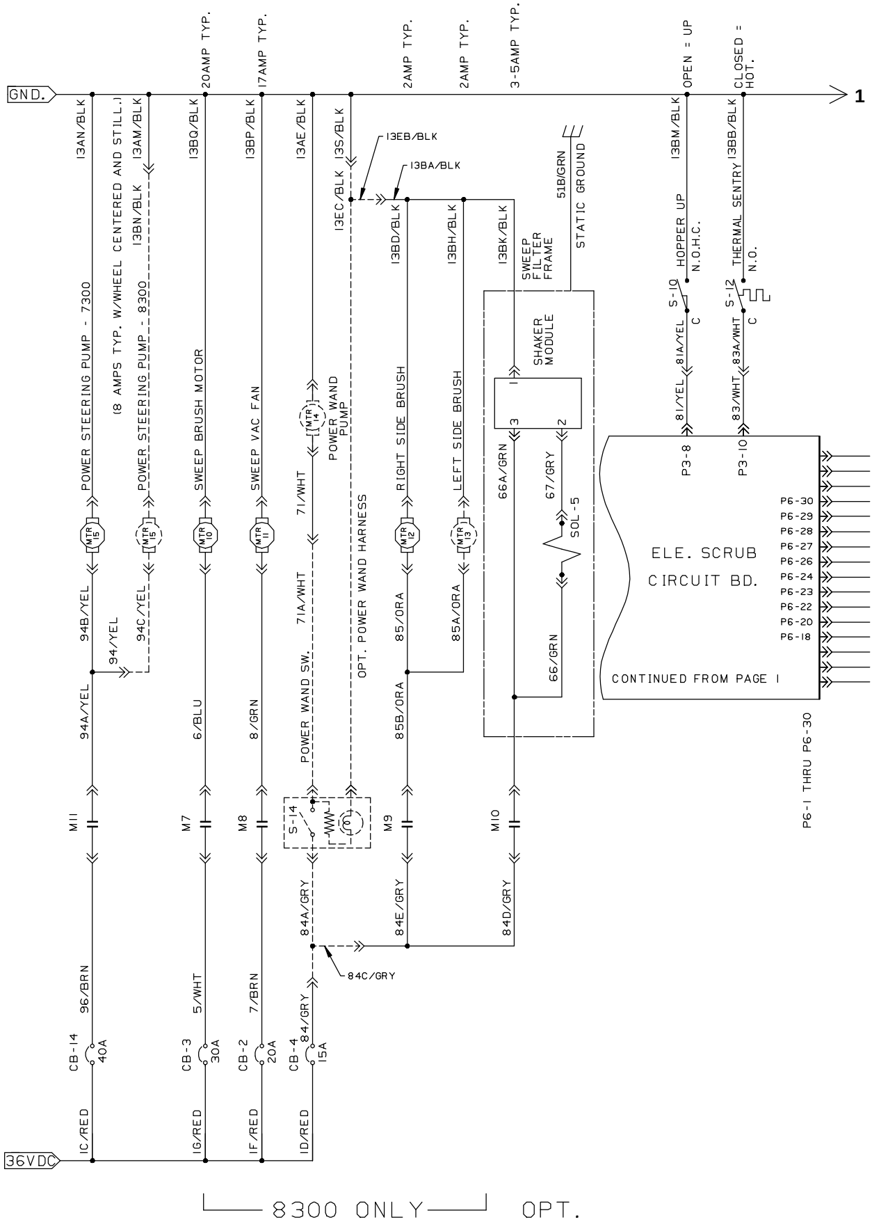
Fig. 43 – Electrical Schematic (000000–003746)
