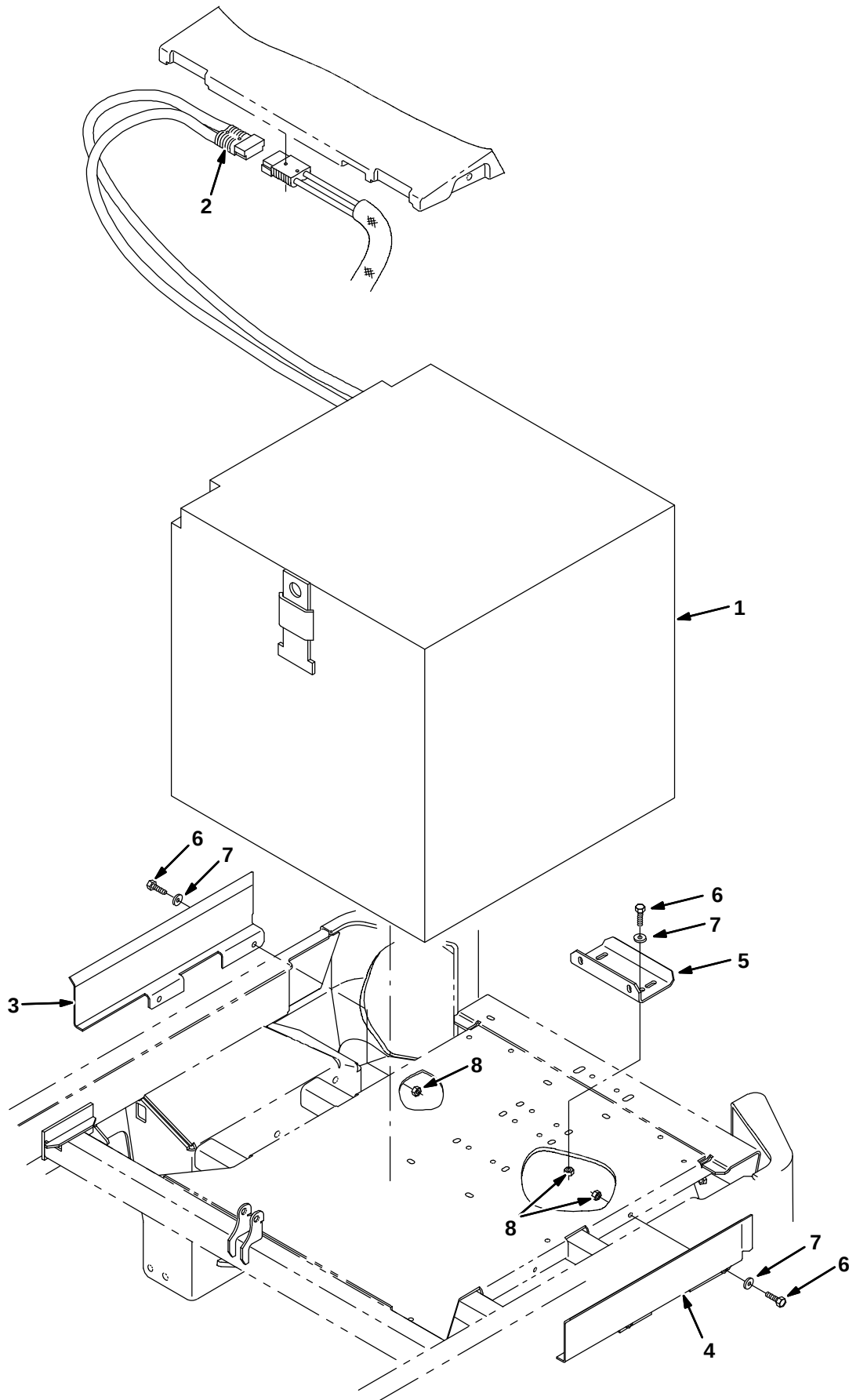
Fig. 80 – Battery Kit, 600AH (005000- )
