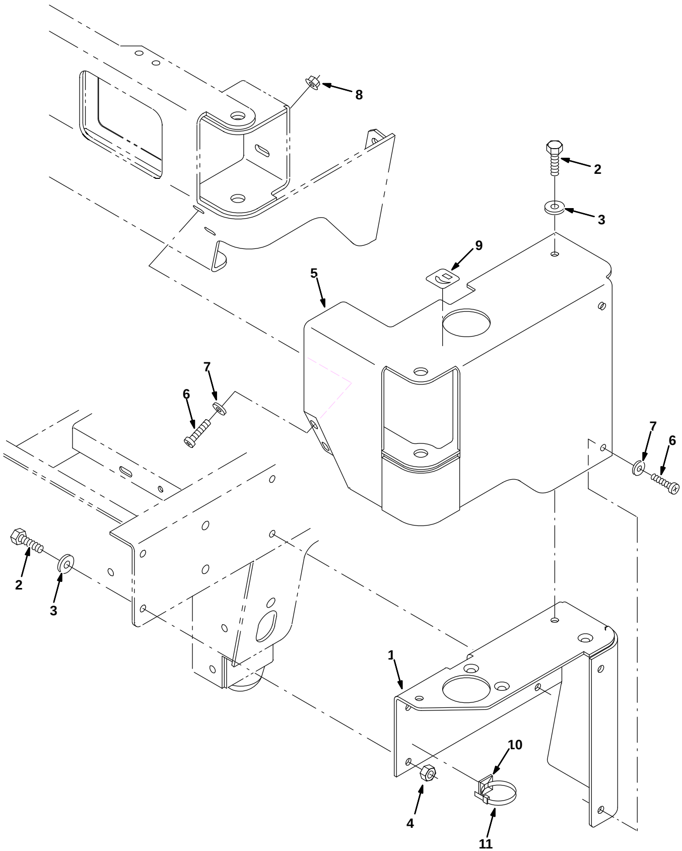
Fig. 22 – Left Side Brush Mount Group
