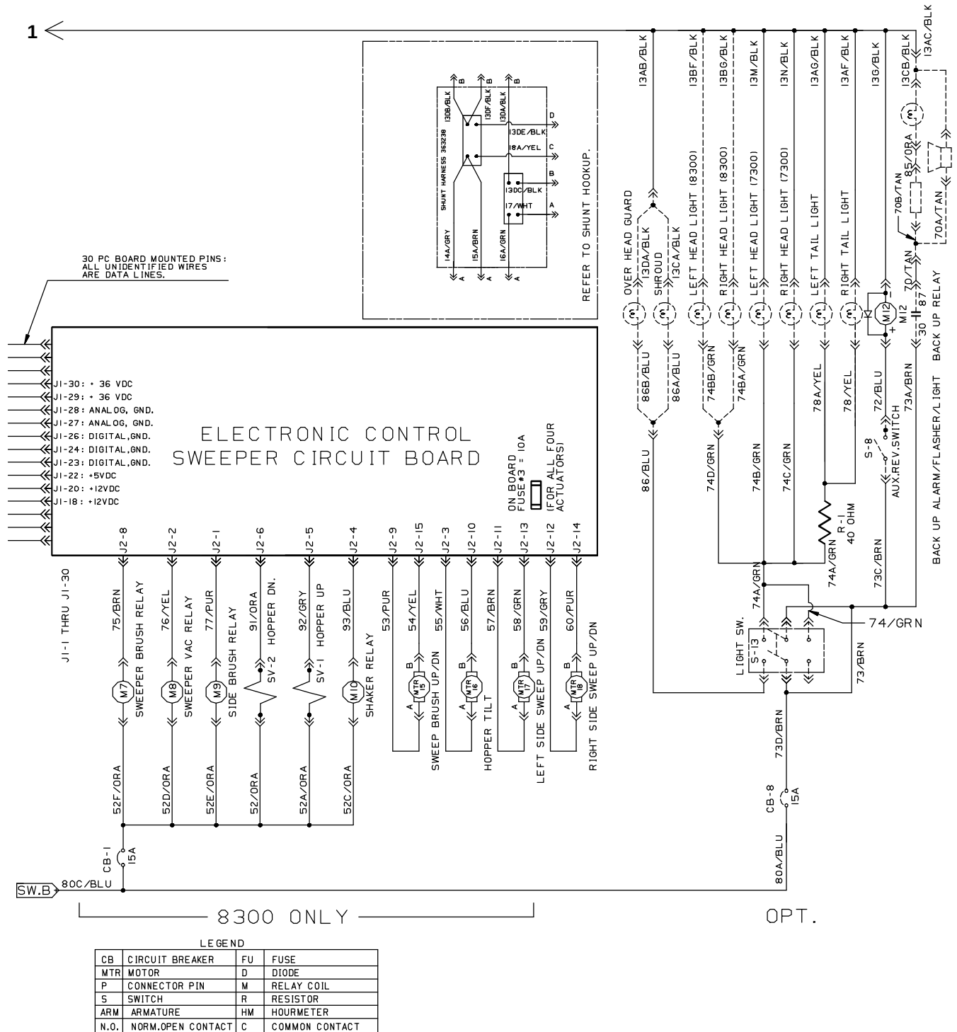
Fig. 43 – Electrical Schematic (000000-003746)
