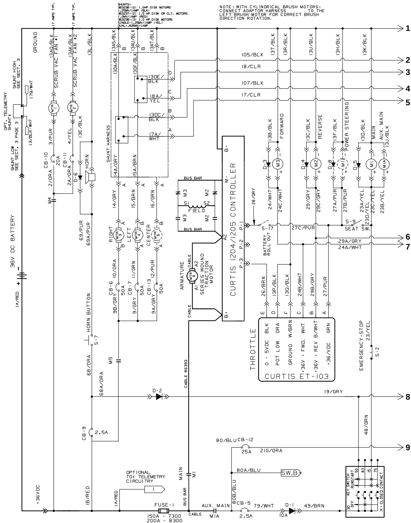
Fig. 44 – Electrical Schematic (003747– )
