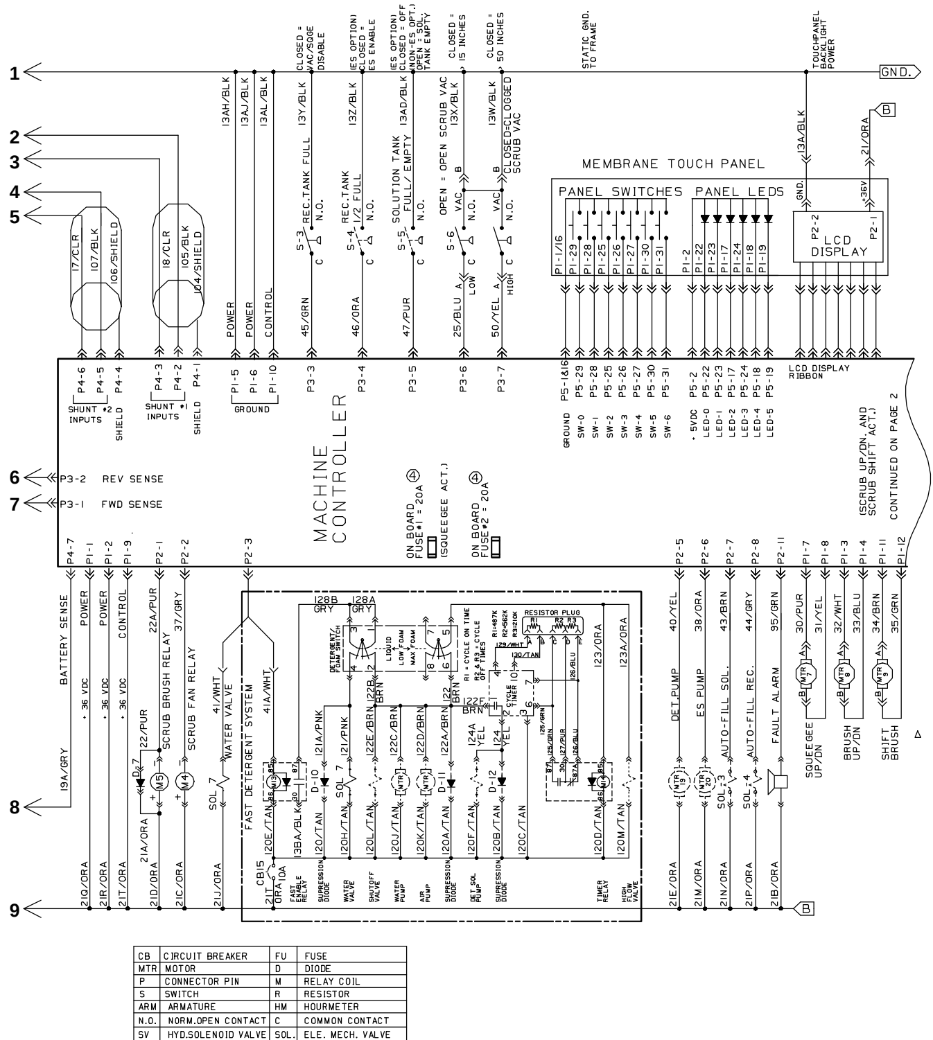
Fig. 43 – Electrical Schematic (000000-003746)
