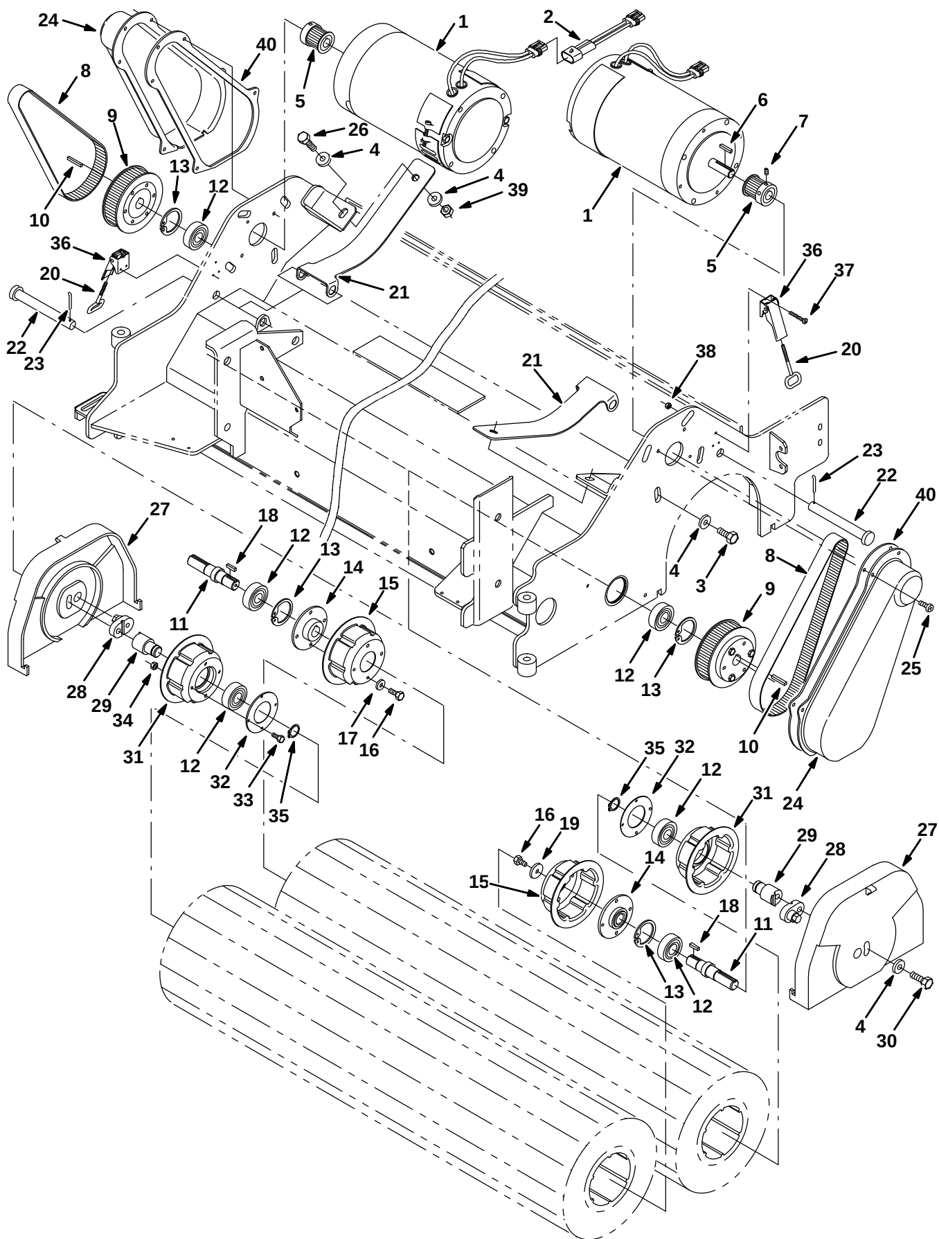
Fig. 42 – Max Pro 1200 (Cylindrical Brush) Scrub Head Drive Group
