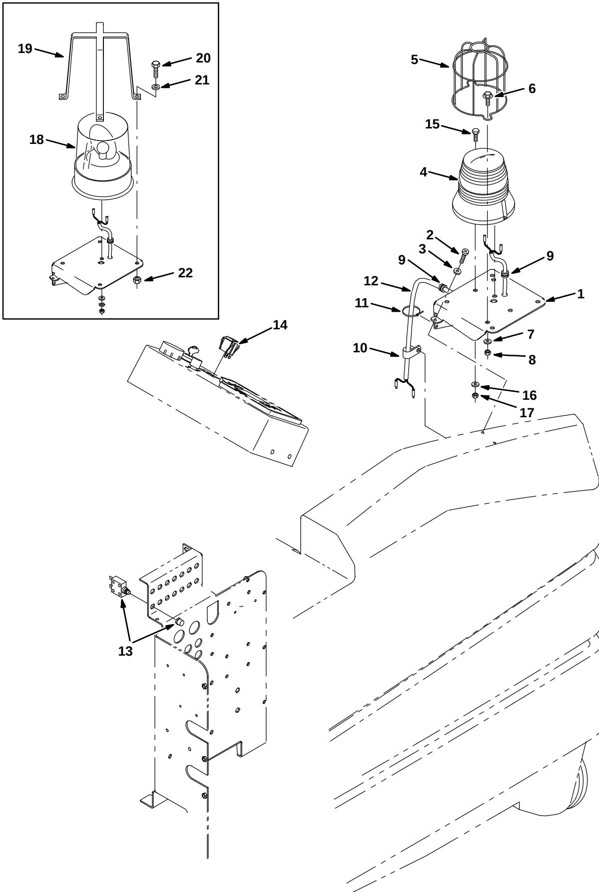
Fig. 2 – Revolving Light Kit (005000– )
