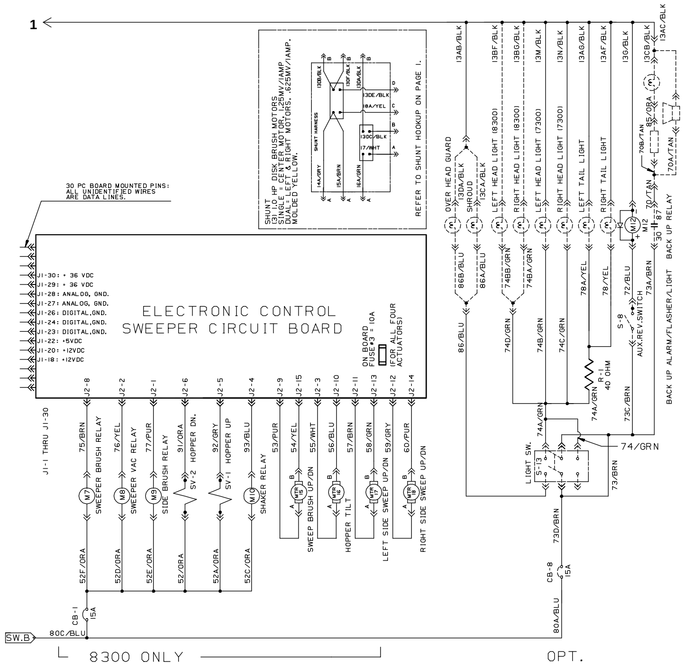
Fig. 44 – Electrical Schematic (003747– )
