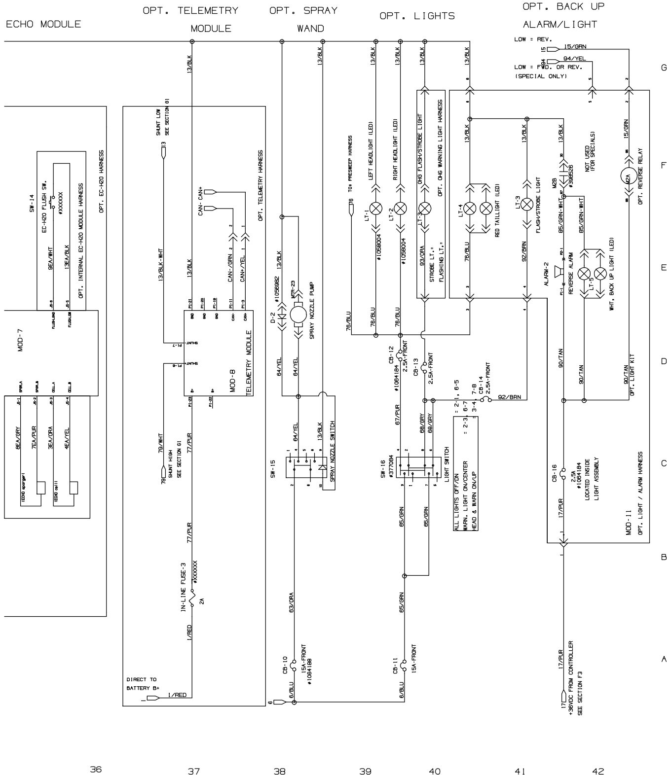
Fig. 33 – Electrical Schematic (011000-012999)
