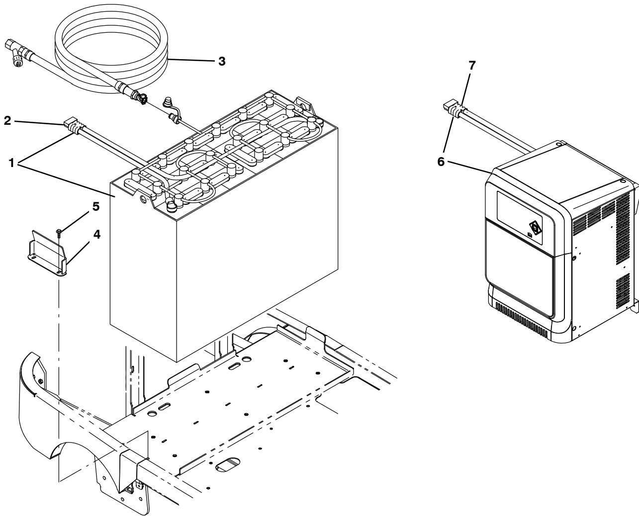
Fig. 45 – Battery and Charger Group, 930AH, Opportunity Charging
