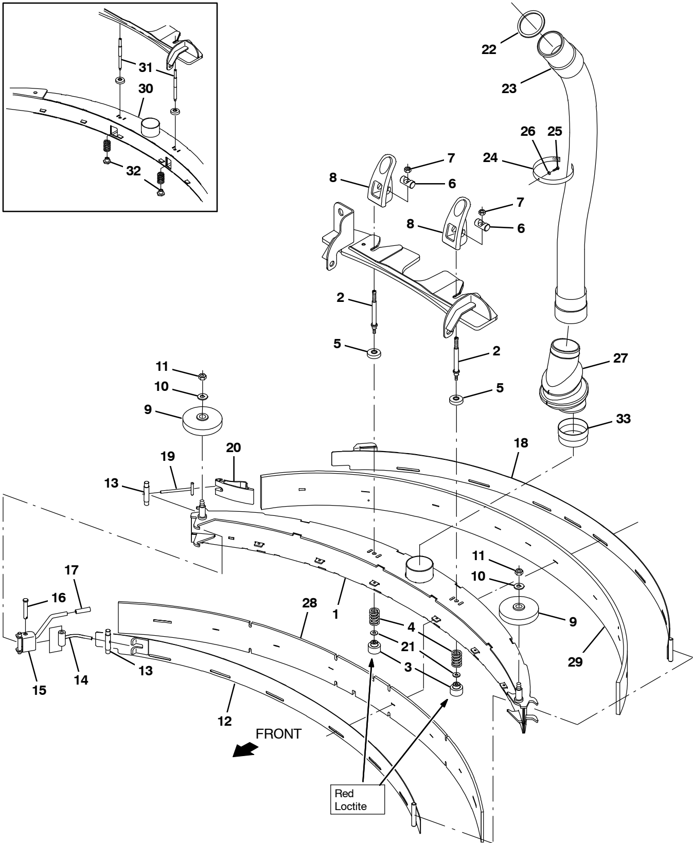
Fig. 28 – Rear Squeegee Group
