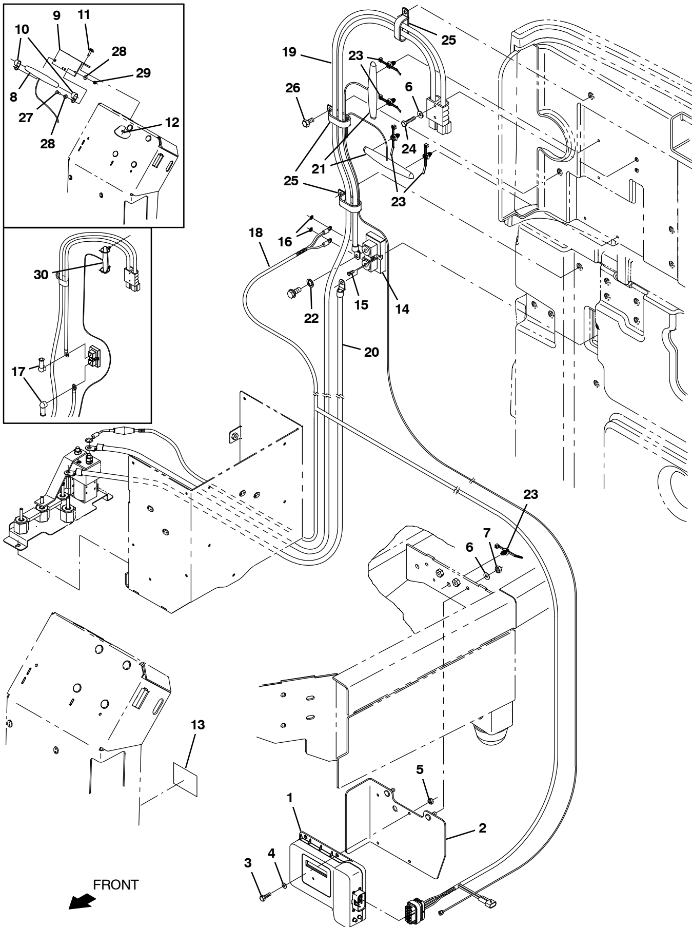
Fig. 40 – Telemetry Group
