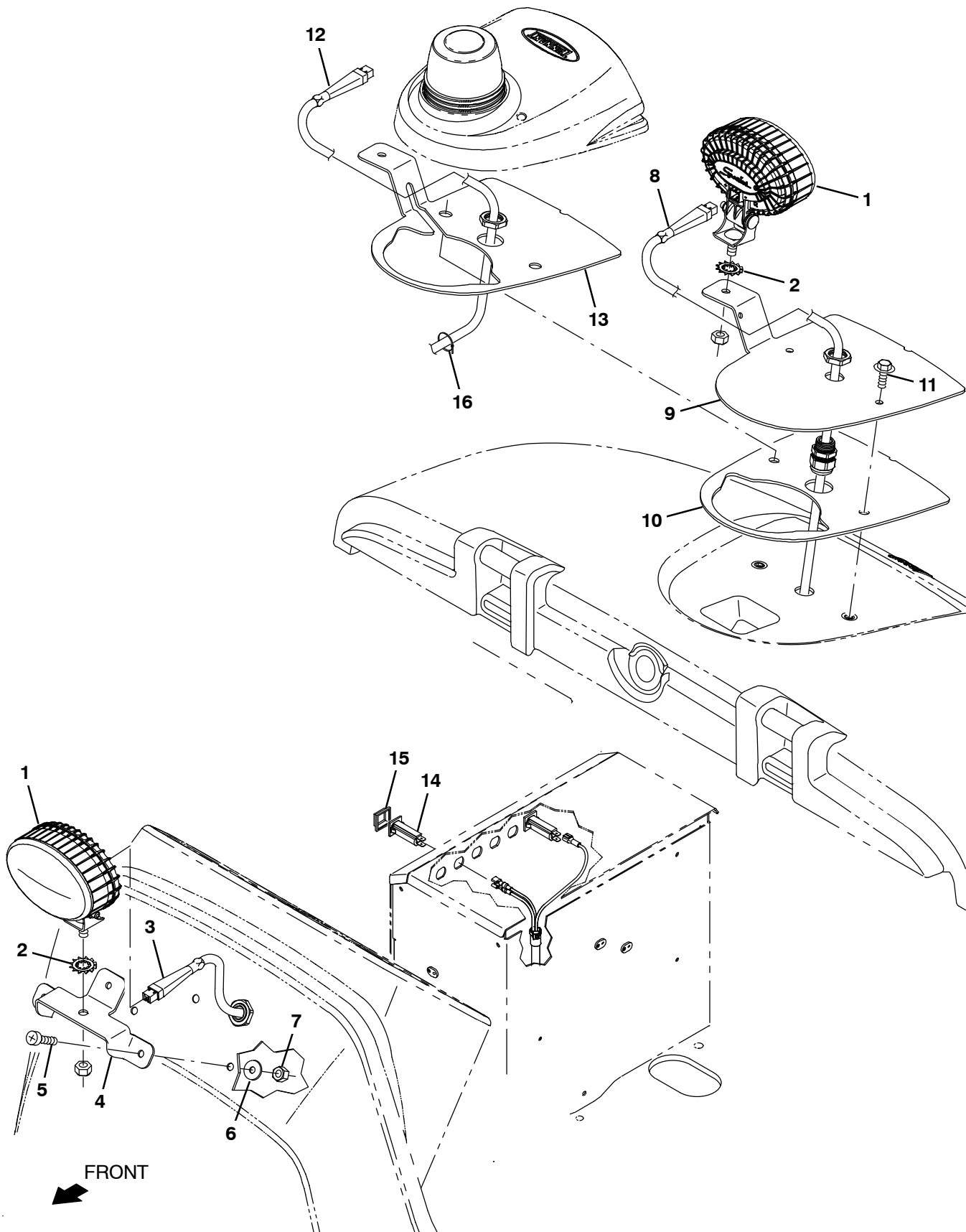
Fig. 65 – Spotlight Kit, Blue
