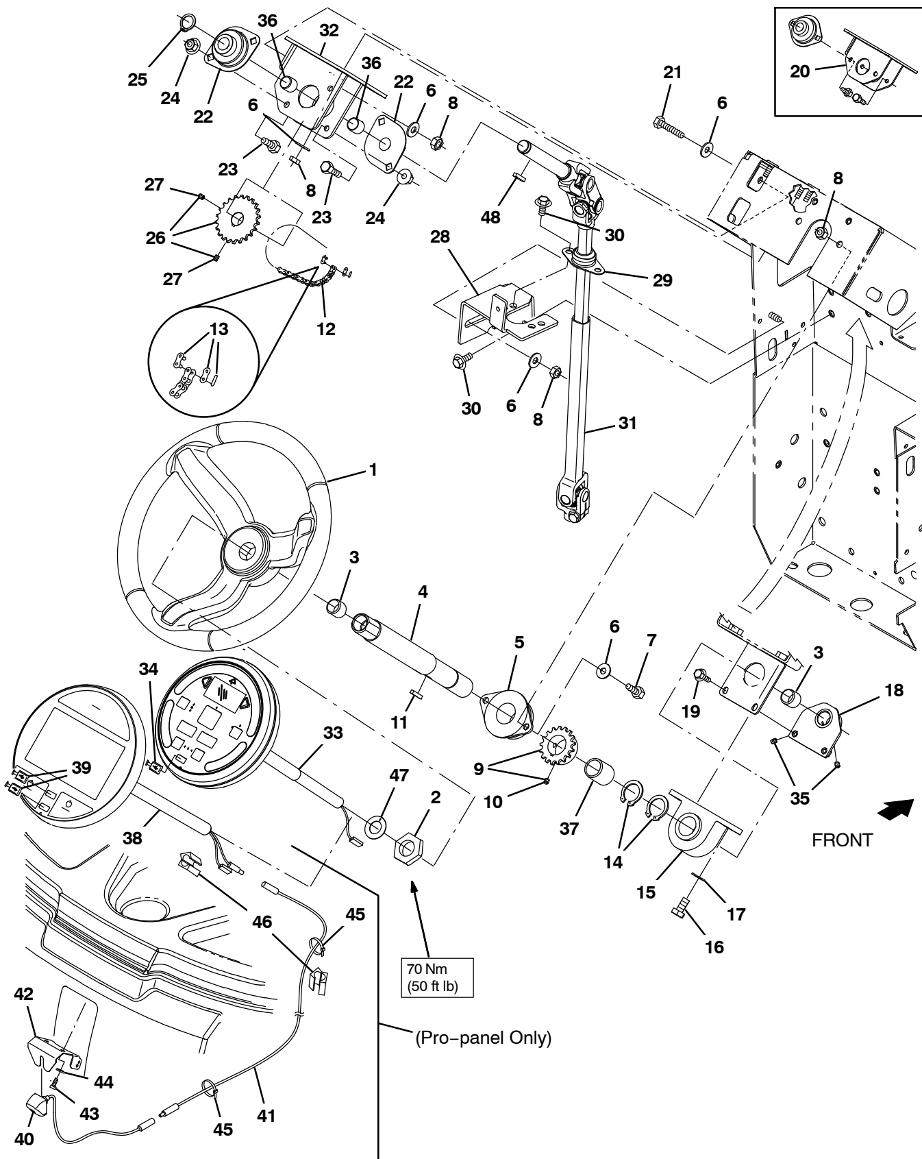
Fig. 5 – Steering Group
