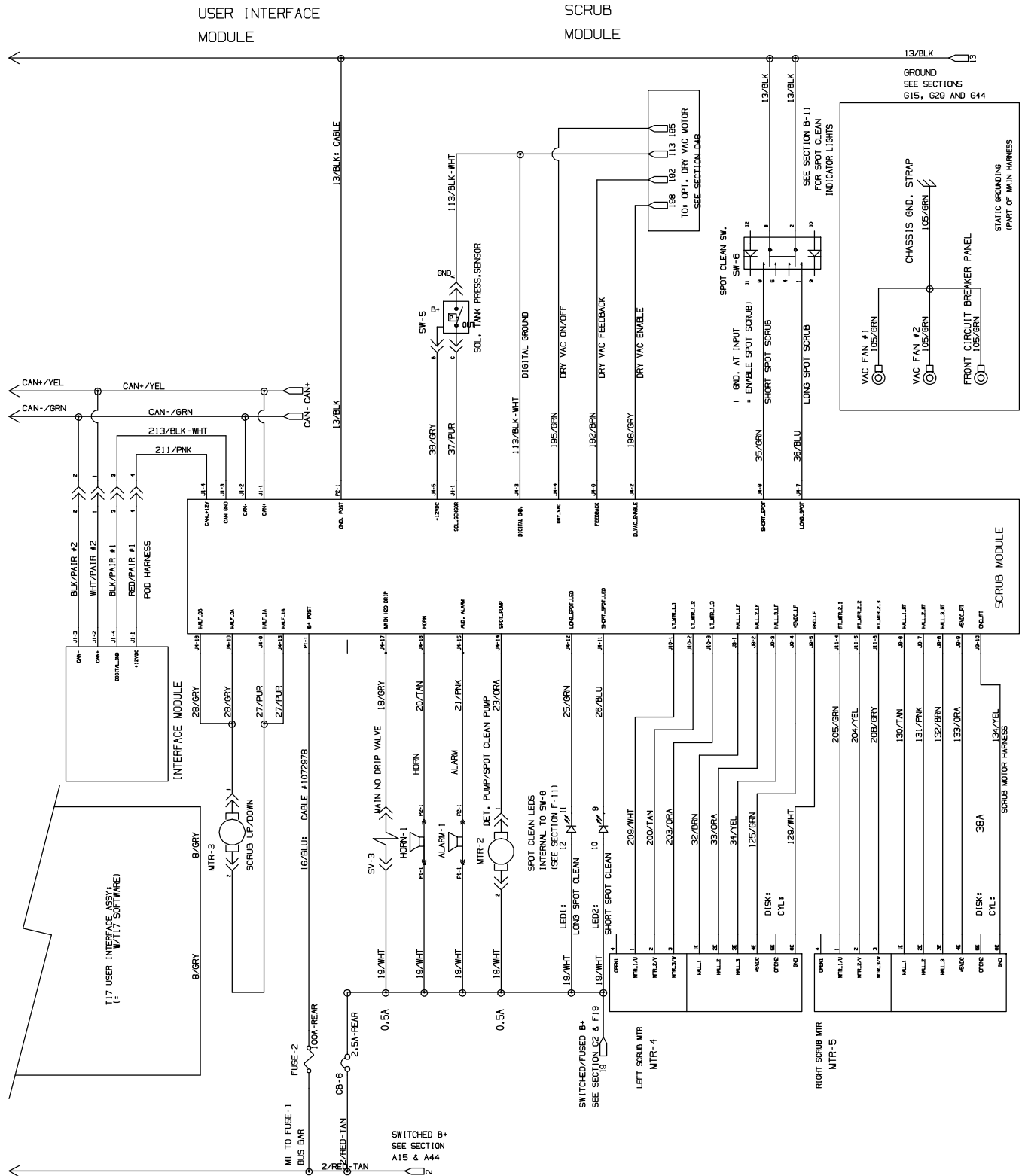
Fig. 35 – Electrical Schematic (014000- )
