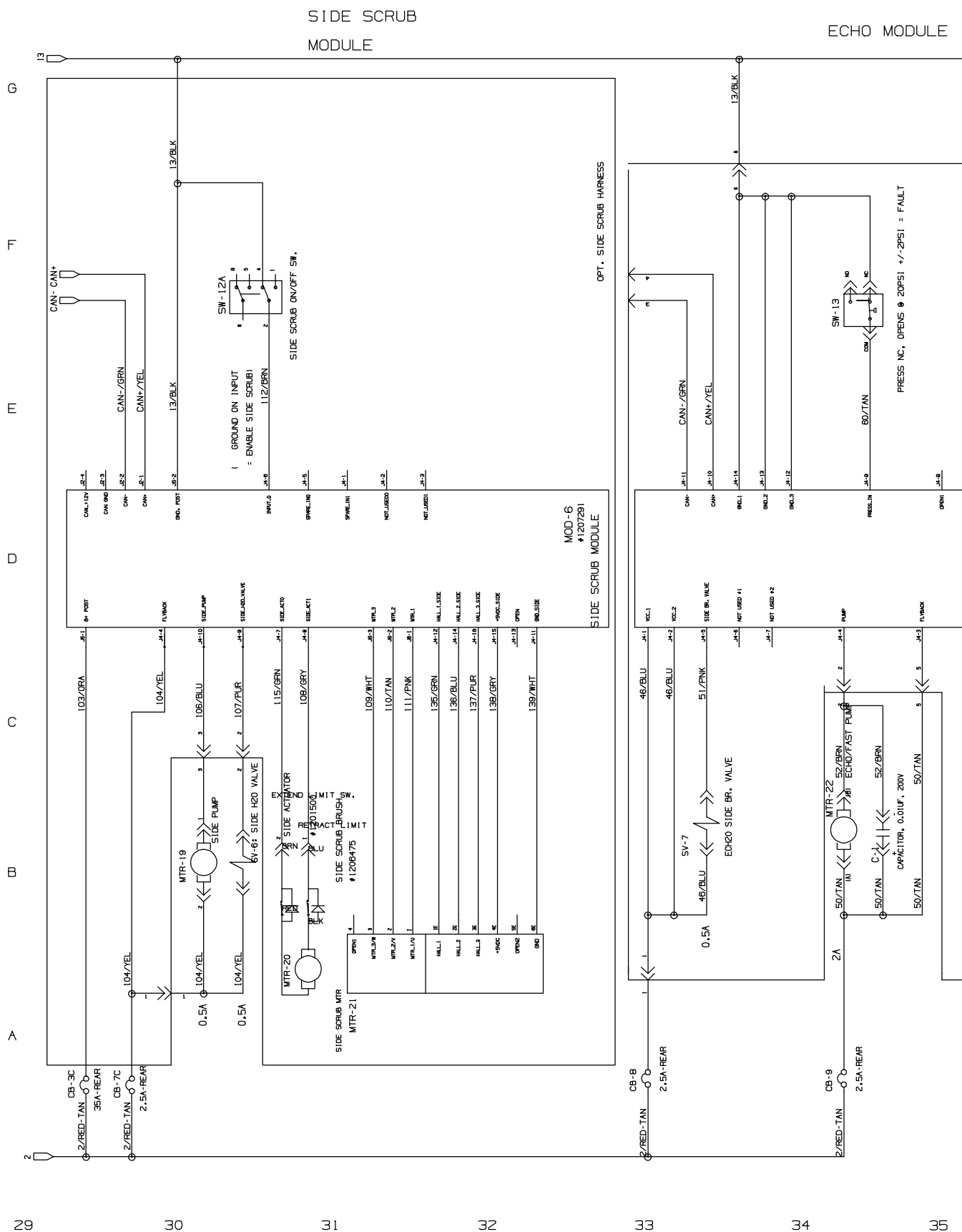
Fig. 33 – Electrical Schematic (011000-012999)
