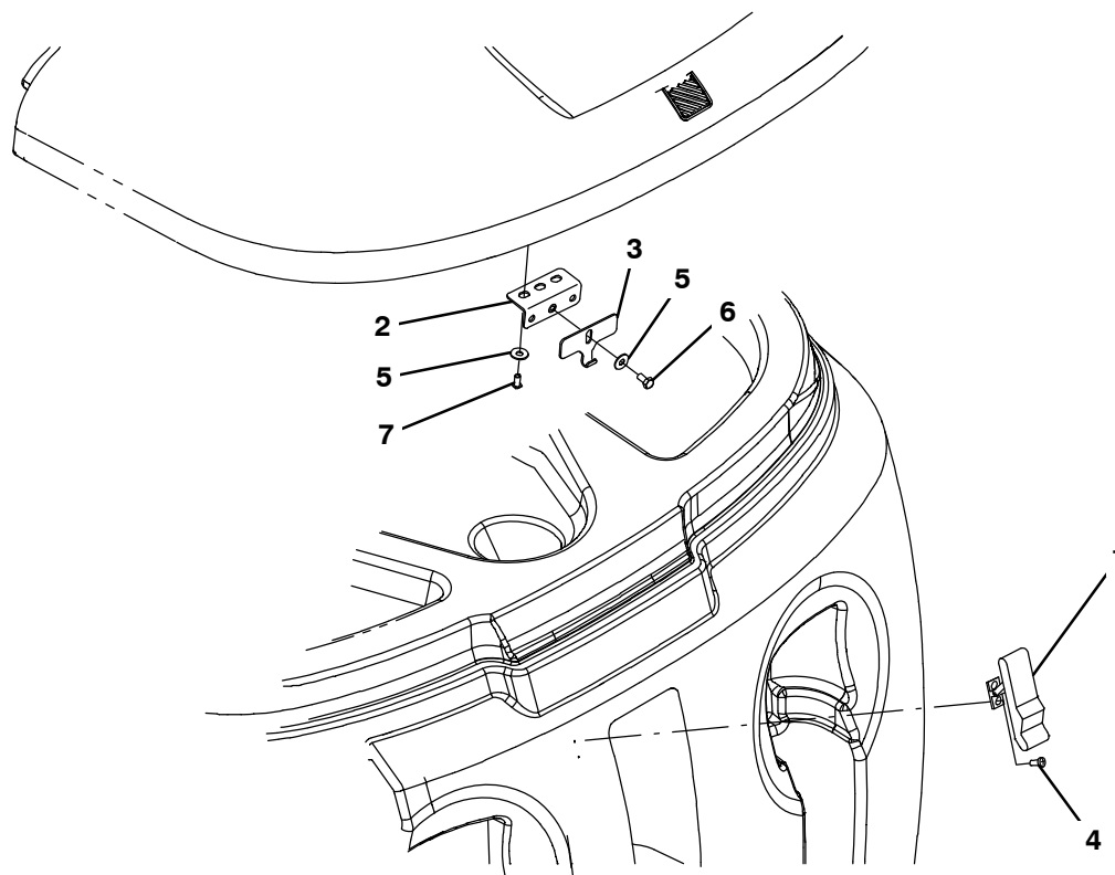
Fig. 9 – Transport Group
