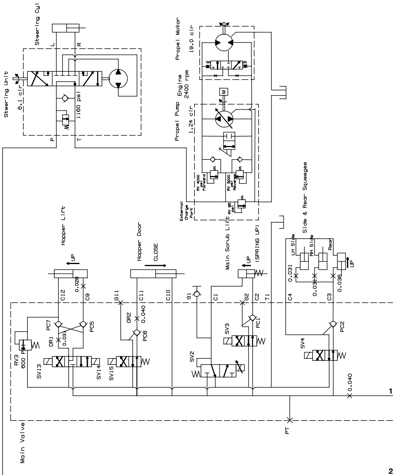
Fig. 51 - Hydraulic Schematic (001463- )
