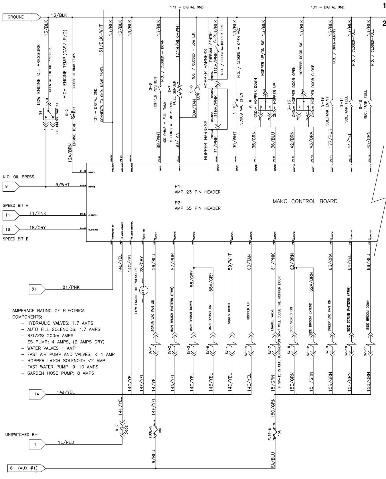
Fig. 61 - Electrical Schematic, (000000-001544)
