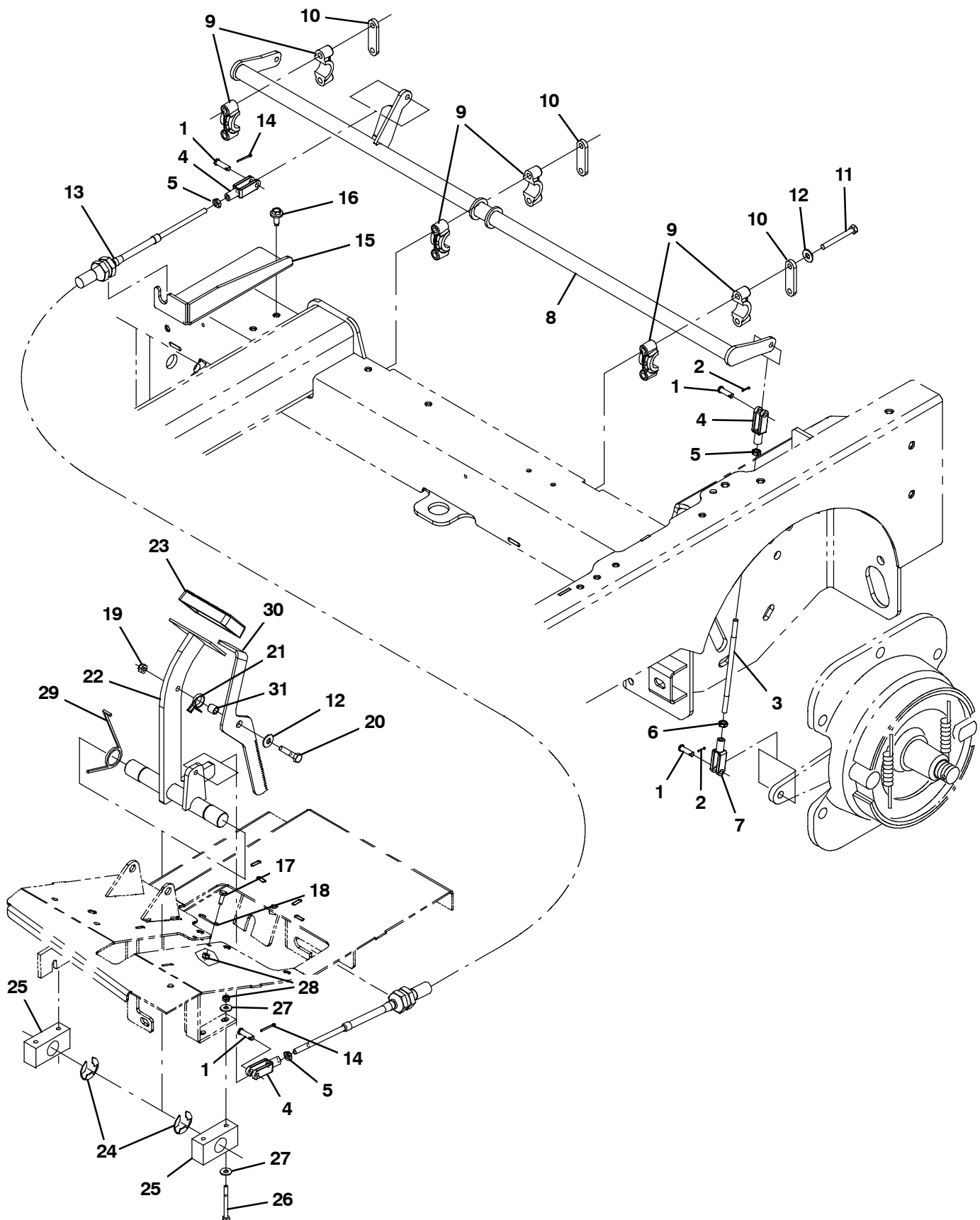
Fig. 24 - Brake Pedal Linkage Group
