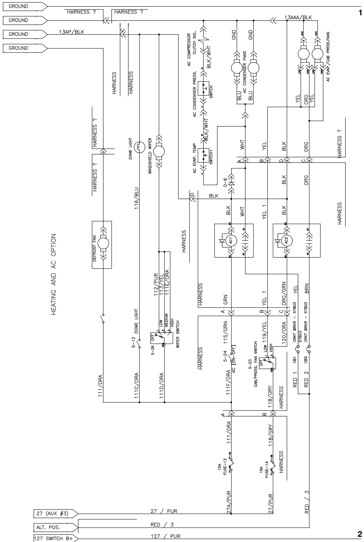
Fig. 62 - Electrical Schematic, (001545-003999)
