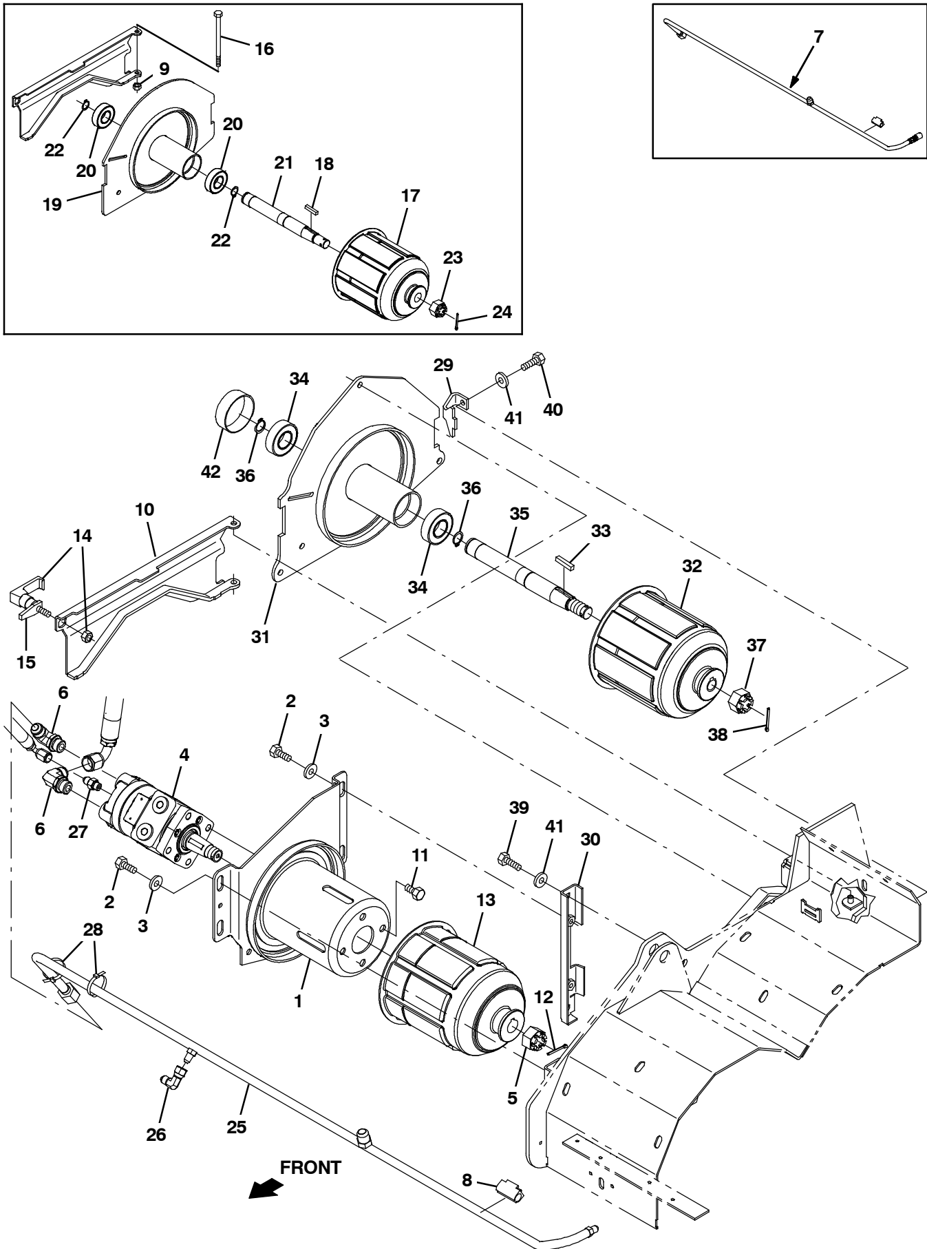
Fig. 32 - Brush Drive Group, Right Side
