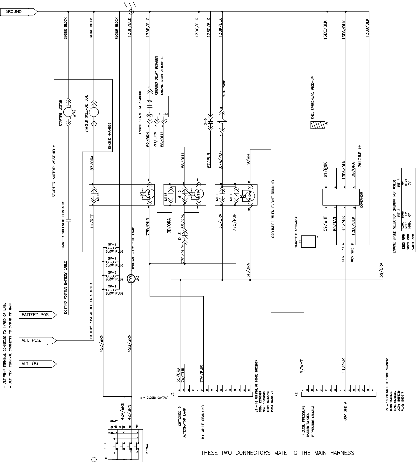
Fig. 64 - Electrical Schematic, Diesel Engine Harness
