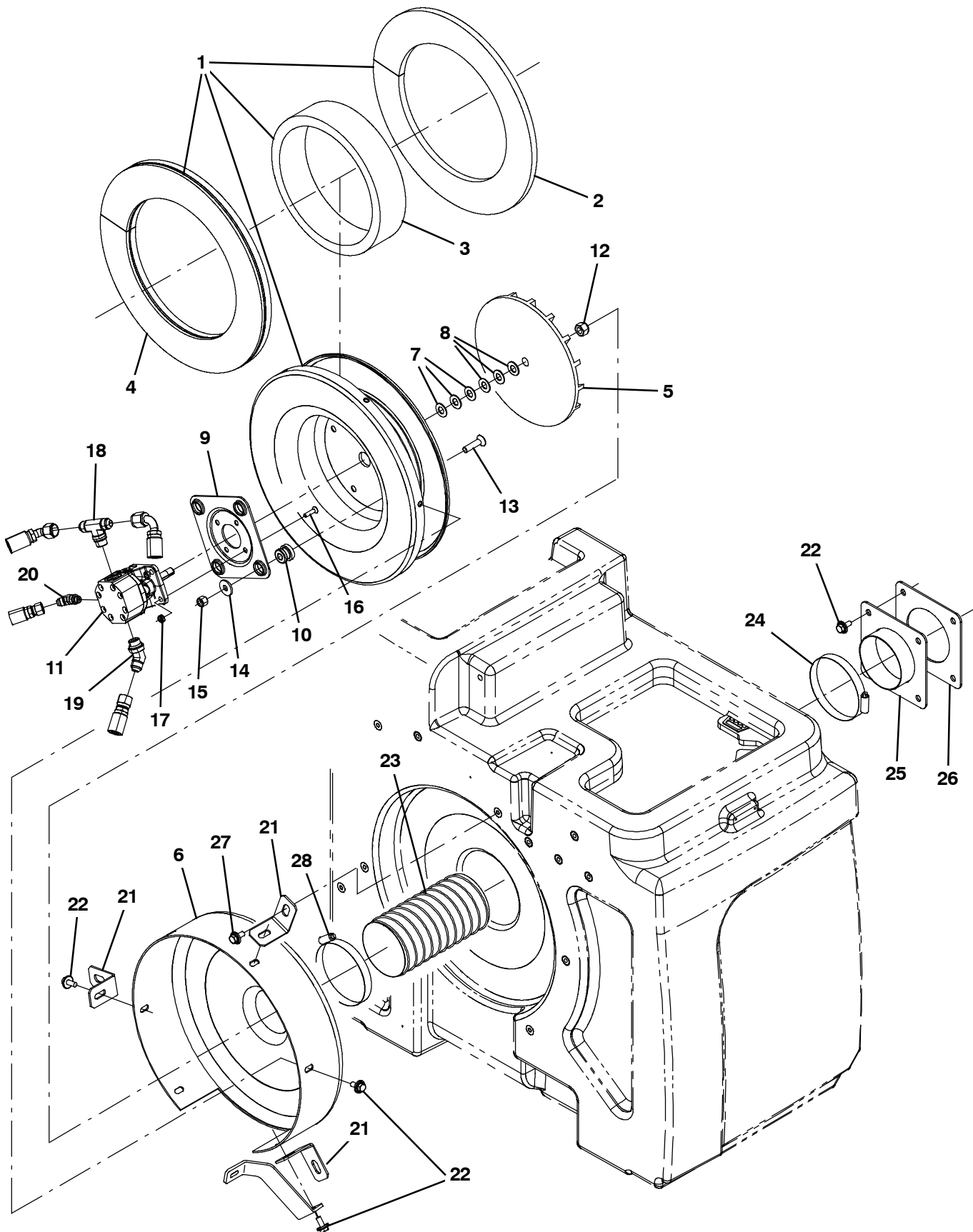
Fig. 47 - Vacuum Fan Group, Scrubbing (000000-004454)
