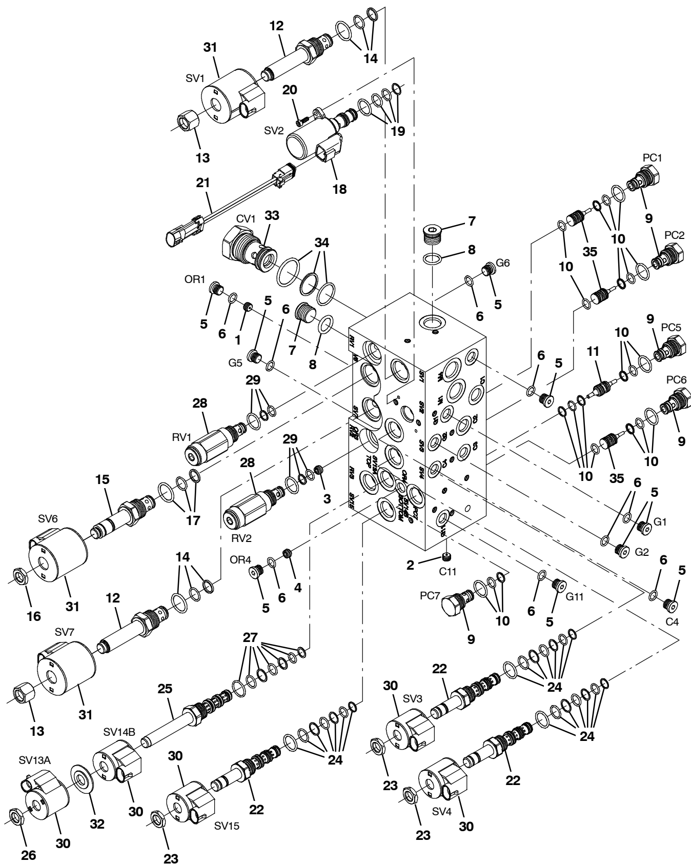
Fig. 9 - Hydraulic Valve Breakdown, 1072995
