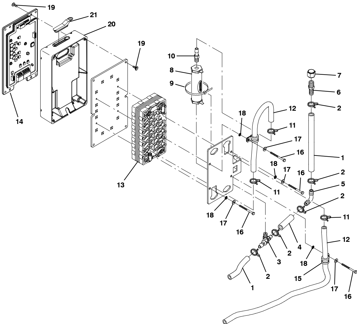
Fig. 16 - ec-H20 Module Assembly Breakdown, 9007882
