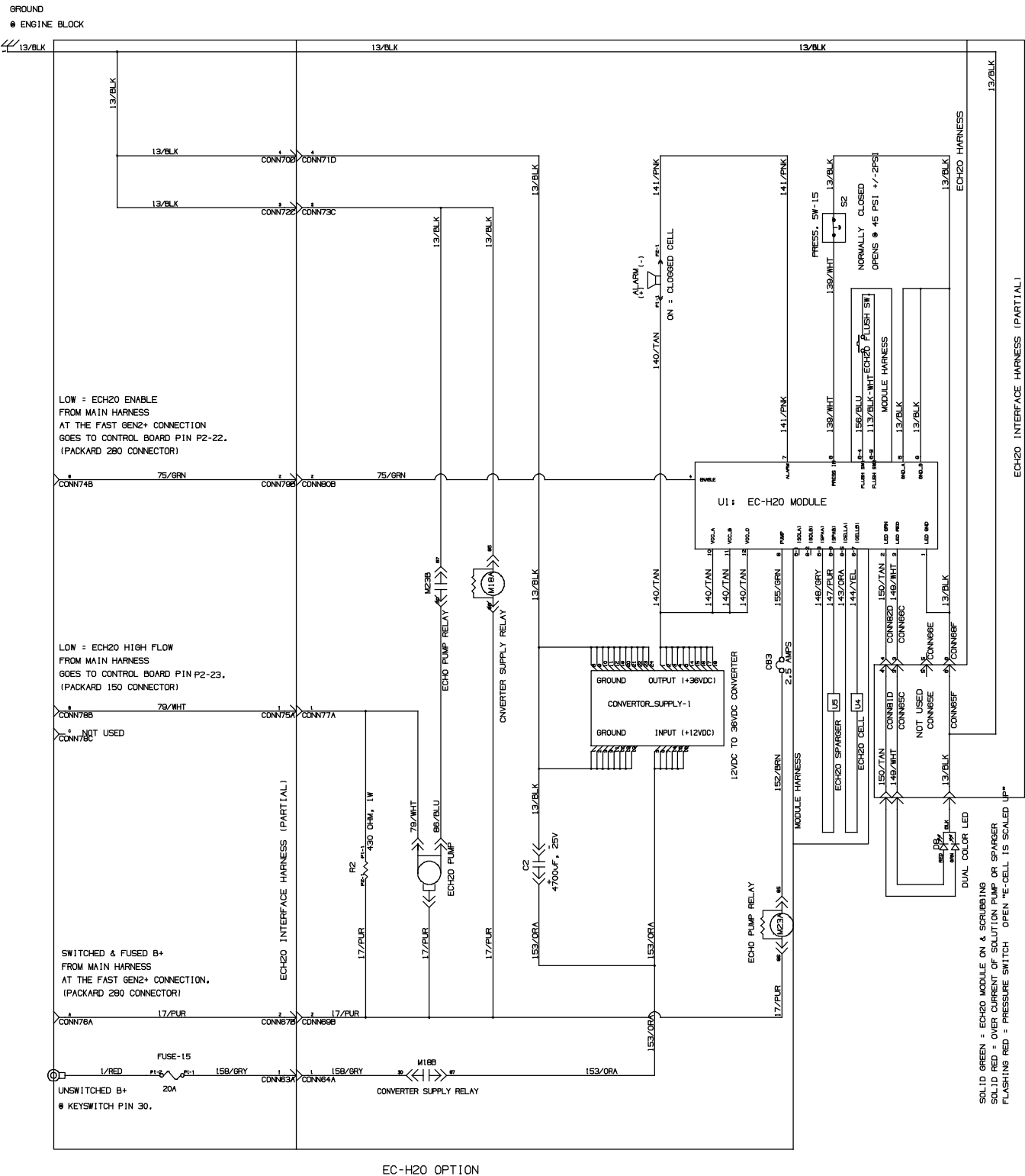
Fig. 62 - Electrical Schematic, (001545-003999)
