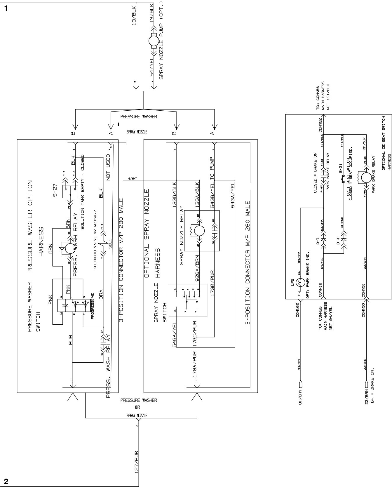
Fig. 63 - Electrical Schematic, (004000- )
