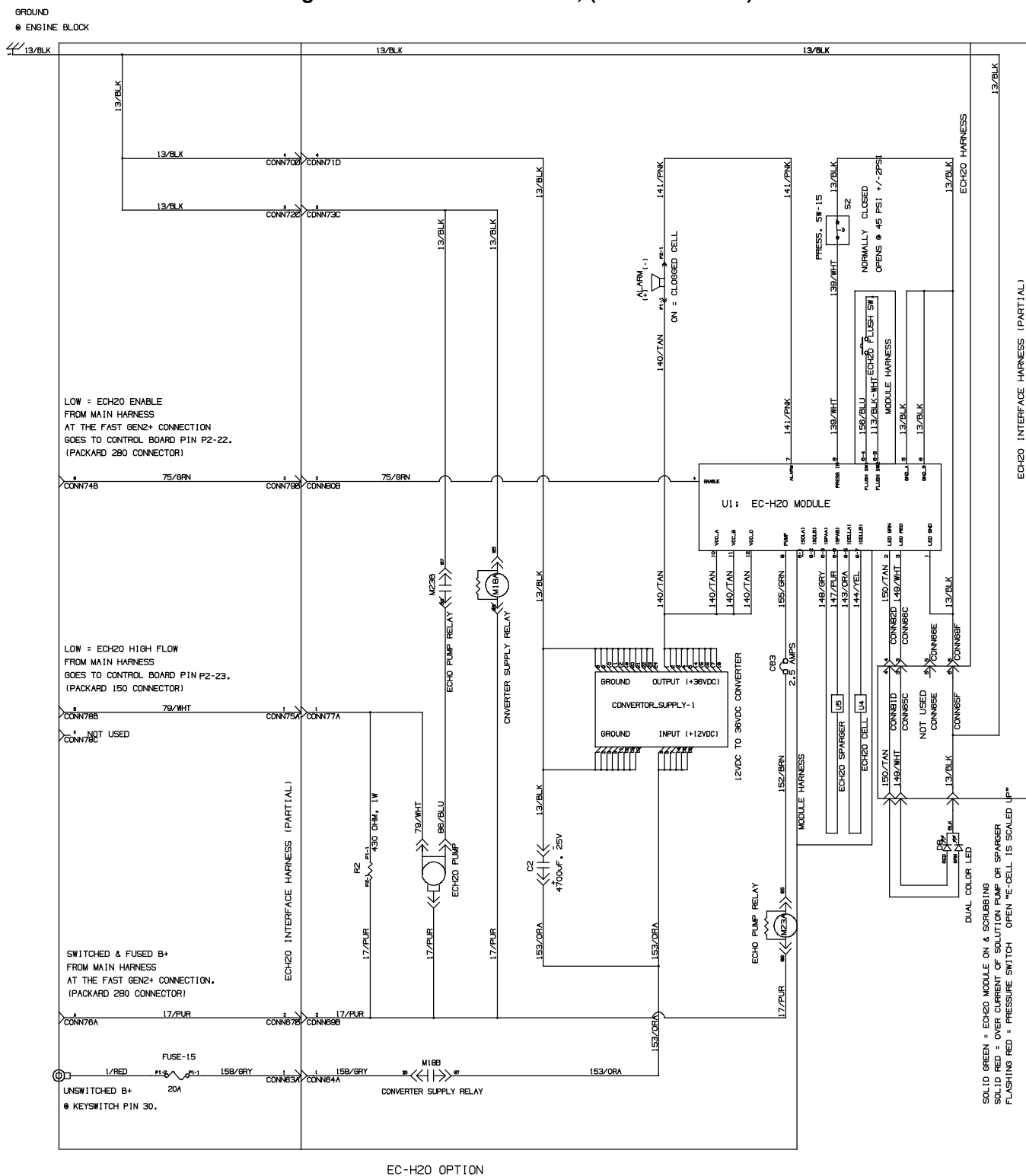
Fig. 61 - Electrical Schematic, (000000-001544)
