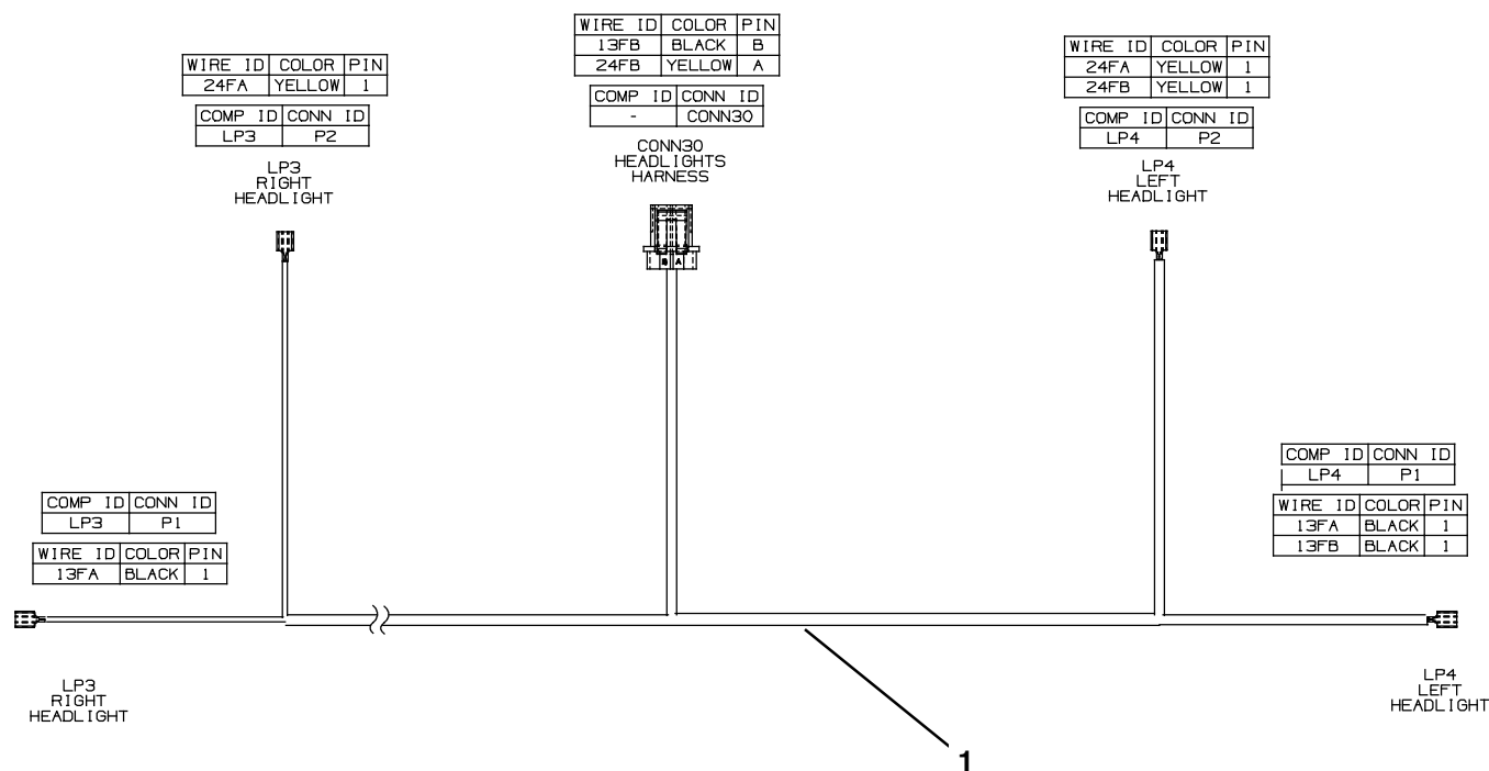
Fig. 66 - Electrical Wire Harness Group, Headlight
