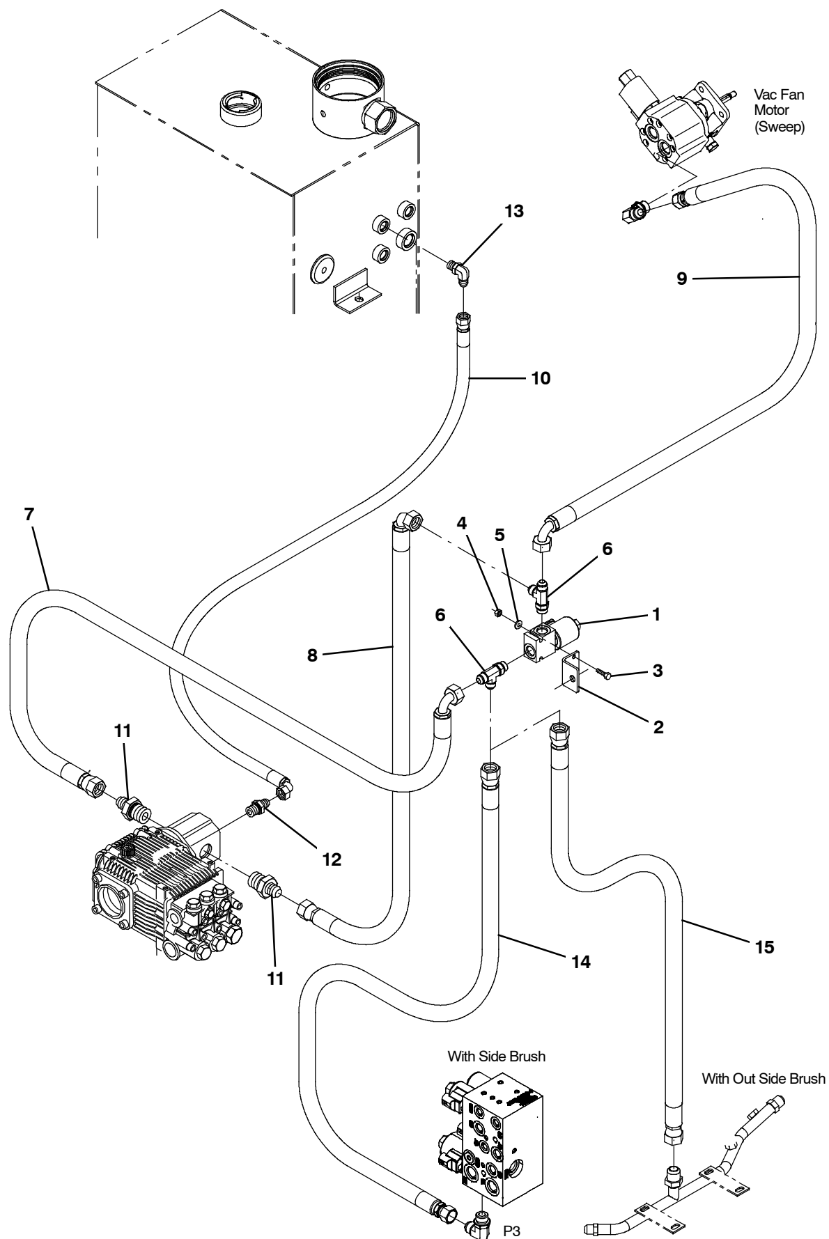
Fig. 29 - Pressure Washer Hydraulic Hoses Group (000000-003999)
