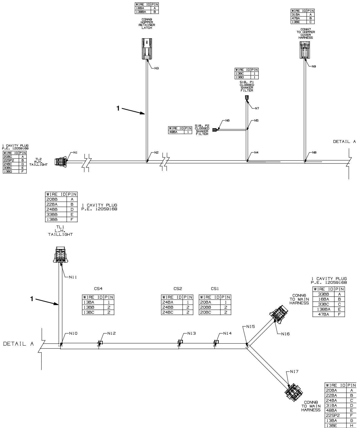
Fig. 67 - Electrical Wire Harness Group, Hopper
