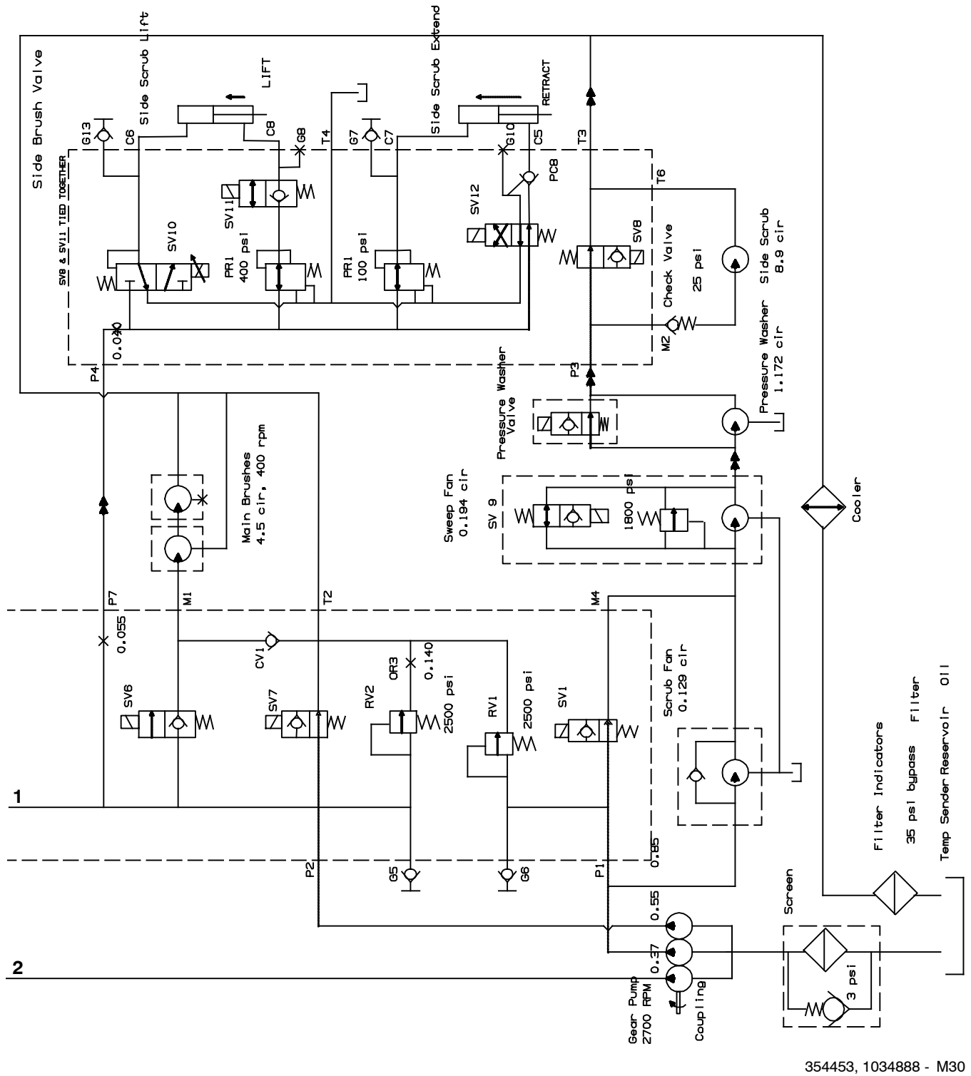
Fig. 50 - Hydraulic Schematic (000000-001462)
