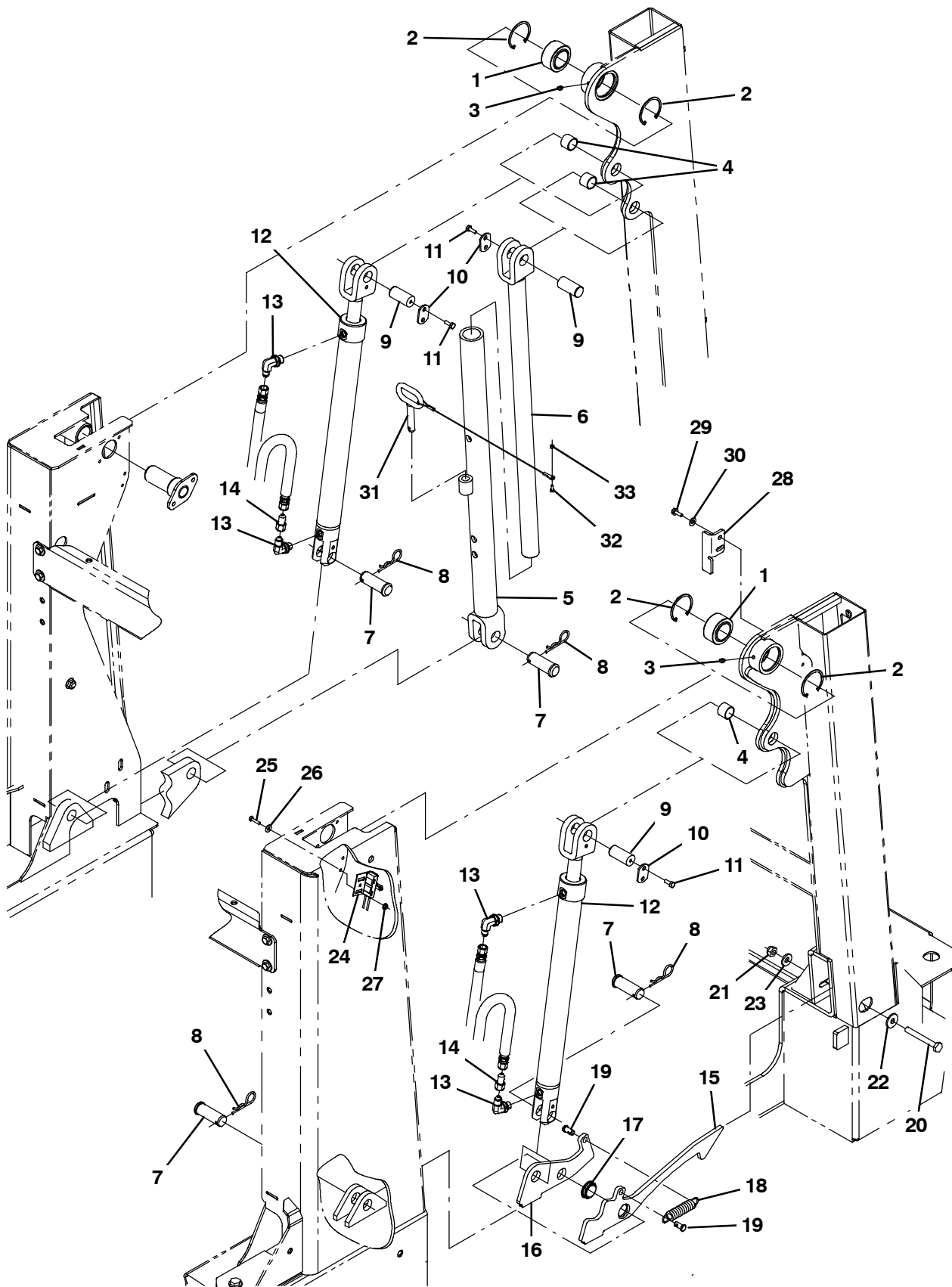
Fig. 26 - Hopper Lift Arms Group
