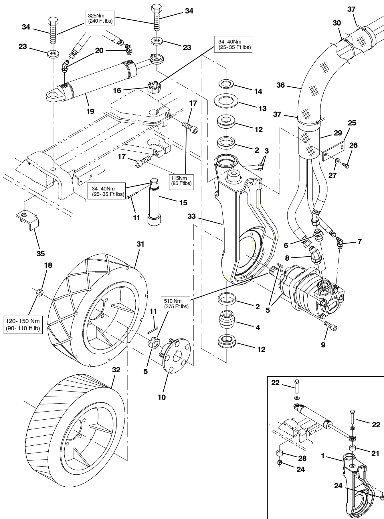
Fig. 22 - Wheel Group, Front Drive
