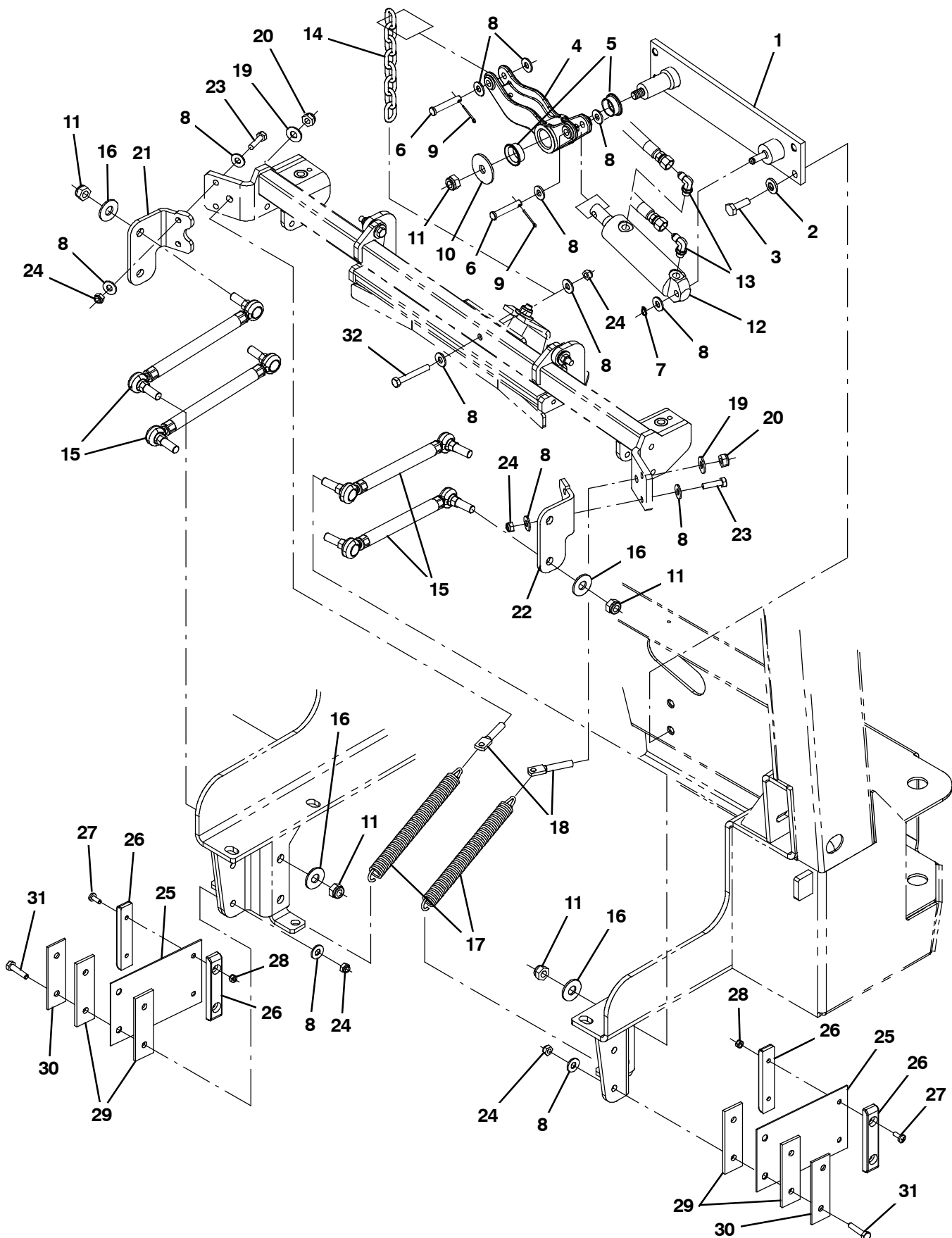
Fig. 35 - Squeegee Lift Group, Rear
