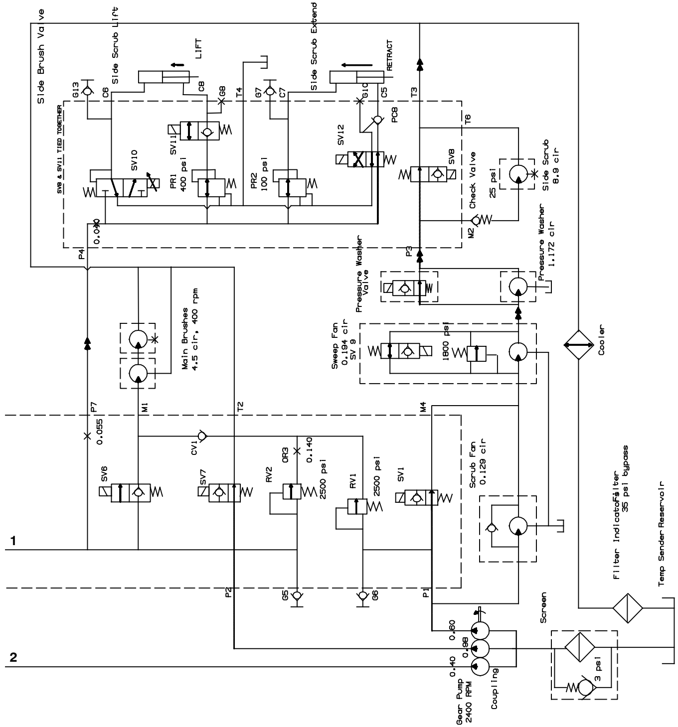
Fig. 51 - Hydraulic Schematic (001463- )
