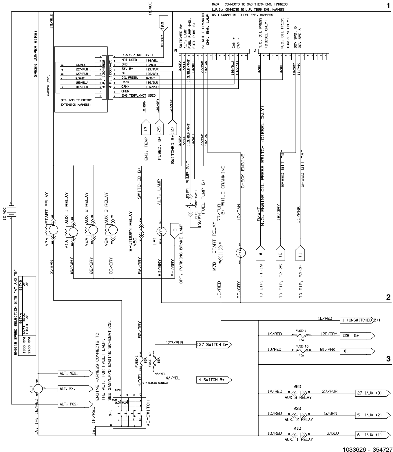
Fig. 63 - Electrical Schematic, (004000- )
