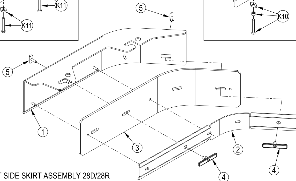
LEFT SIDE SKIRT ASSEMBLY 28D/28R
