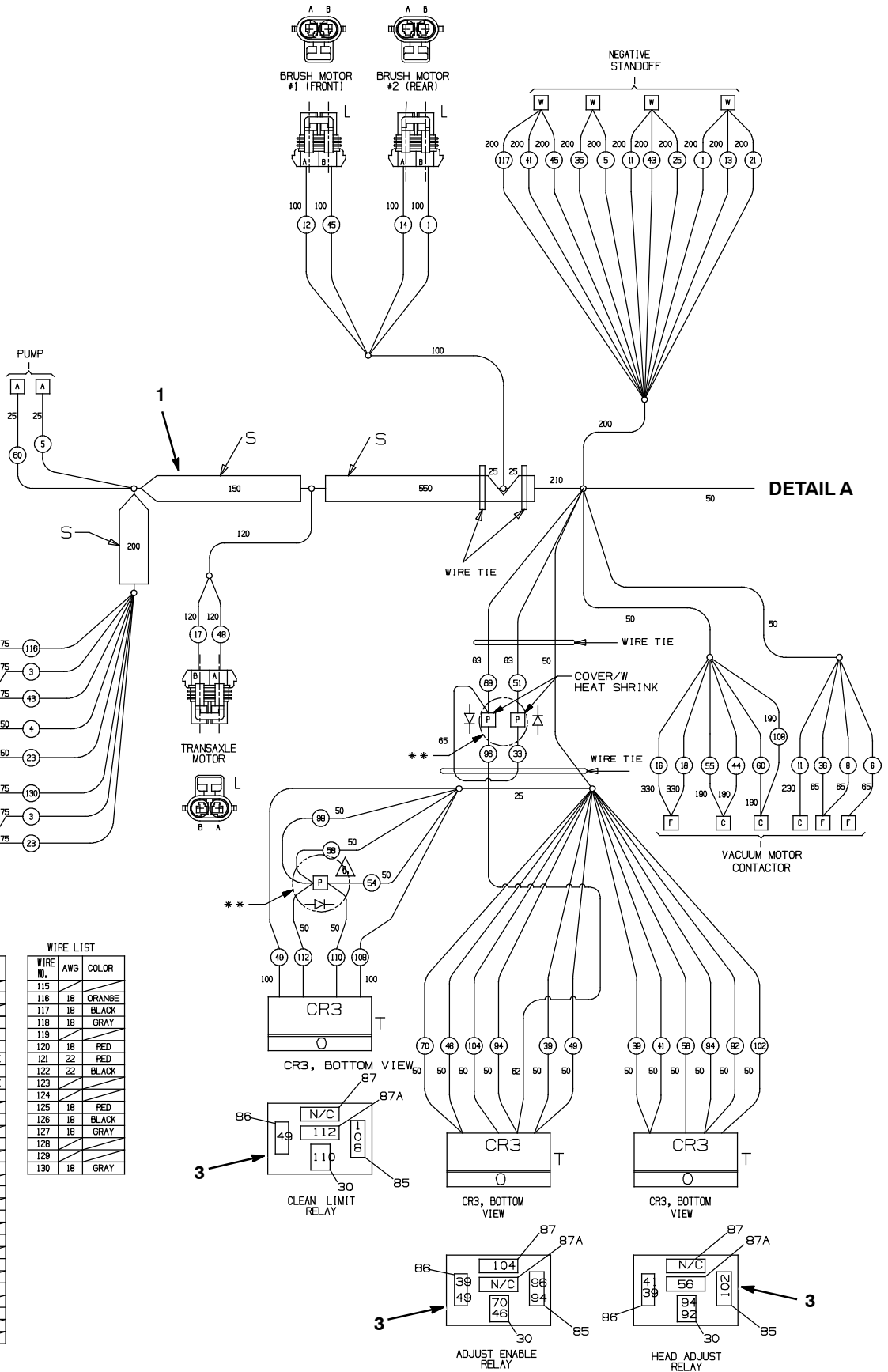
WIRE LIST
