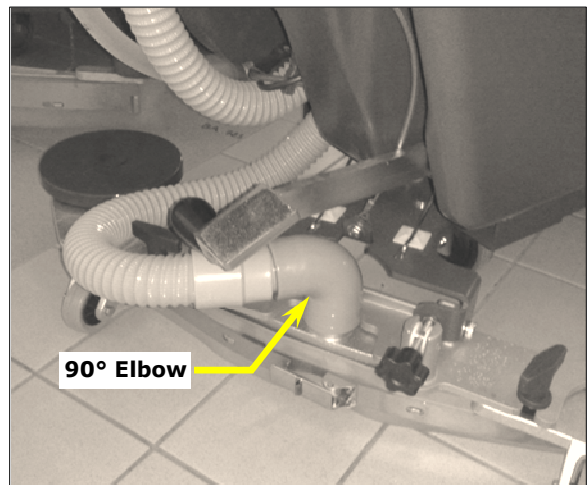
Figure 2 – Squeegee Vacuum Hose Connected to Squeegee with 90° Elbow
