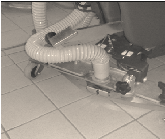
Figure 1 – Squeegee Vacuum Hose Connected Directly into Squeegee
