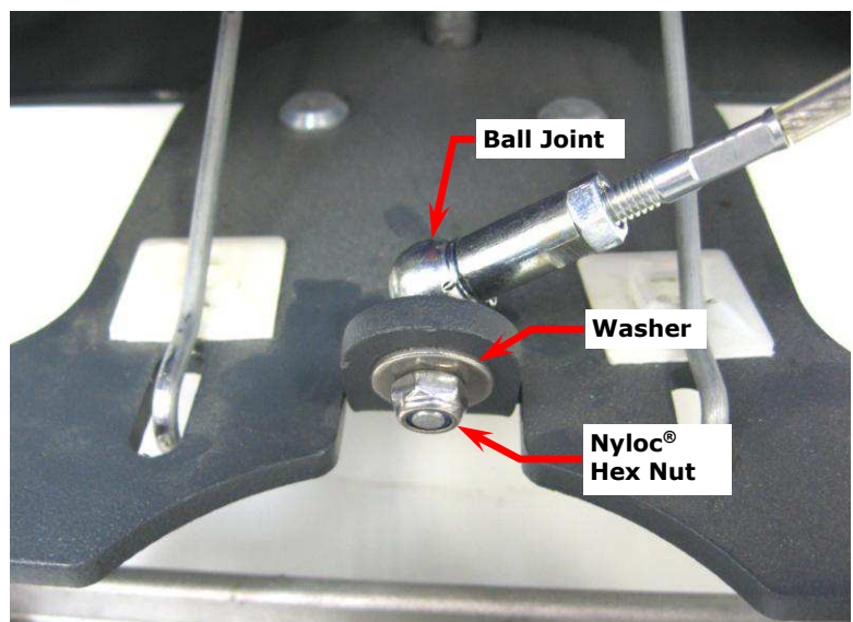
Figure 5 – Attaching New Squeegee Cable to the Squeegee Support
