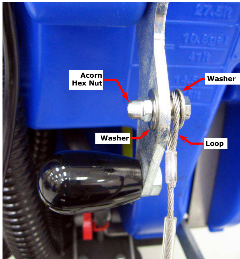
Figure 6 – Attaching New Squeegee Cable to the Squeegee Lifting Lever
