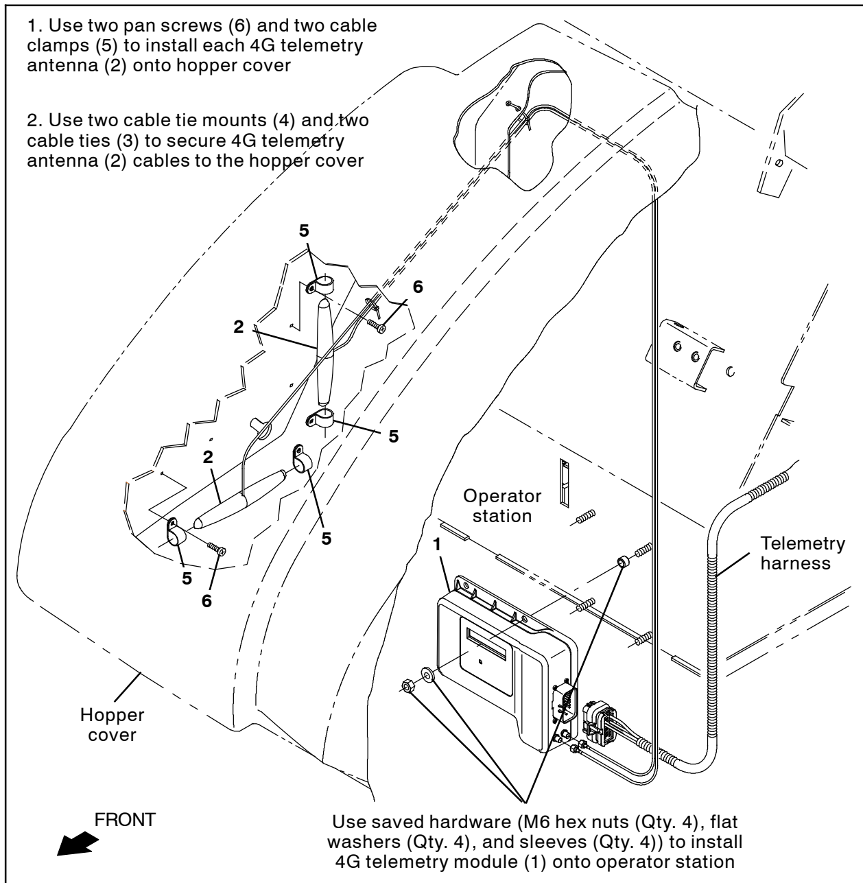
FIG. 10 - S20 Sweeper
