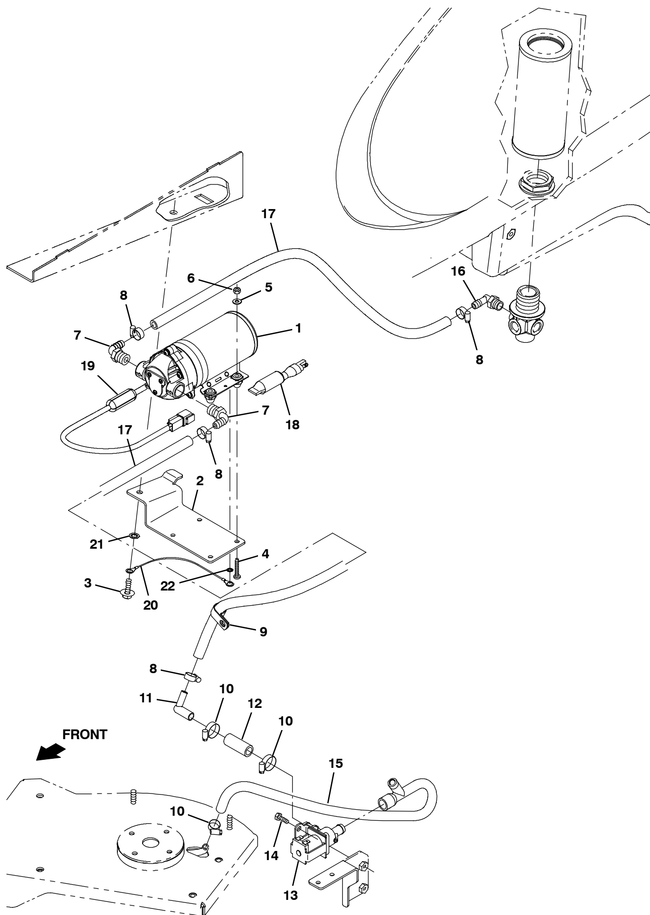
Fig. 31 - Side Brush Solution Supply Group
