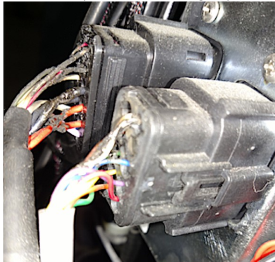
Example of a Bad Steering amp (Damaged wiring)
