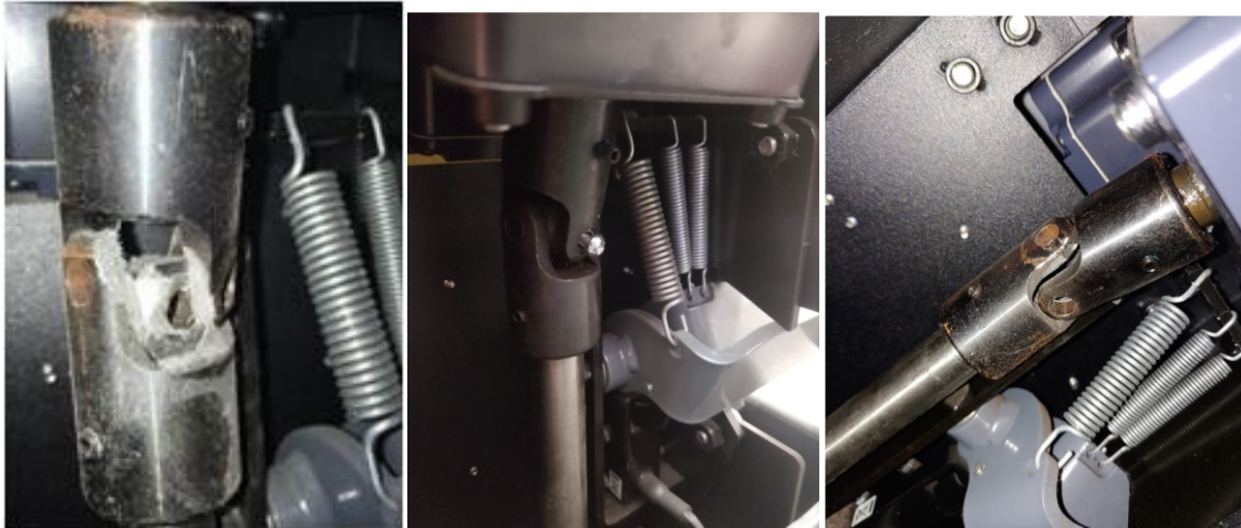
Example of a broken U-joint
