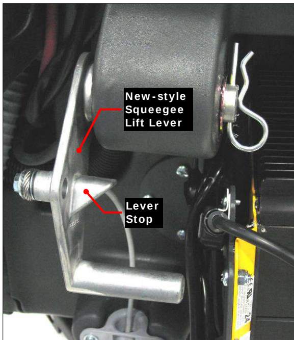
Figure 1 – New-style Solution Tank and Squeegee Lift Lever
