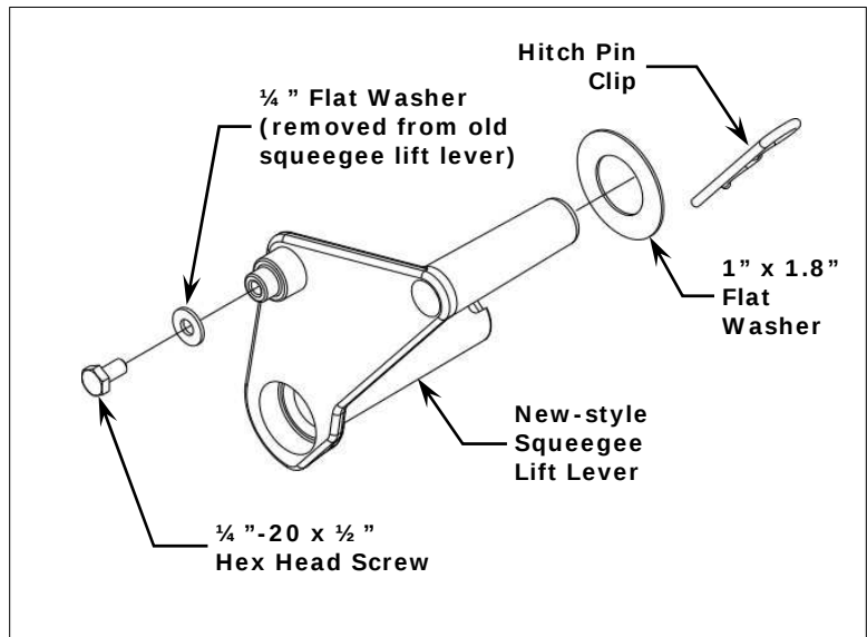
Figure 3 – New-style Squeegee Lift Lever and Mounting Hardware
