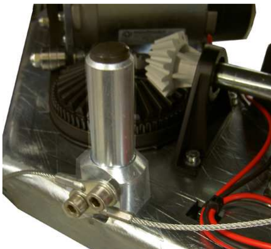
Guidance bolt fixed to motor base plate
