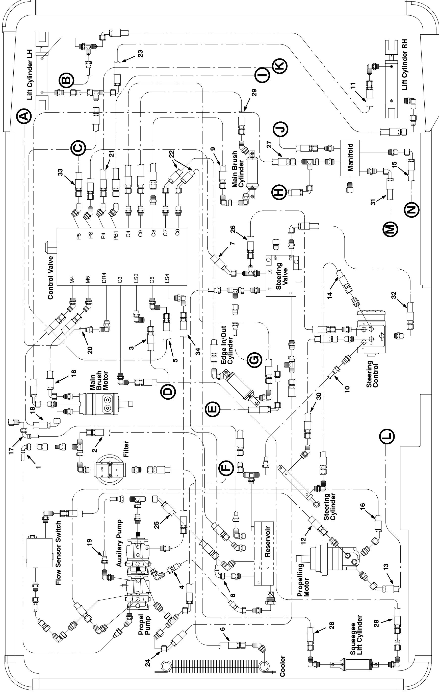
Fig. 36 – Hydraulic Hose Group
