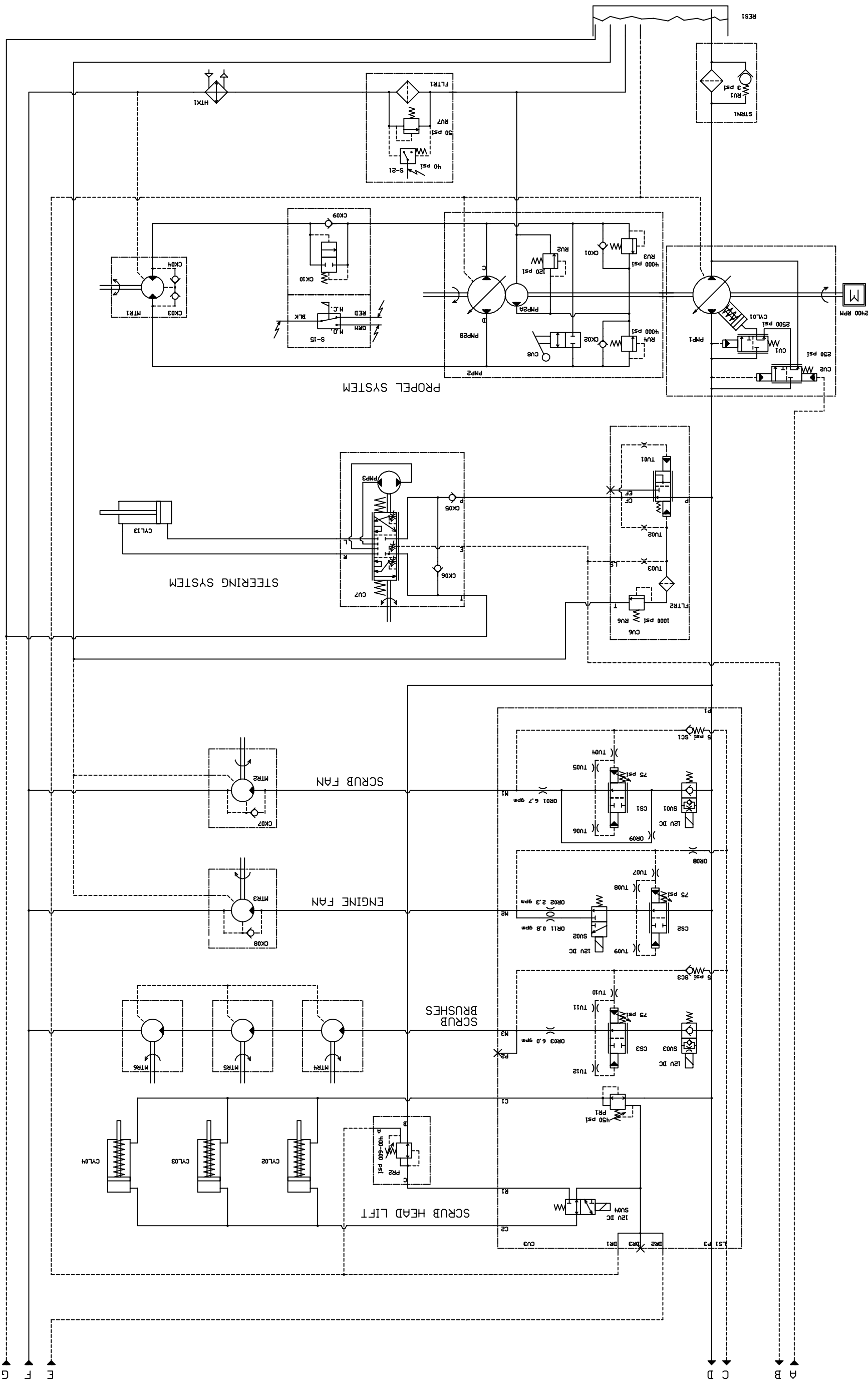
Fig. 35 - Hydraulic Schematic
