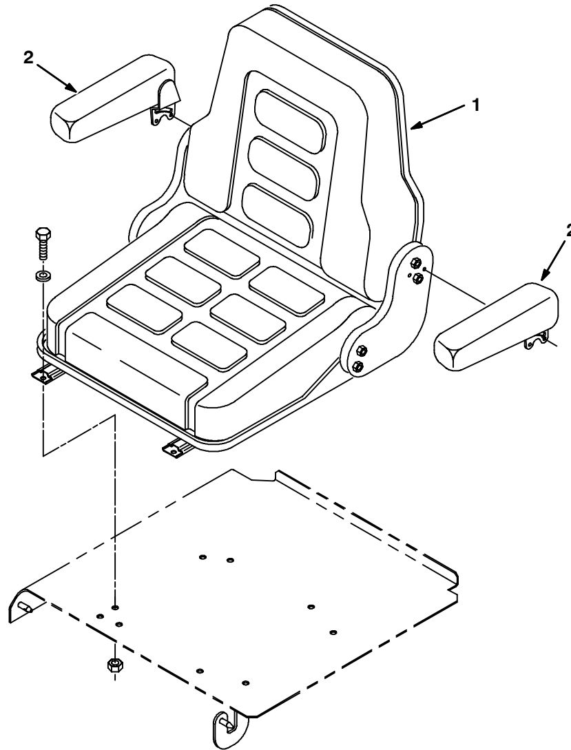
Fig. 13 - Seat Kit
