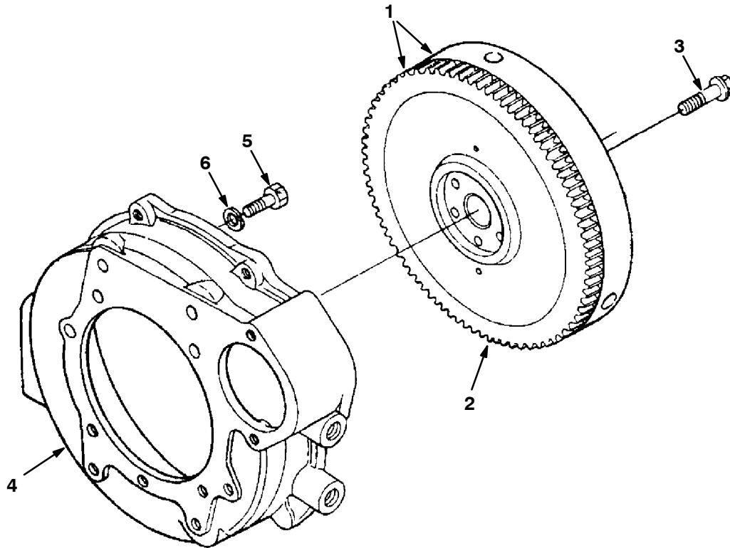
Fig. 11 - Flywheel
