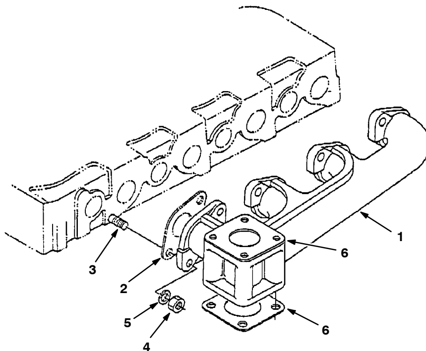
Fig. 26 - Exhaust Manifold
