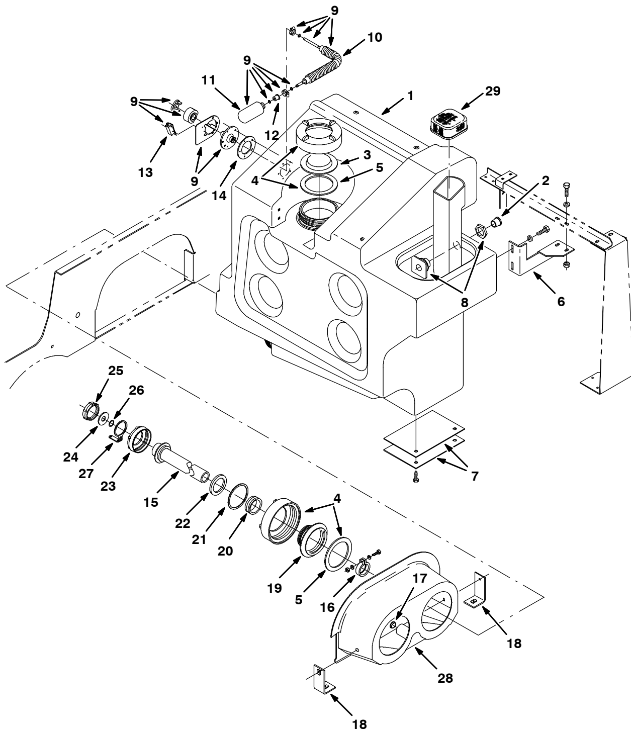
Fig. 55 - Recovery Tank Group
