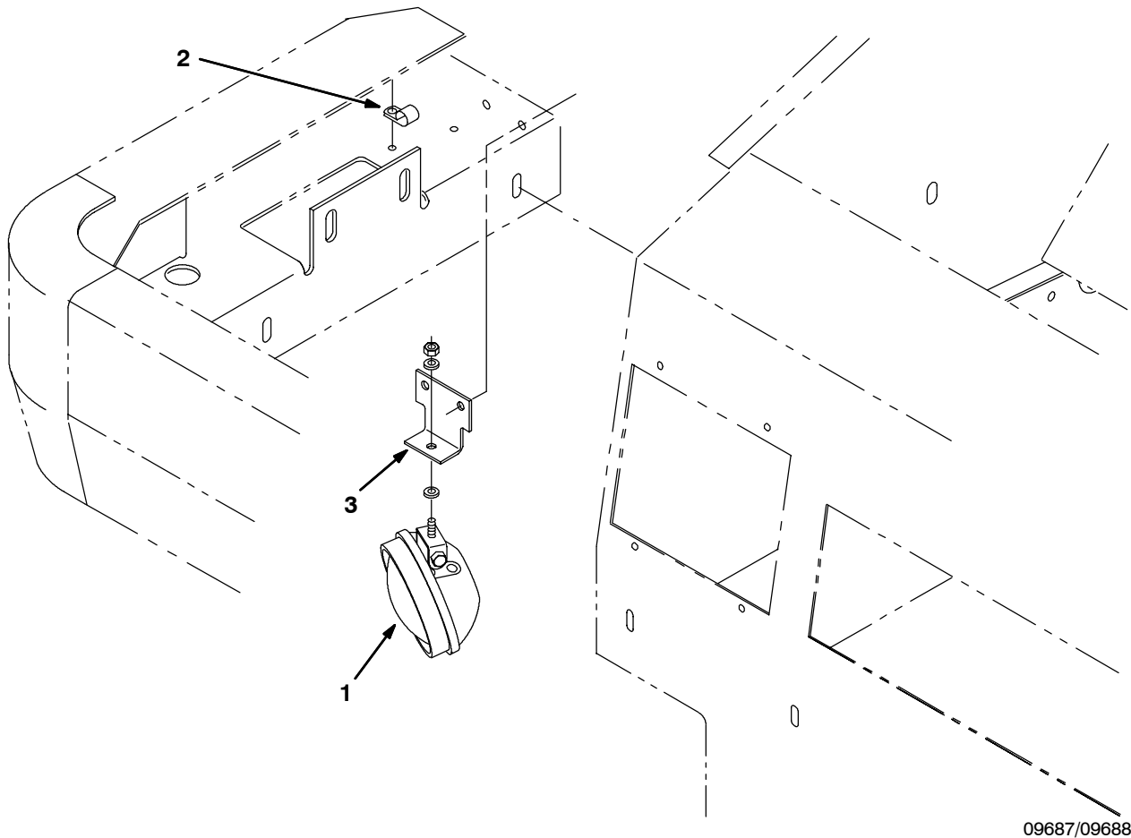
Fig. 9 - Side Brush Light Kit
