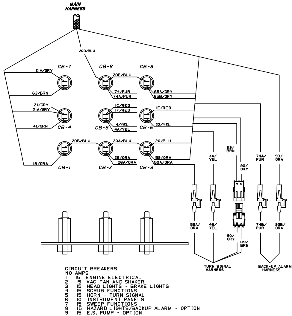
Fig. 62 - Wire Harnesses Group
