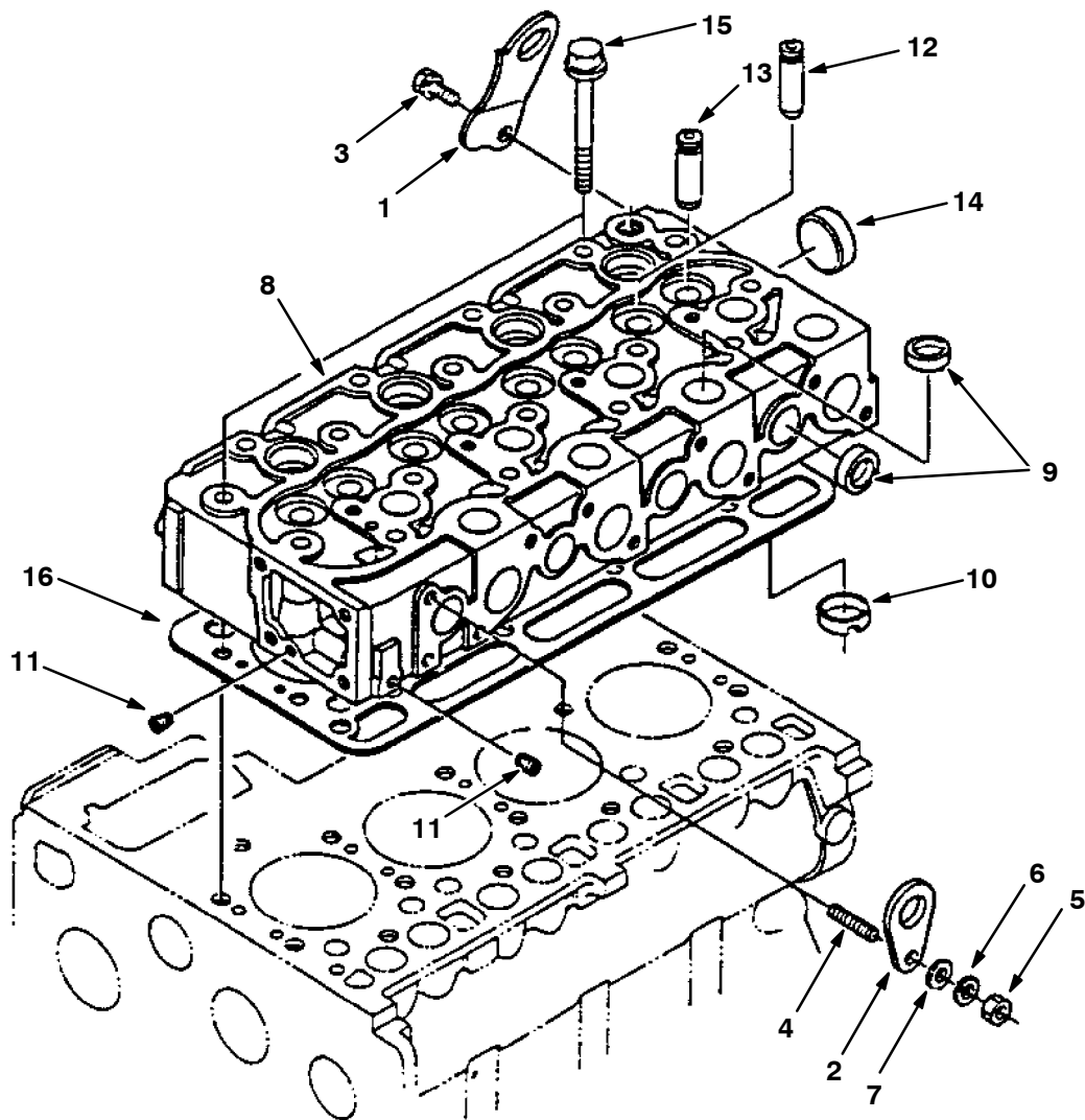
Fig. 3 - Cylinder Head
