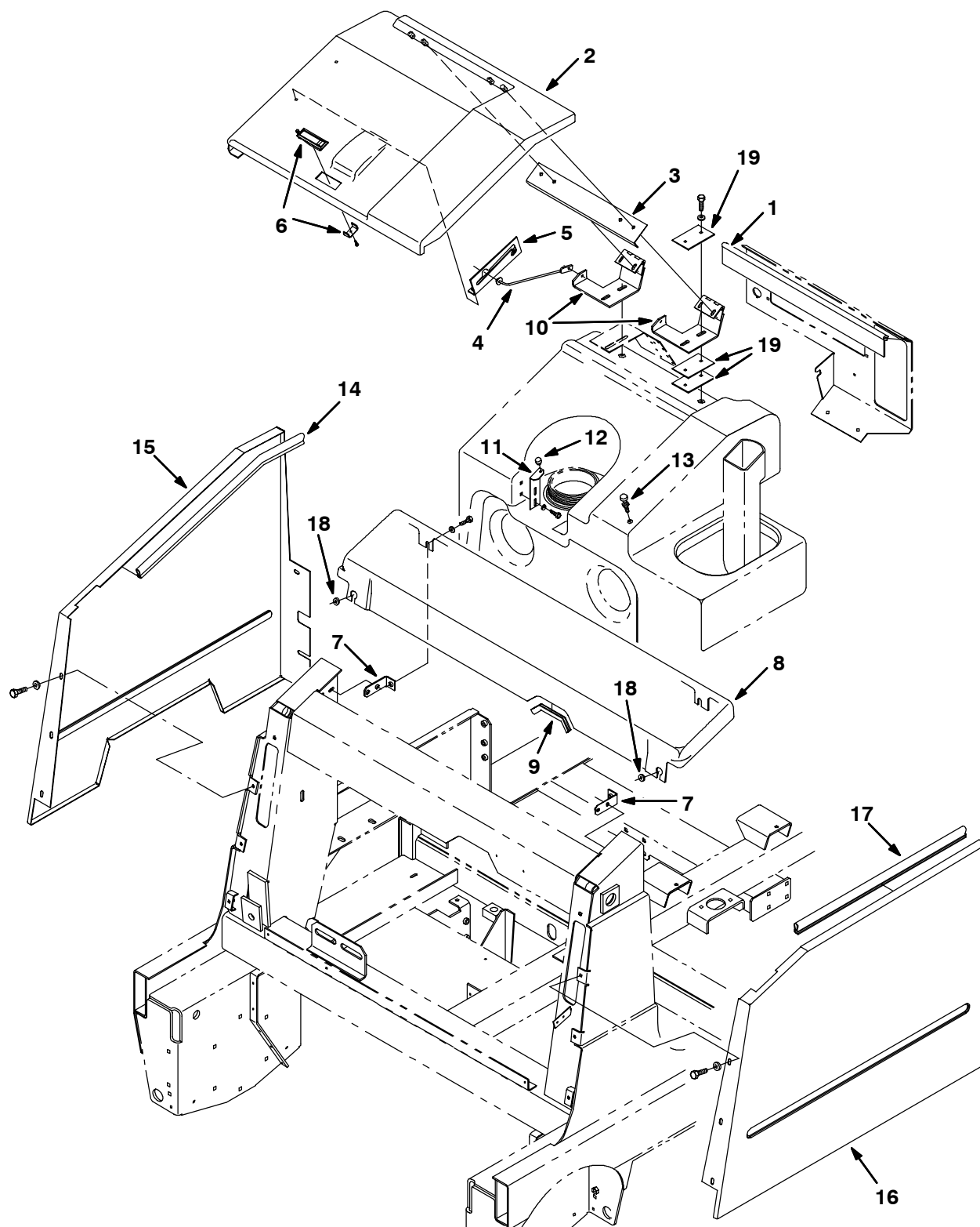
Fig. 10 - Tank Cover and Panel Group
