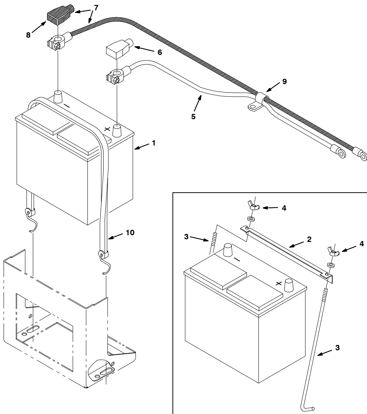
Fig. 28 - Battery Group
