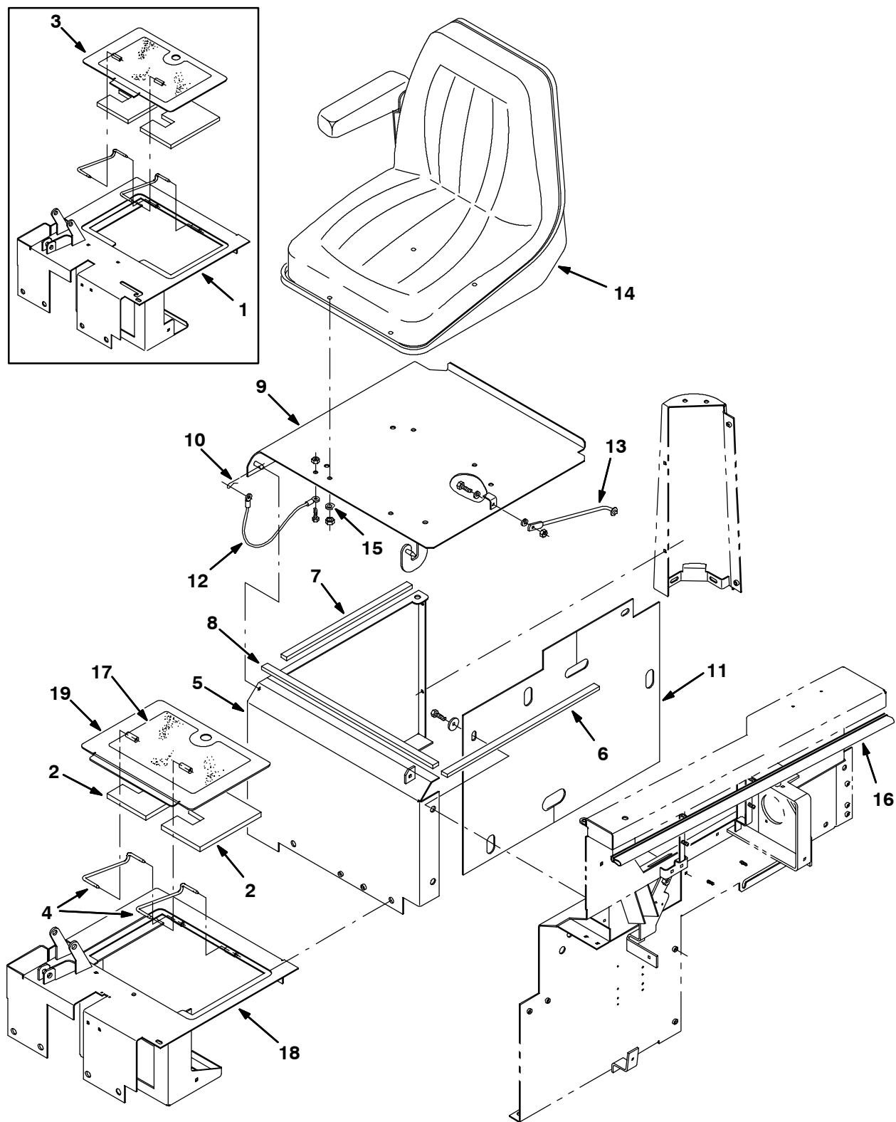
Fig. 6 - Seat and Shroud Group
