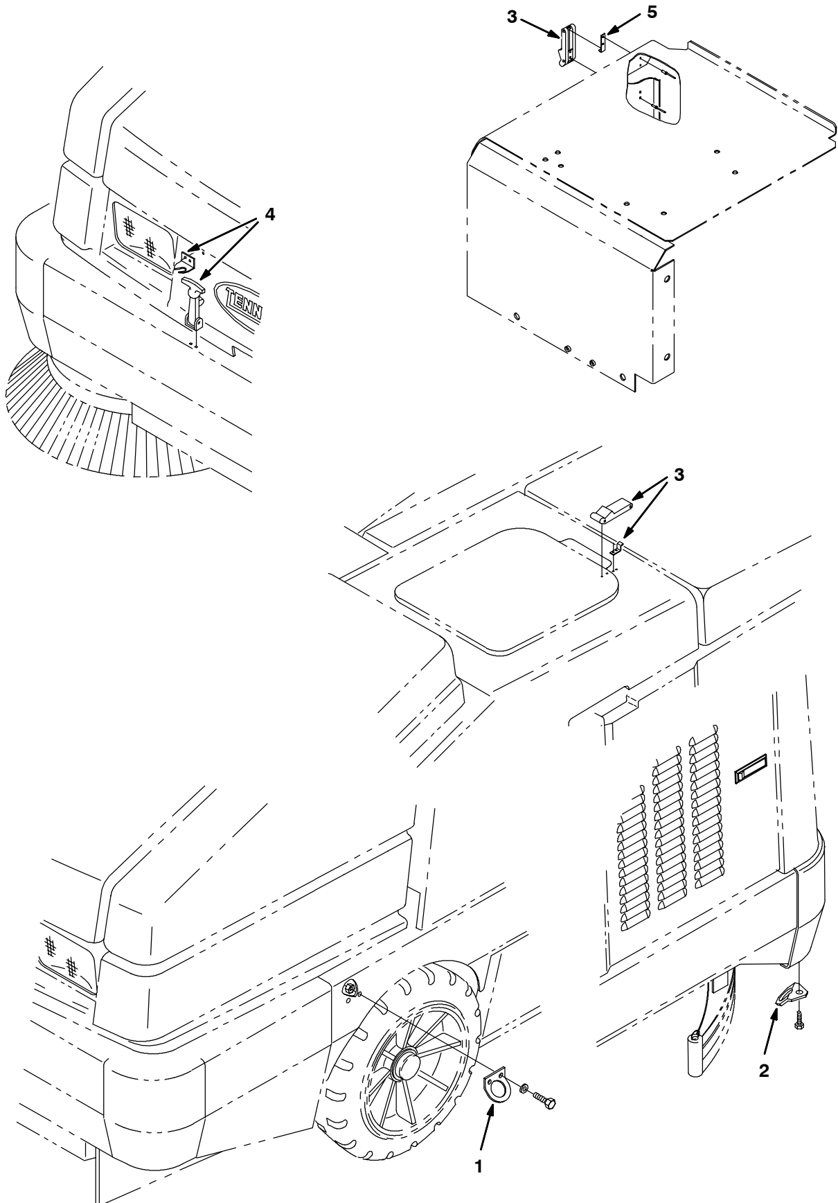
Fig. 27 - Demo Kit
