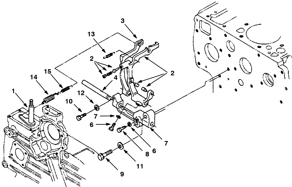
Fig. 16 - Governor
