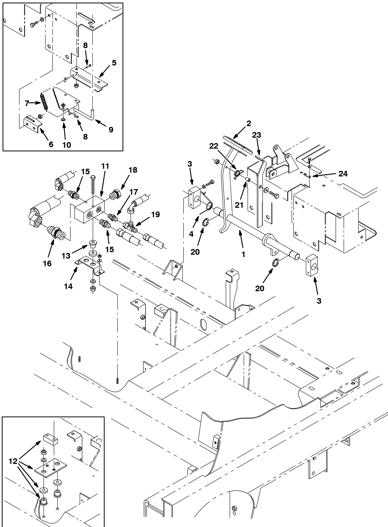
Fig. 31 - Brake Pedals Group
