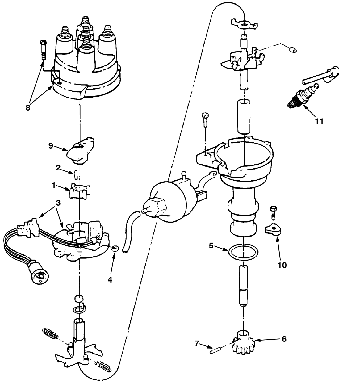
Fig. 13 - Ignitions Group
