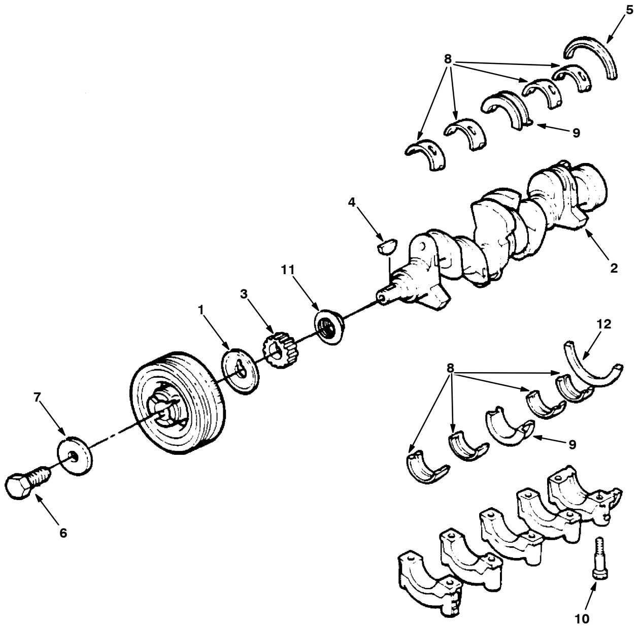
Fig. 7 - Crankshaft Group
