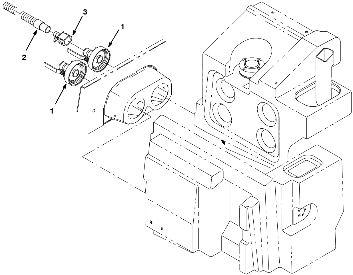
Fig. 23 - Positive Solution Control Drain System Kit ES
