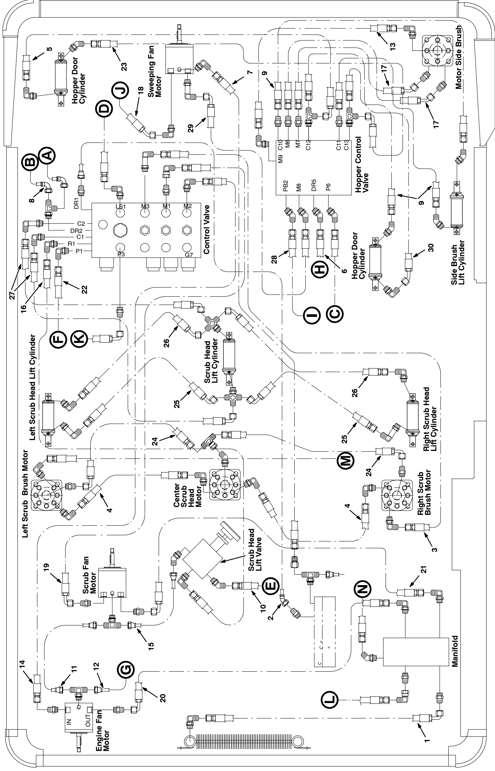
Fig. 42 - Hydraulic Hose Group
