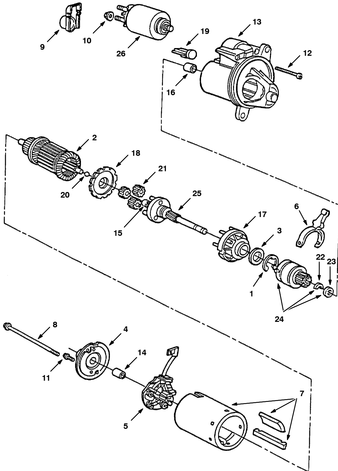
Fig. 14 - Starter Breakdown
