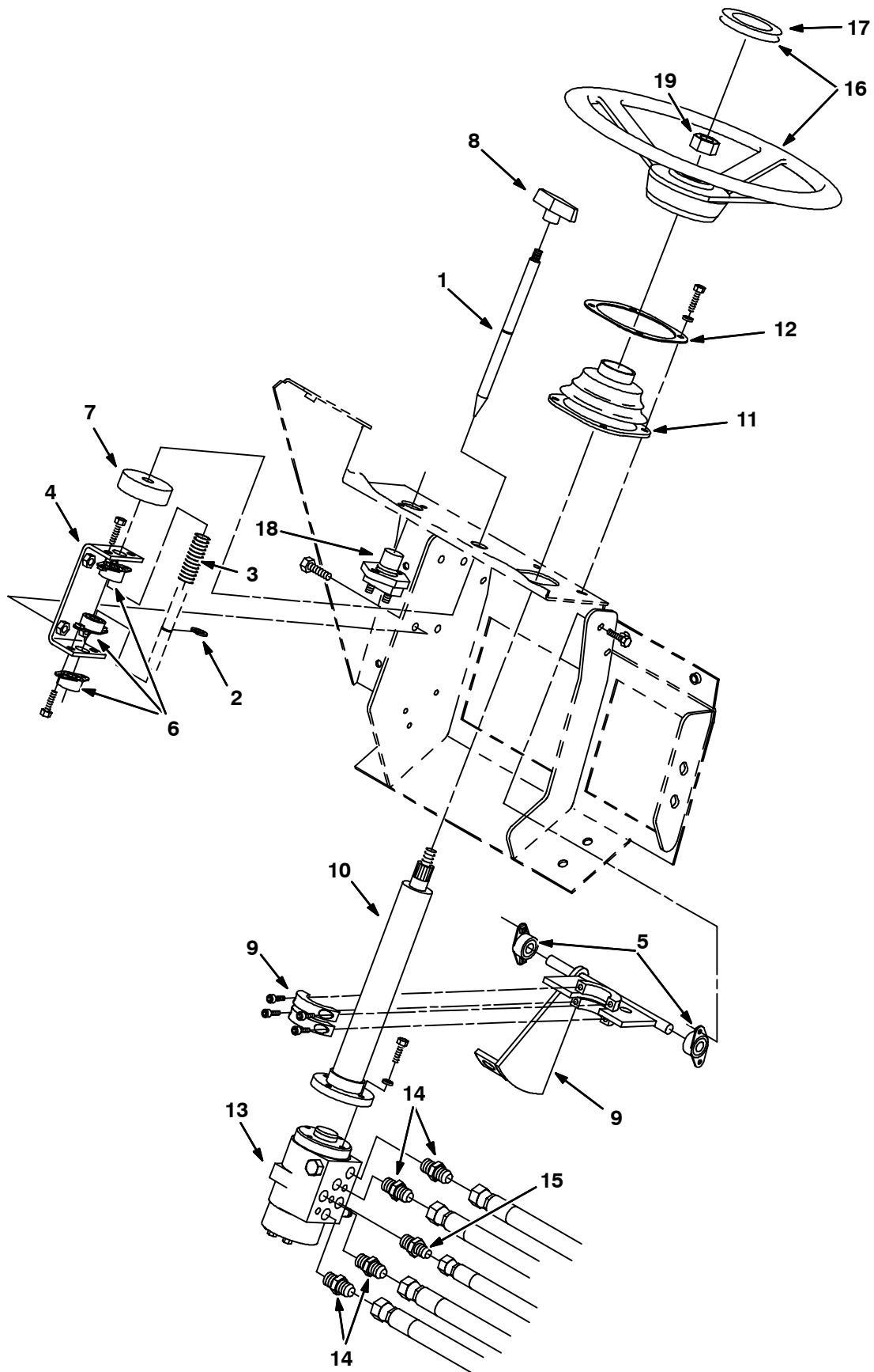
Fig. 62 - Steering Group
