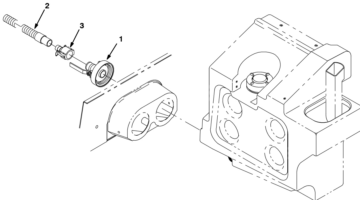
Fig. 22 - Positive Solution Control Drain System Kit Std
