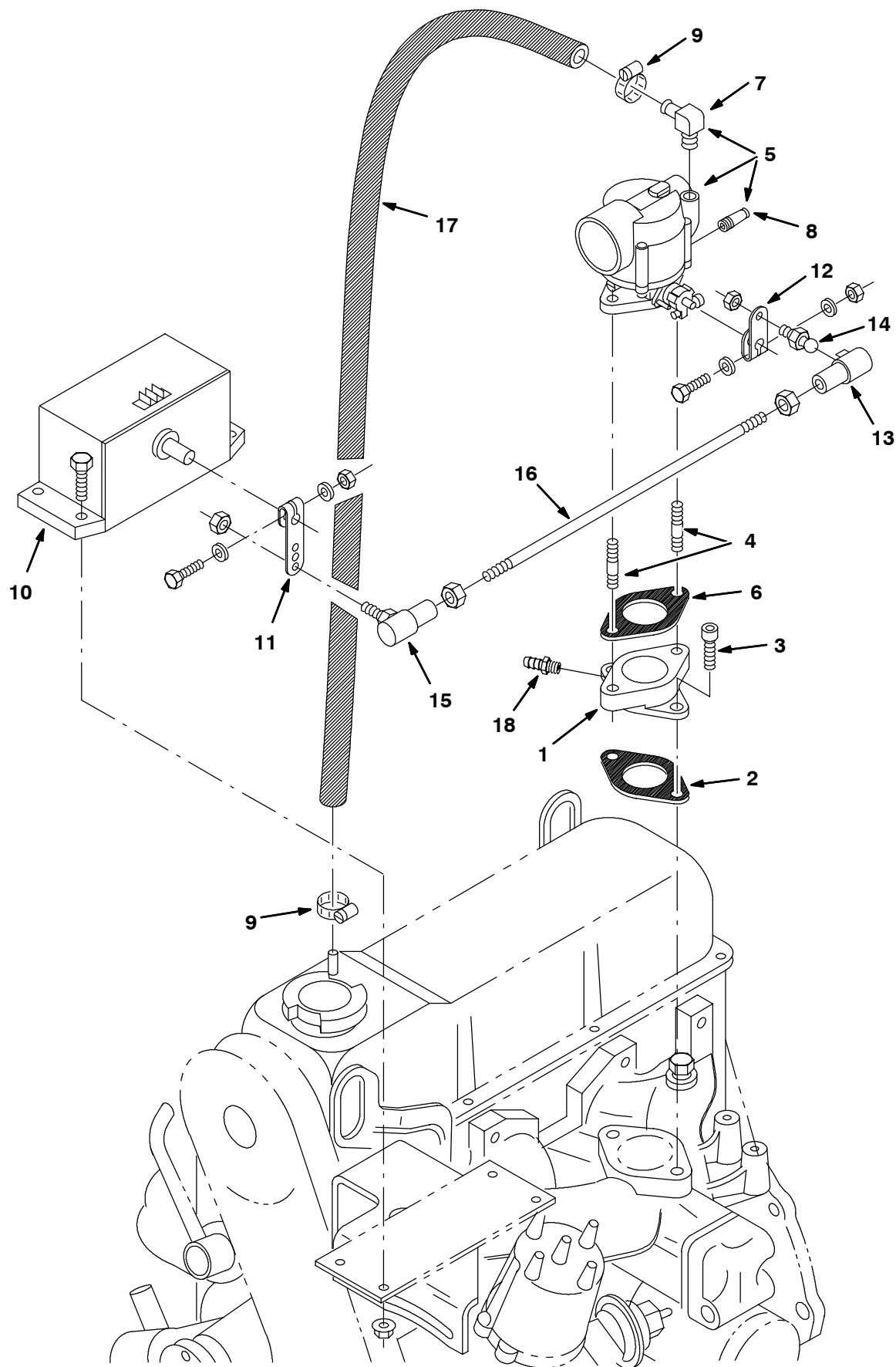
Fig. 23 - Carburetor Group, LPG
