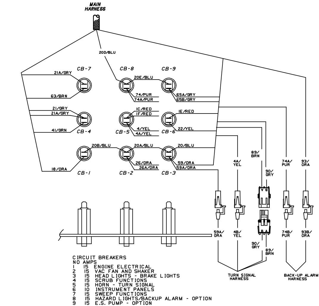
Fig. 67 - Wire Harnesses Group
