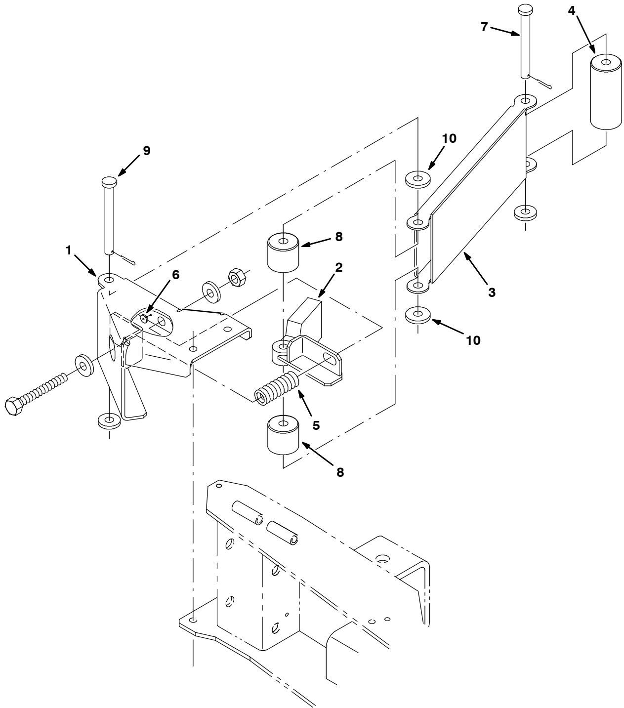
Fig. 28 - Side Squeegee Kit SE
