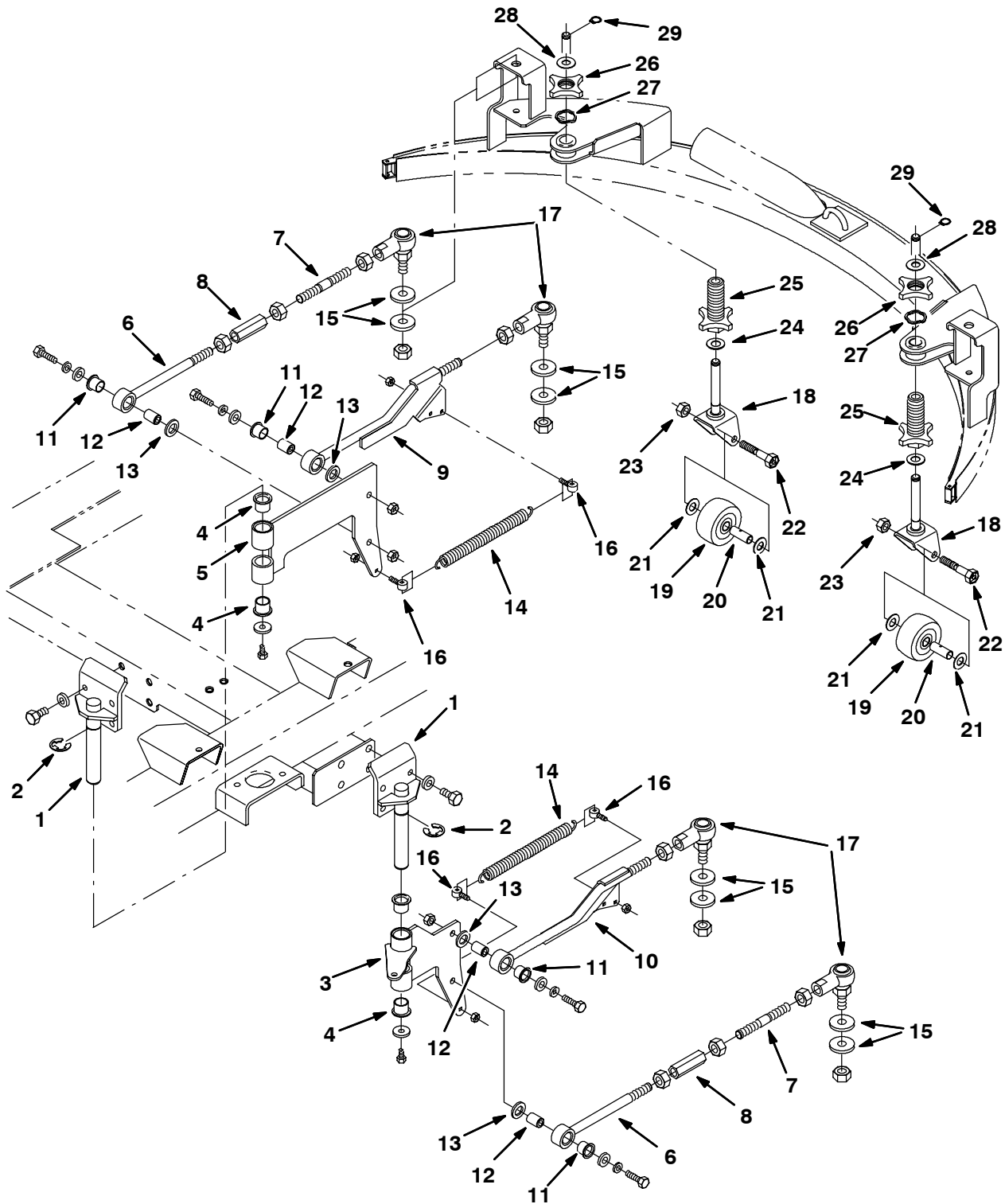
Fig. 56 - Rear Squeegee Linkage Group
