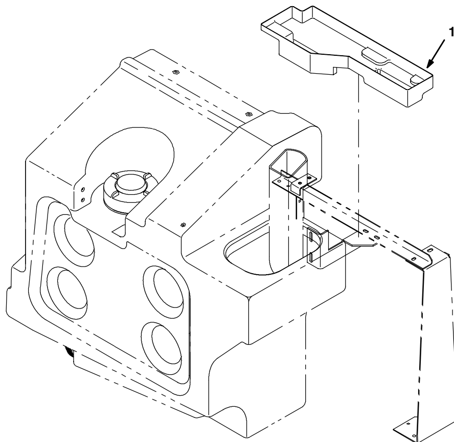
Fig. 24 - Drip Tray Group
