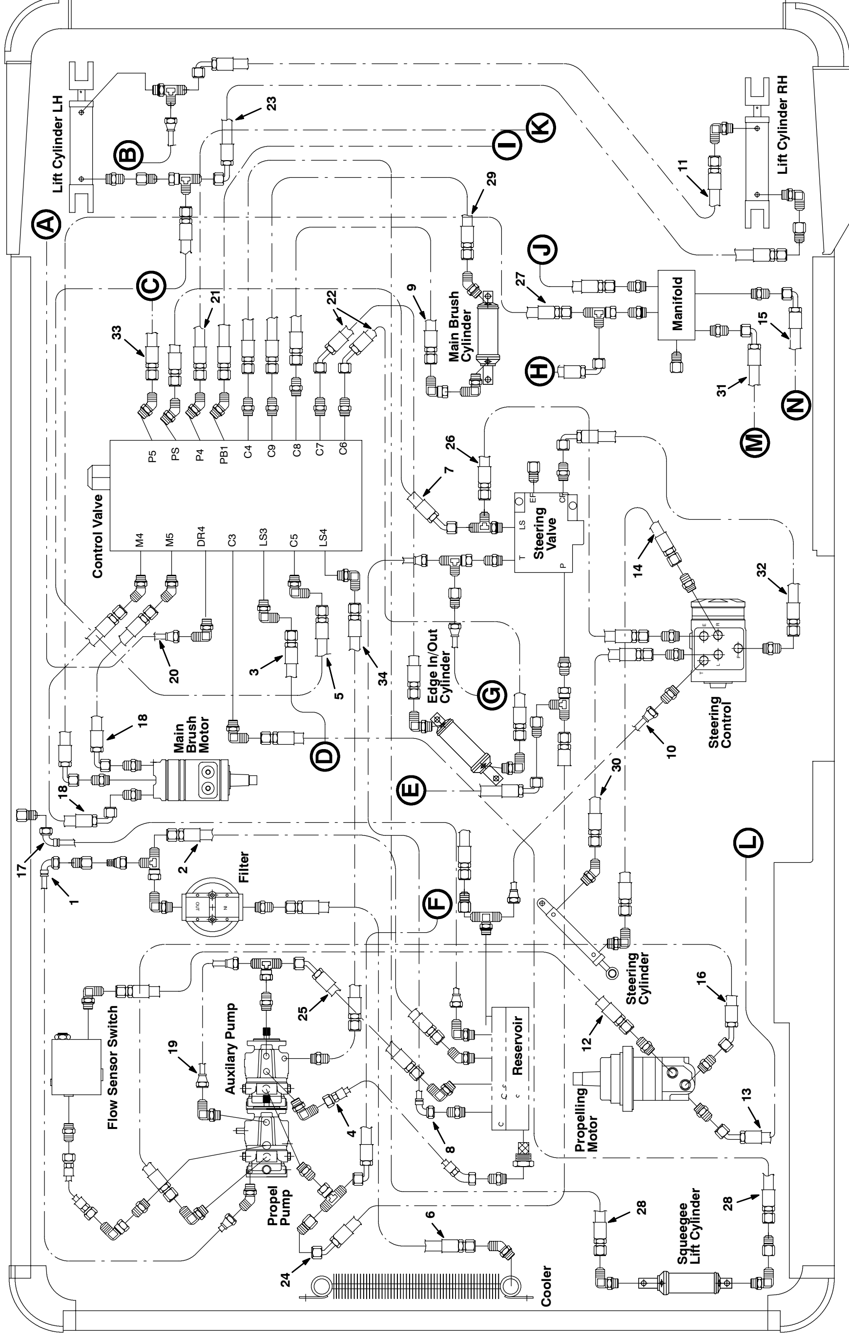
Fig. 41 – Hydraulic Hose Group
