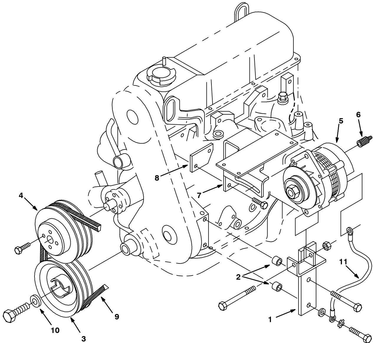
Fig. 21 - Alternator Group
