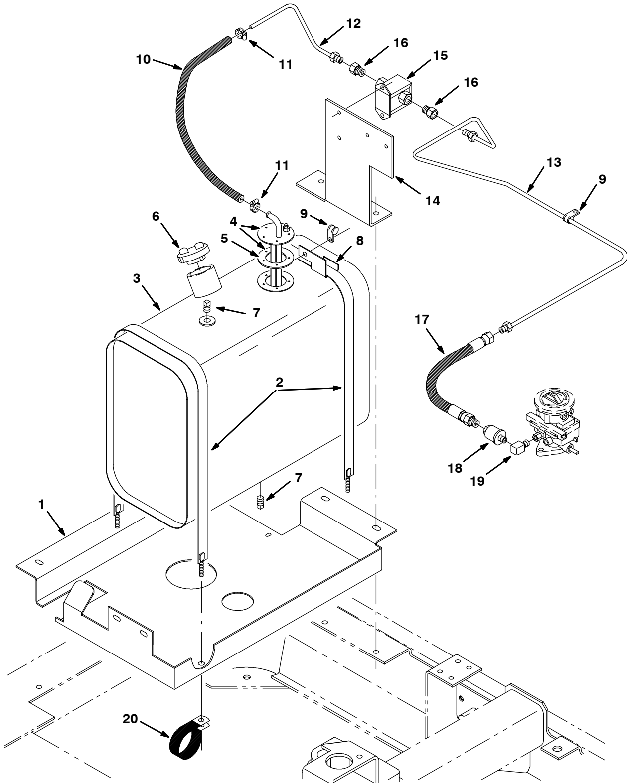
Fig. 27 - Fuel Tank Group, Gasoline
