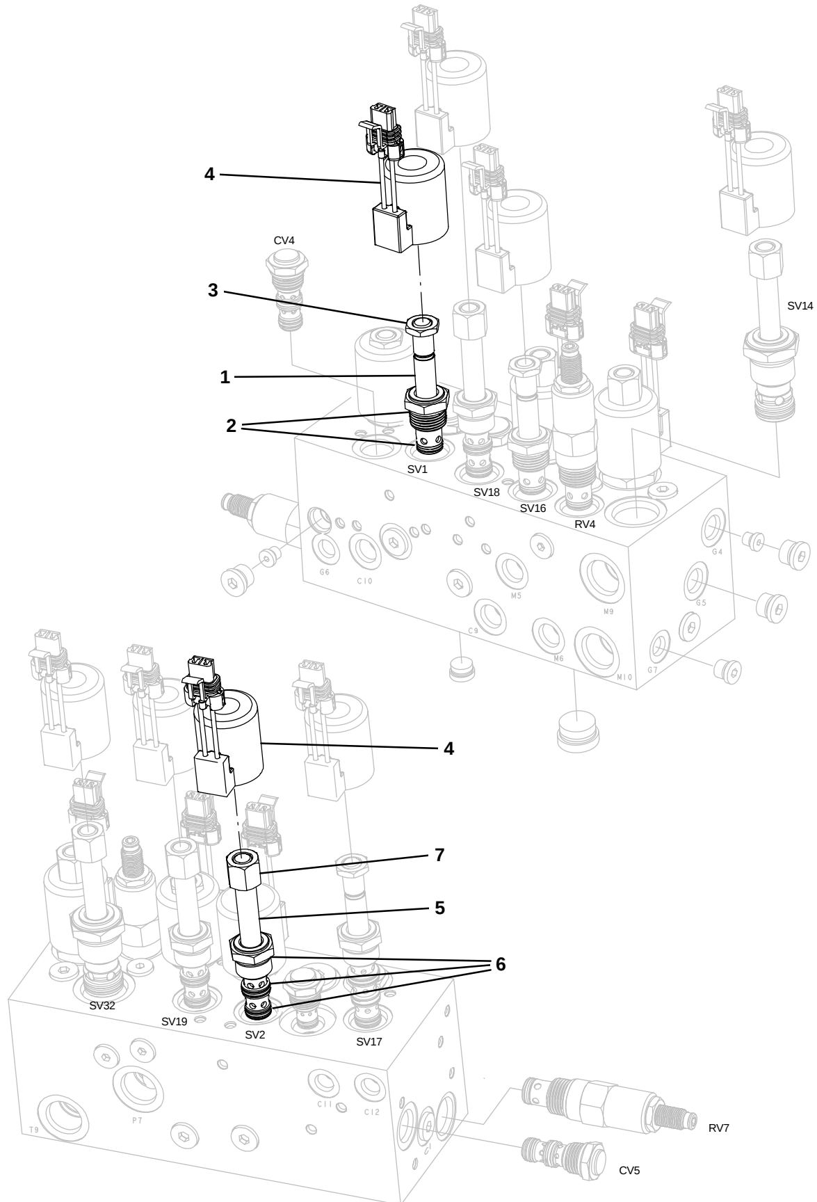
Fig. 25 – Hydraulic Solenoid Valve Breakdown, 1053642 (For High Dump Hopper Lift Option)
