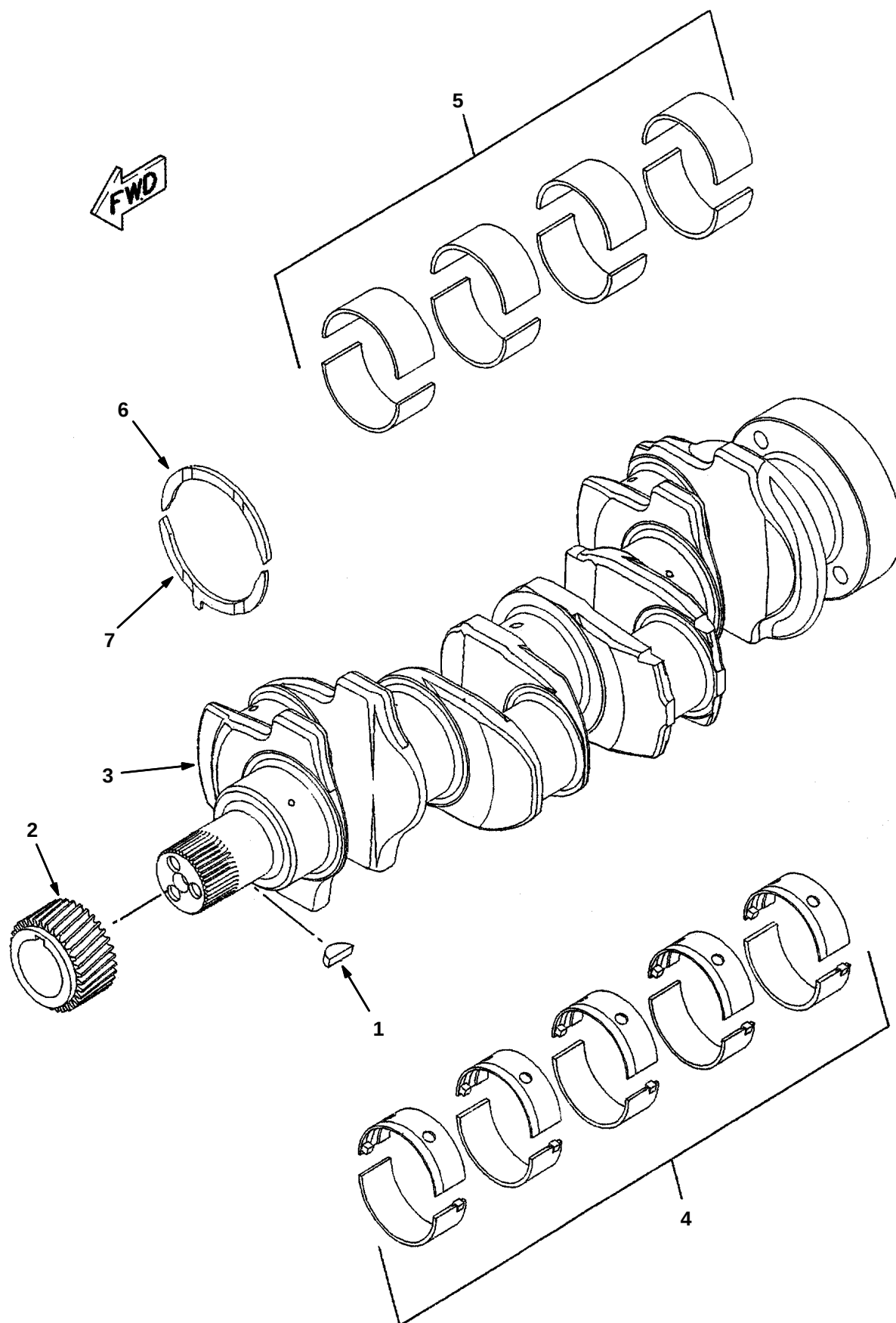
Fig. 22 – Crankshaft Group
