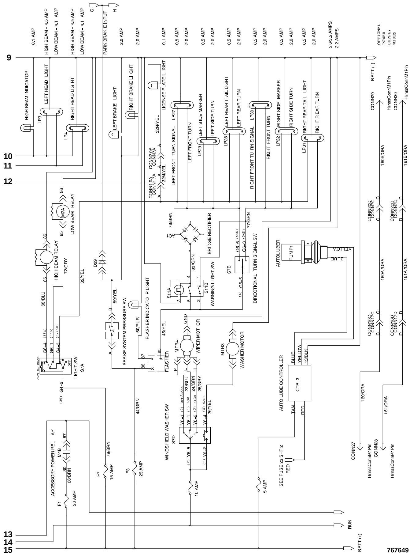
Fig. 75 – Electrical Schematic (000000-008499)
