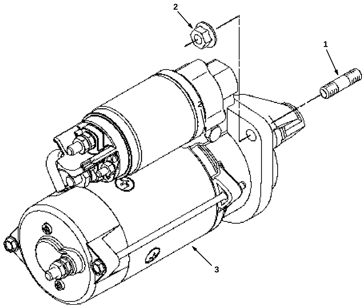
Fig. 24 – Starter Group
