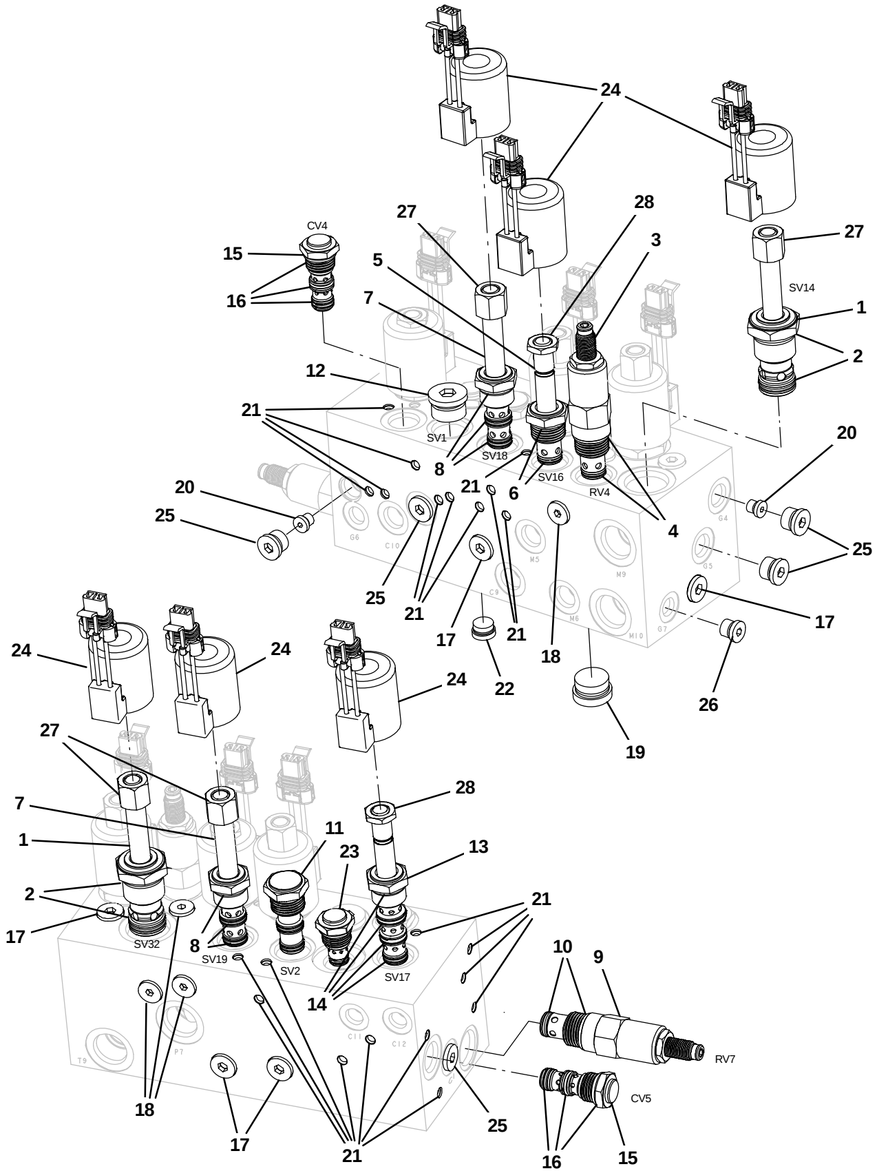
Fig. 24 – Hydraulic Solenoid Valve Breakdown, 1053642
