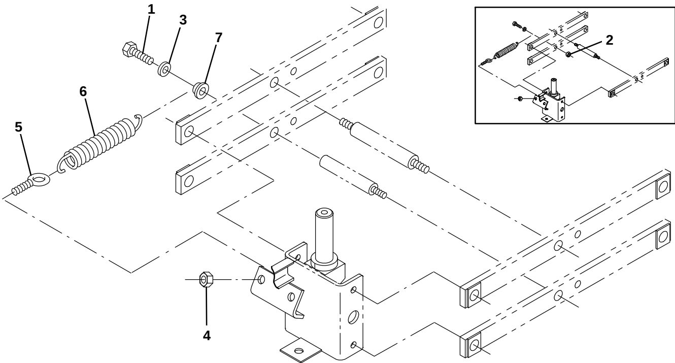
Fig. 43 – Side Brush Spring Kit
