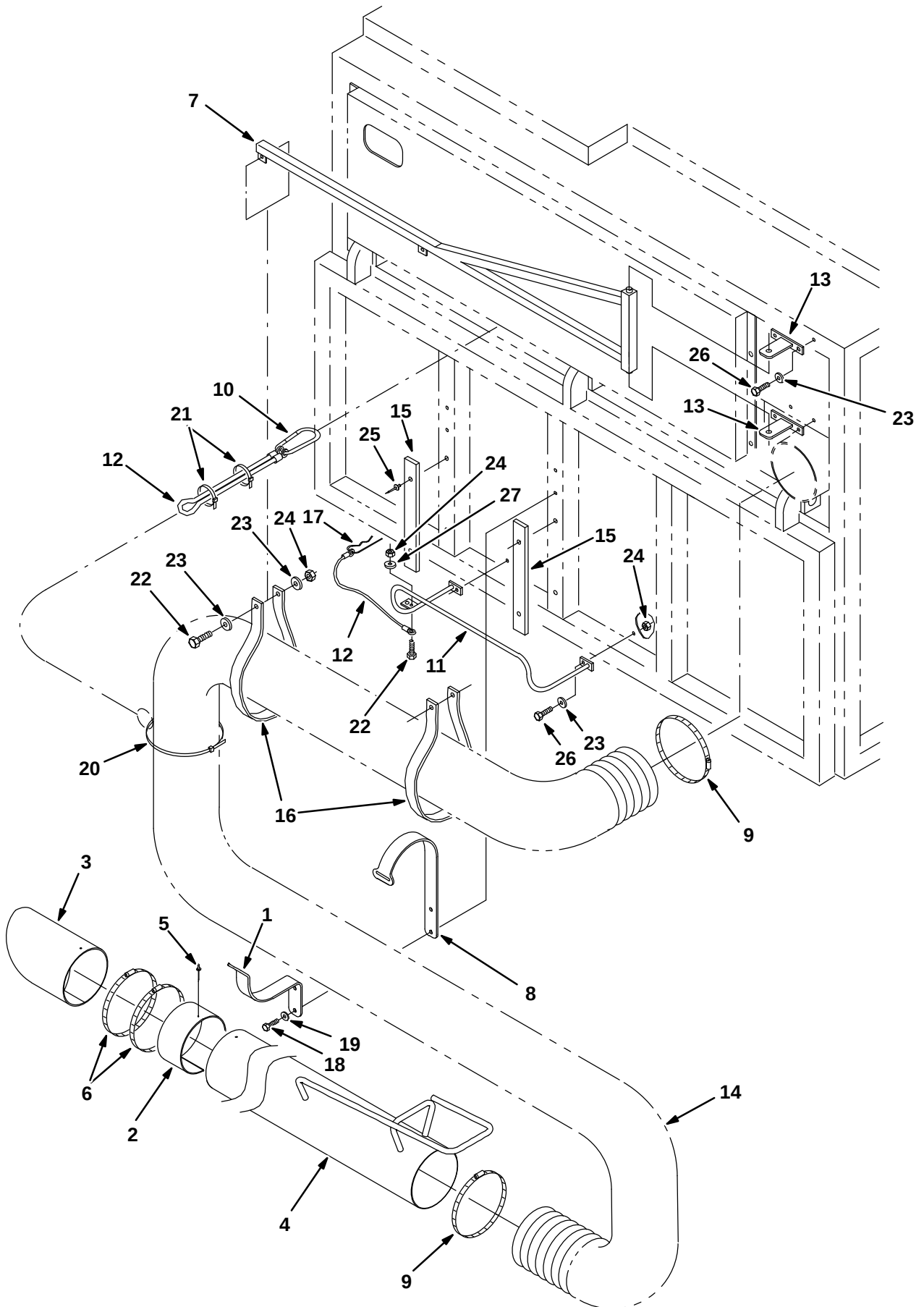
Fig. 22 – Vacuum Wand Group
