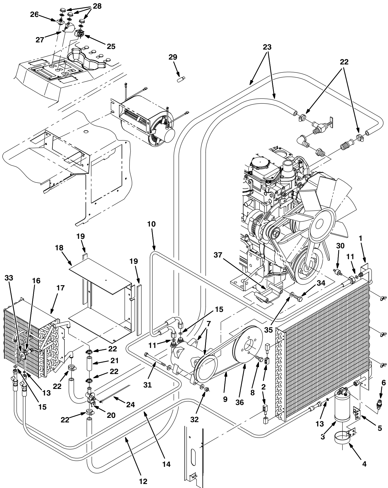
Fig. 21 – Cab Air Conditioner Heater Group
