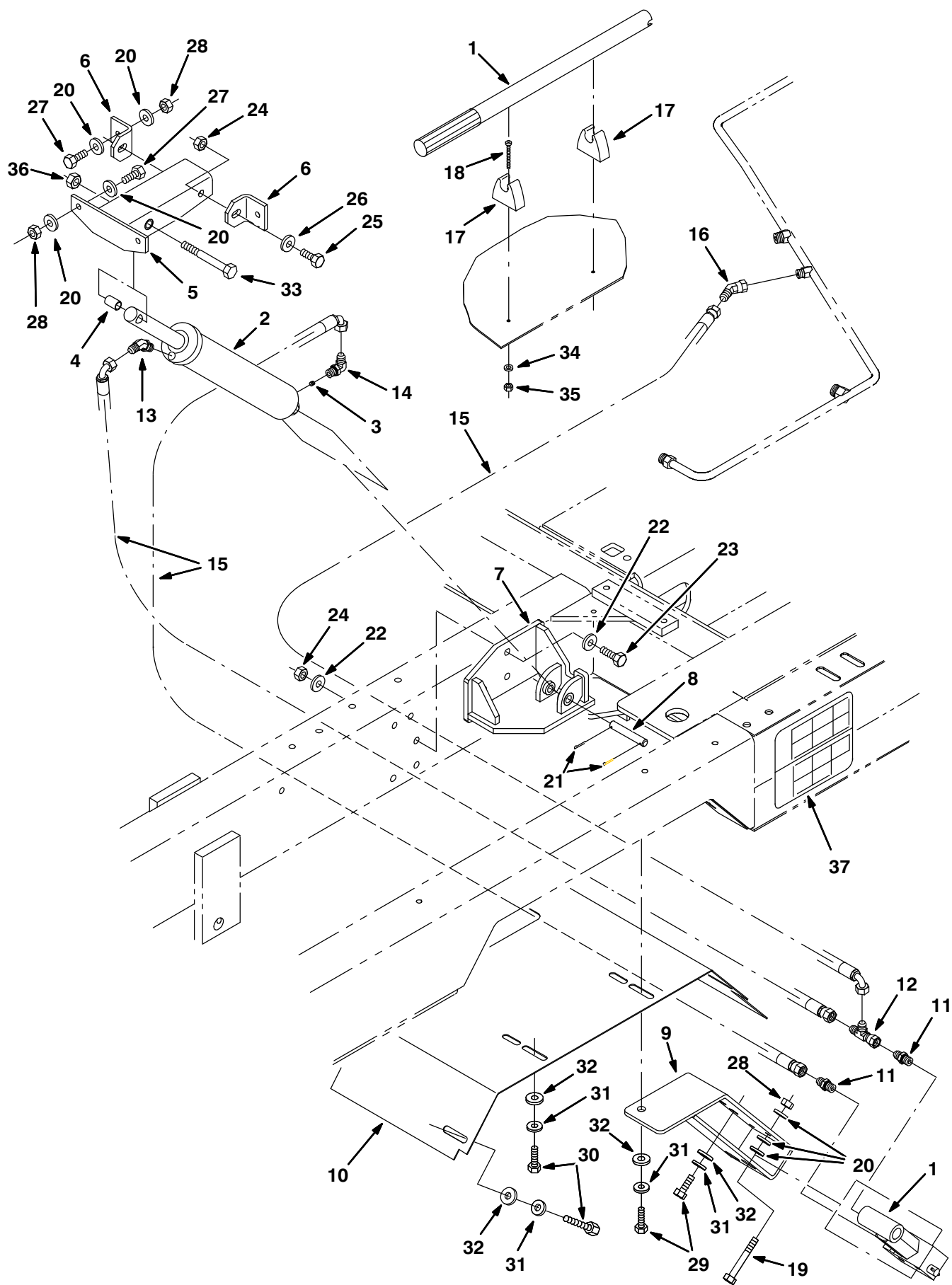
Fig. 18 – Cab Jack Kit
