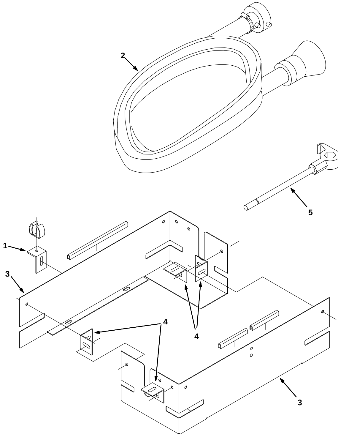
Fig. 31 – Hydrant Wash Down Group
