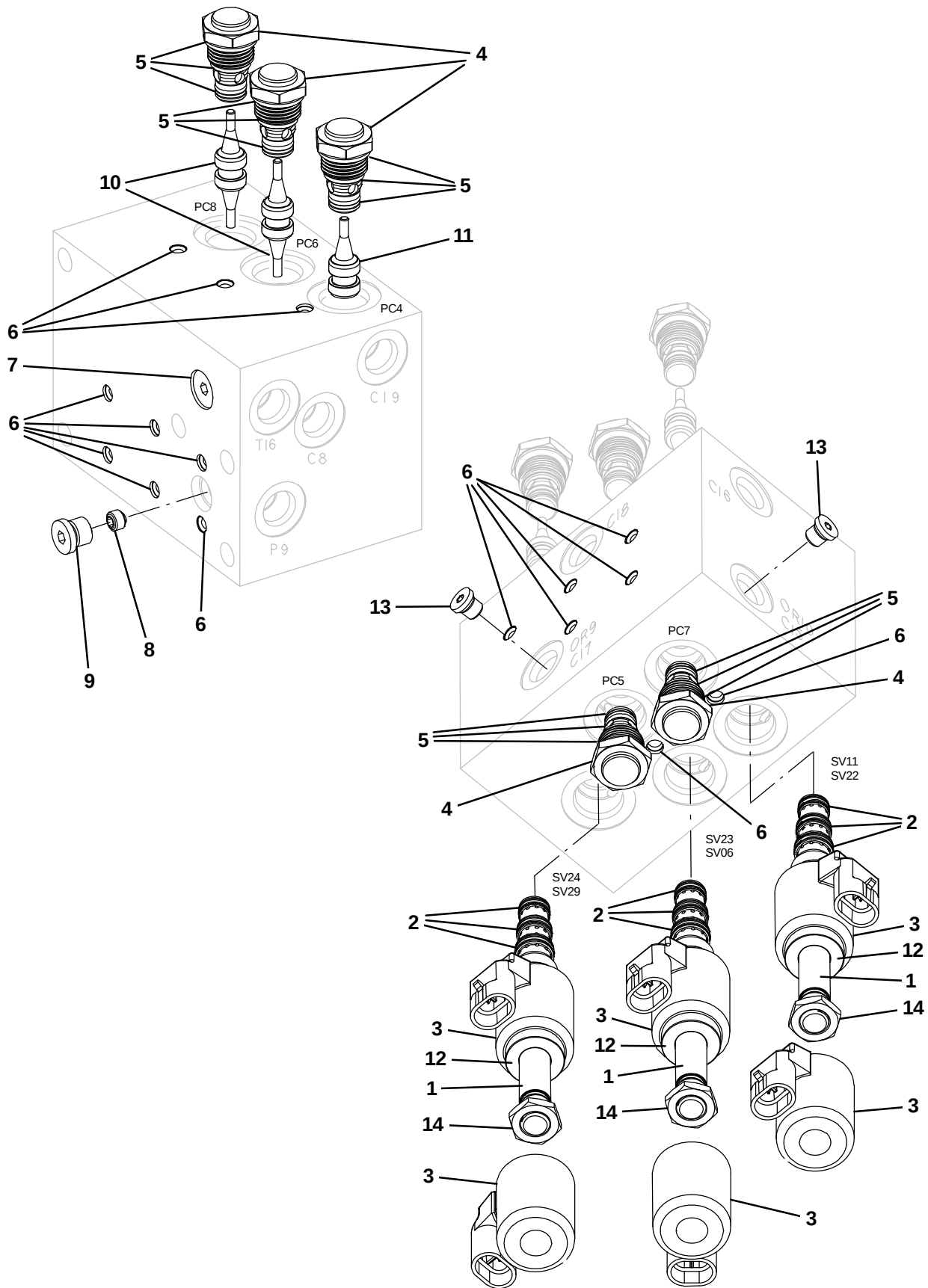
Fig. 30 – Hydraulic Solenoid Valve Breakdown, 1053648
