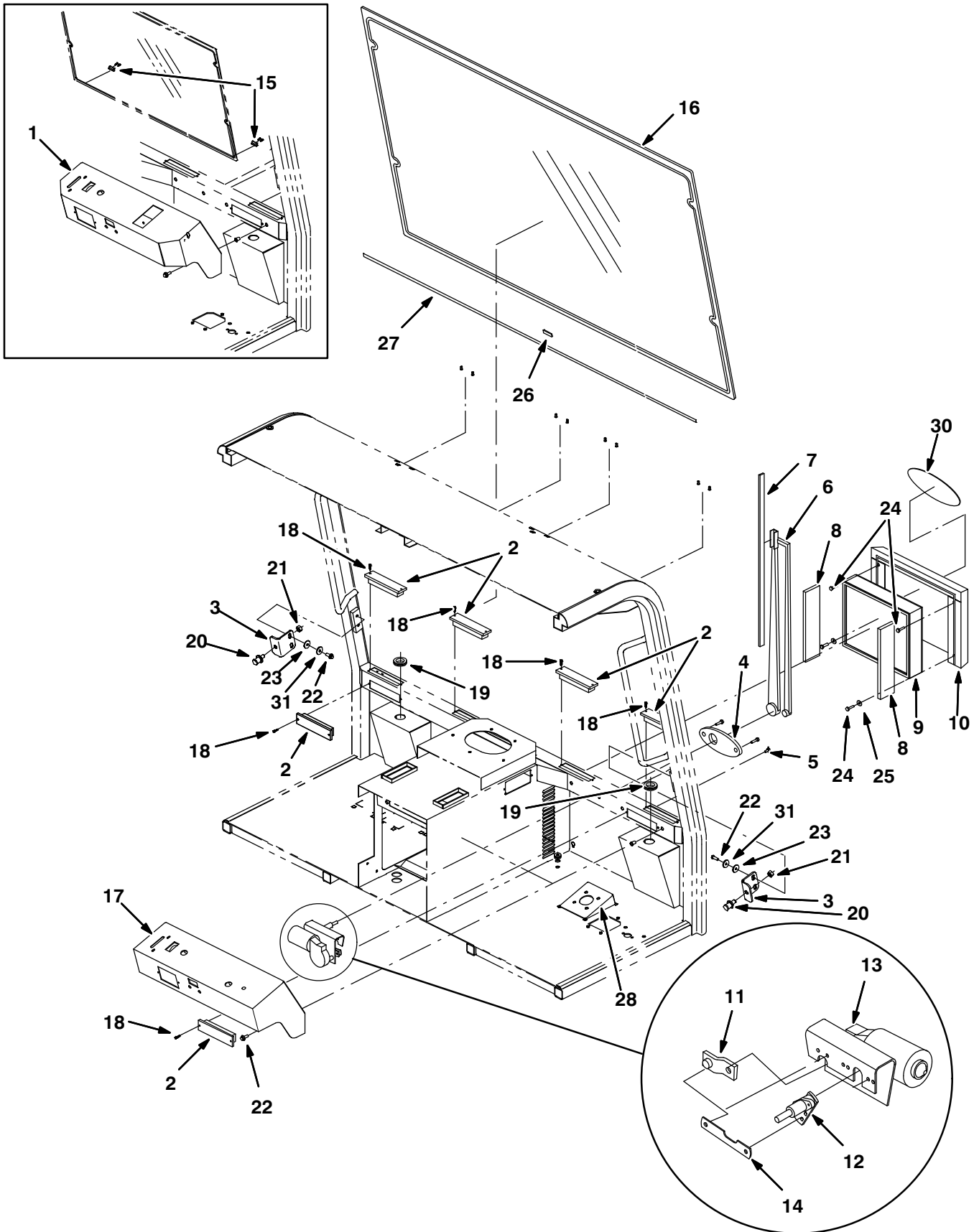
Fig. 39 – Cab Group, Front
