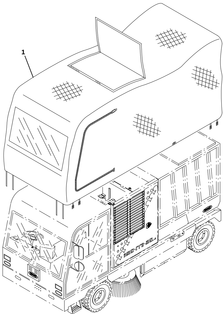
Fig. 45 – Storage Kit
