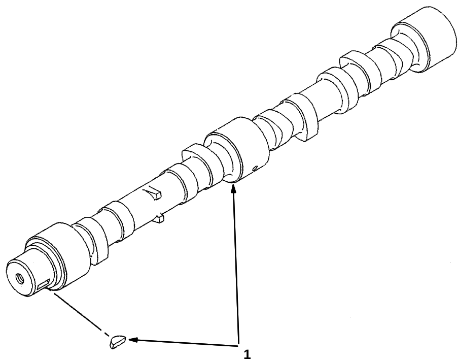
Fig. 21 – Camshaft Group
