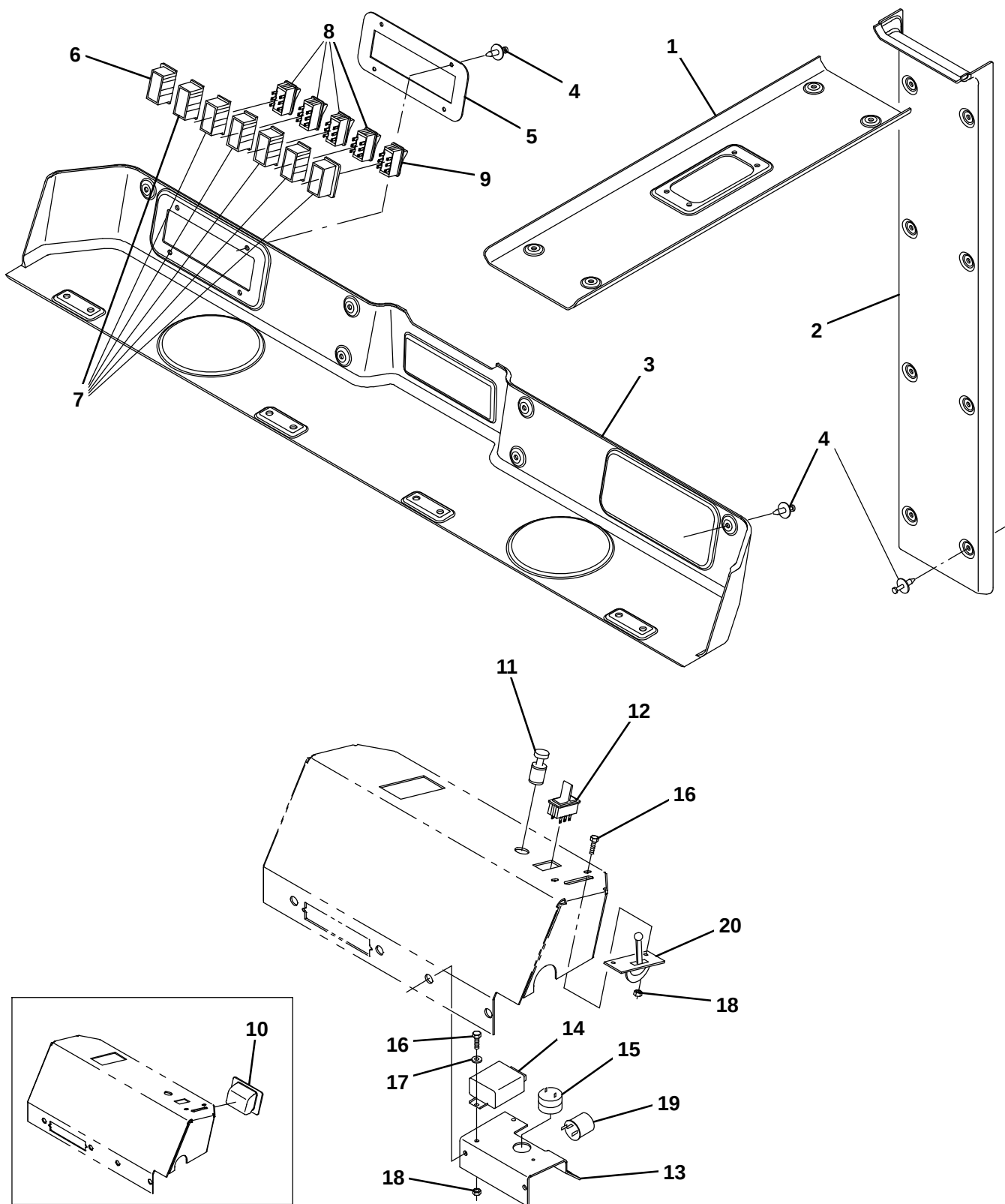
Fig. 46 – Cab Upper and Front Console Group
