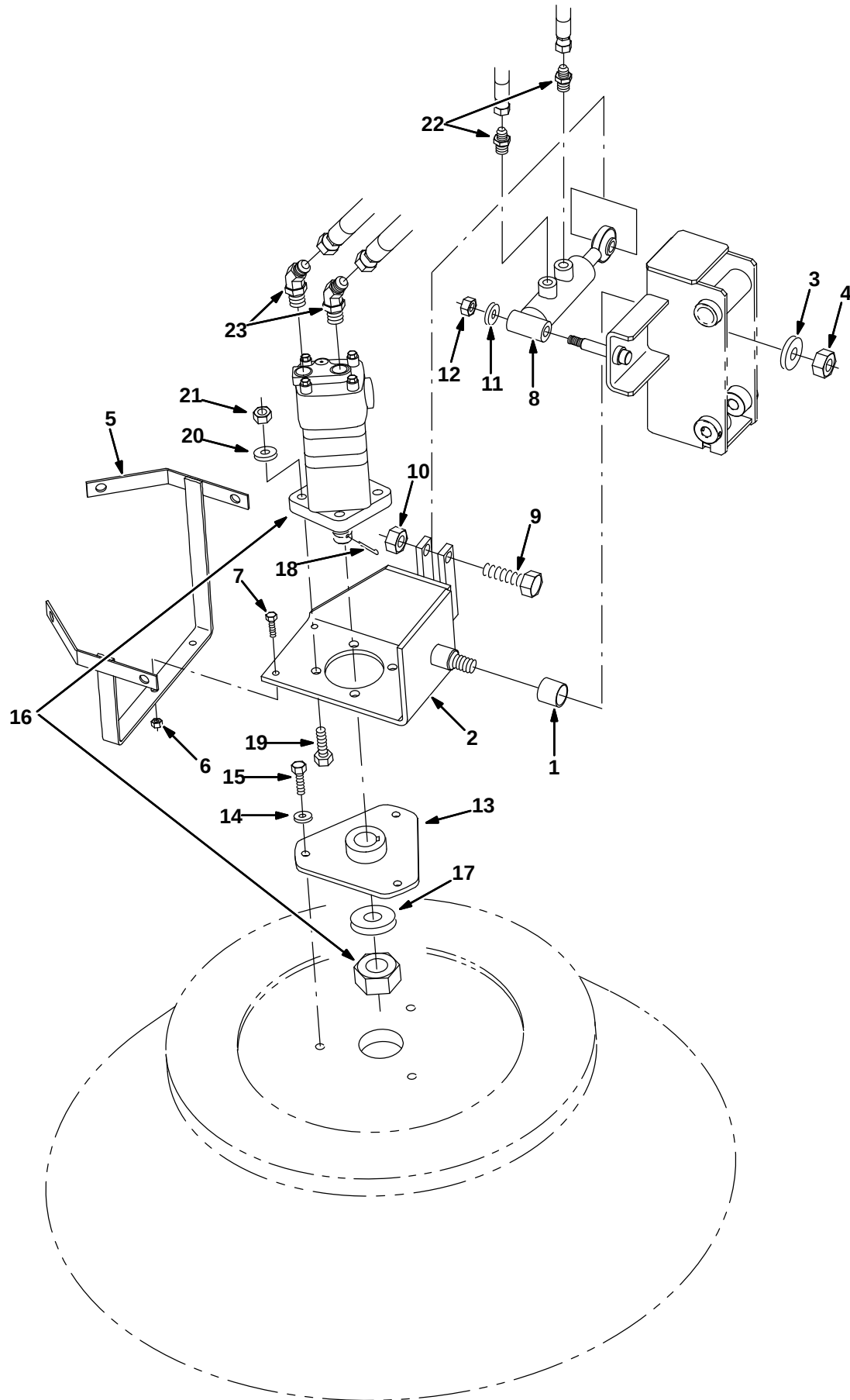
Fig. 11 – Vario Brush Motor Group
