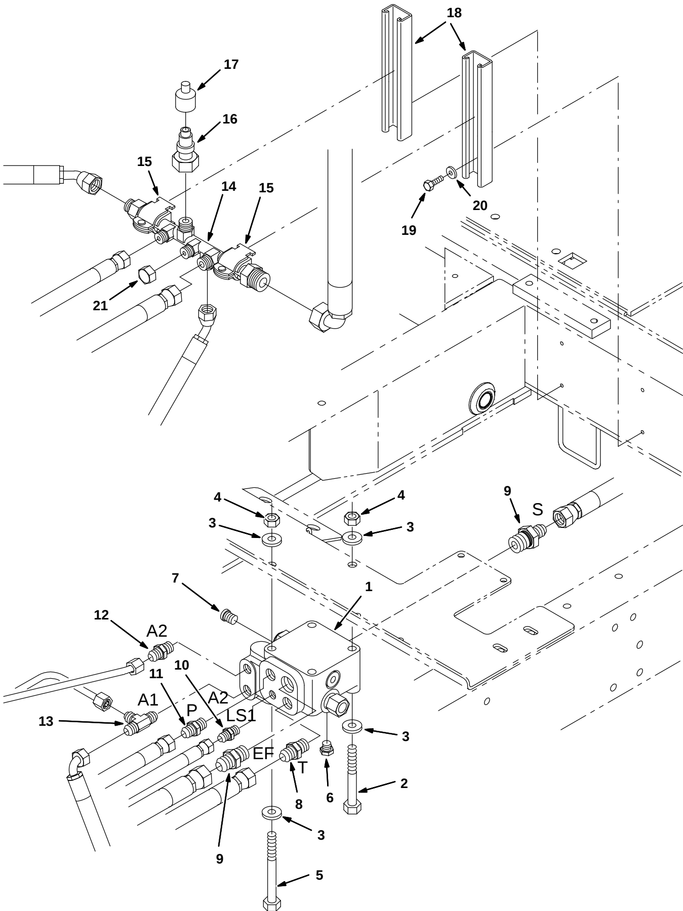
Fig. 70 – Hydraulic Manifold and Priority Valve Group
