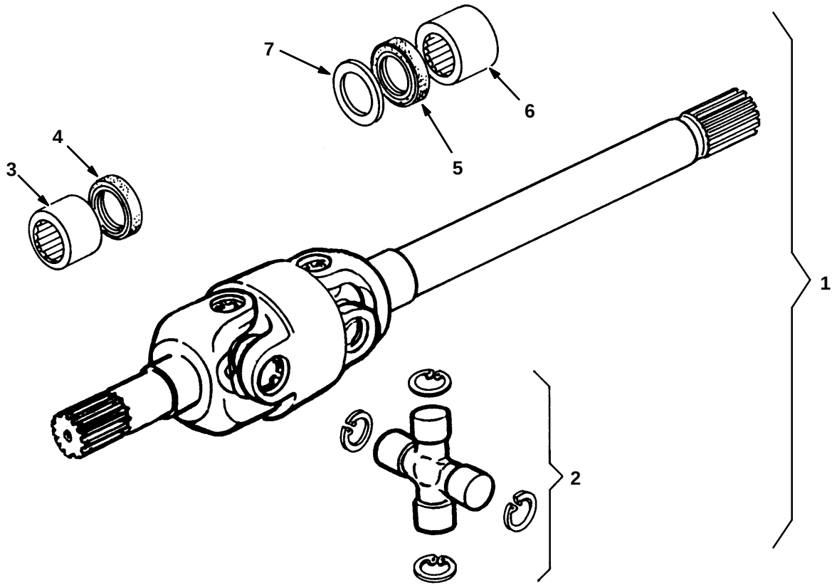
Fig. 10 – Axle CV Joint Breakdown, Front
