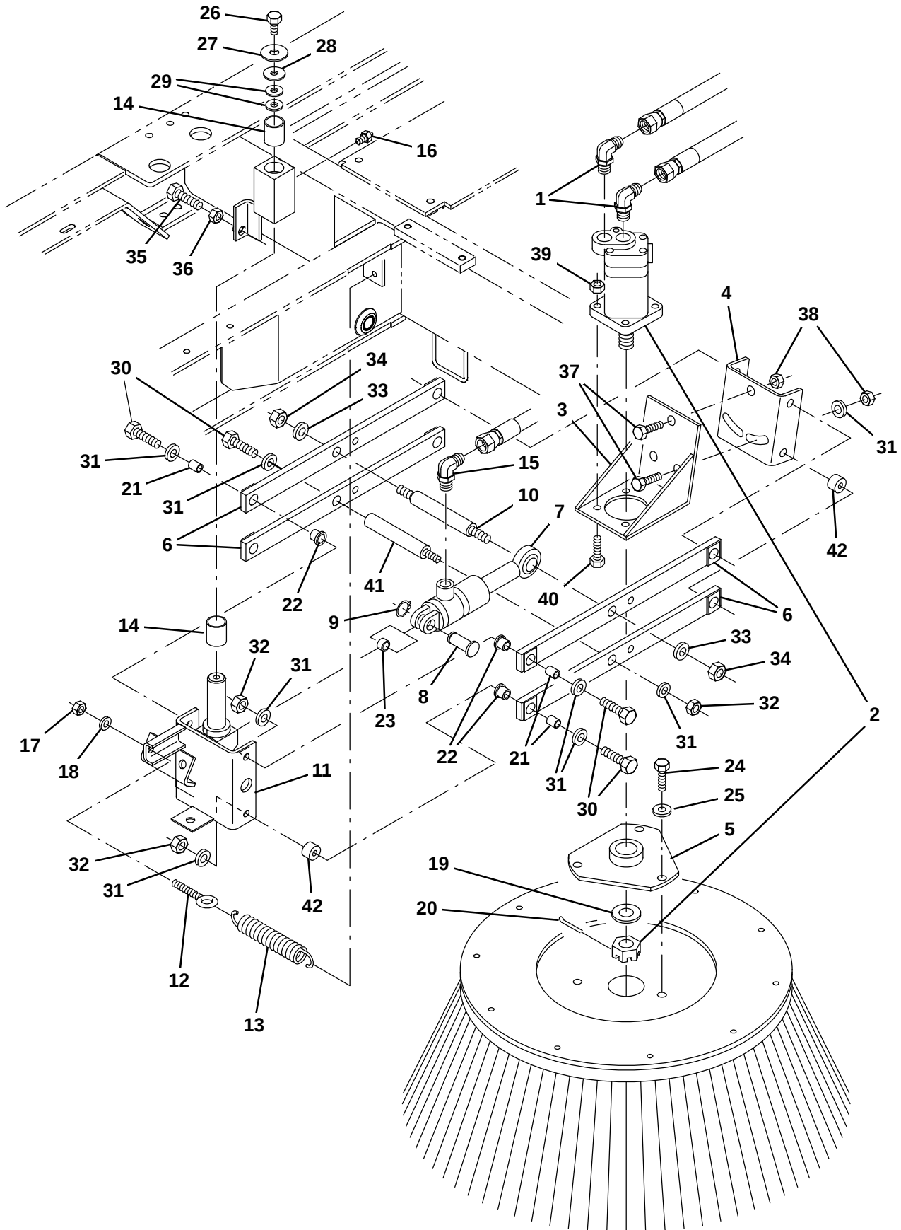
Fig. 54 – Brush Group, Right Side (009838– )
