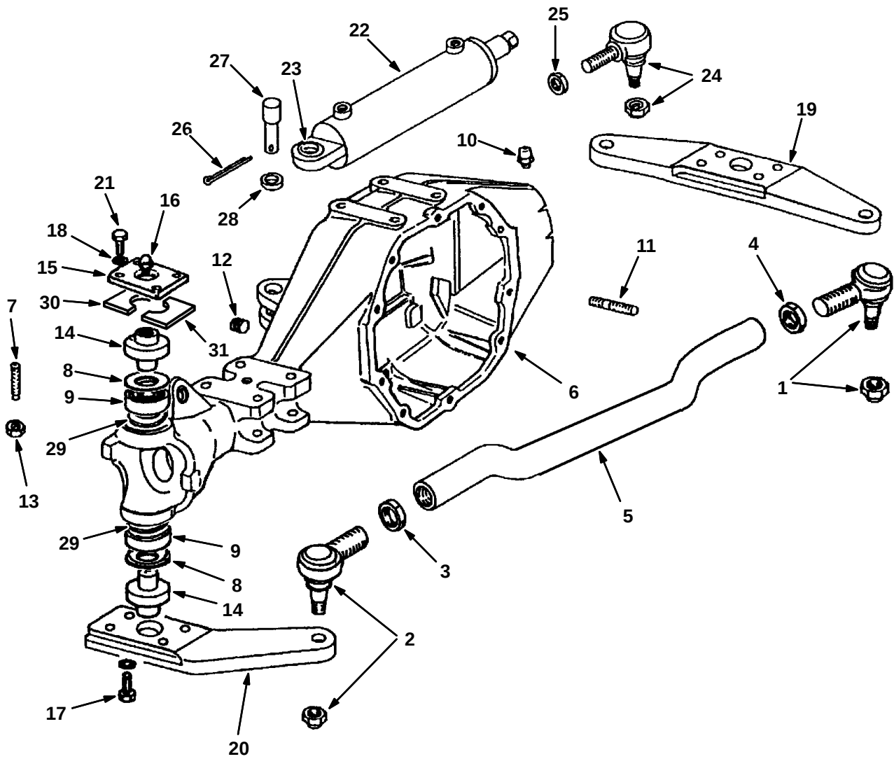
Fig. 6 – Axle And Spindle Breakdown, Front
