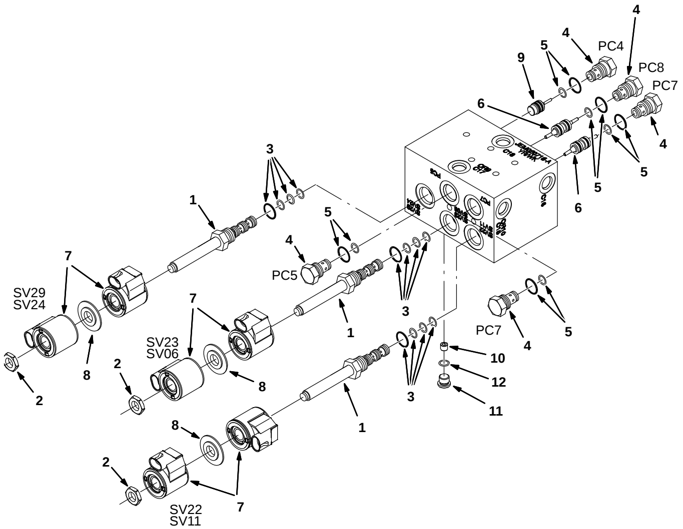
Fig. 23 – Hydraulic Solenoid Valve Breakdown, 771012
