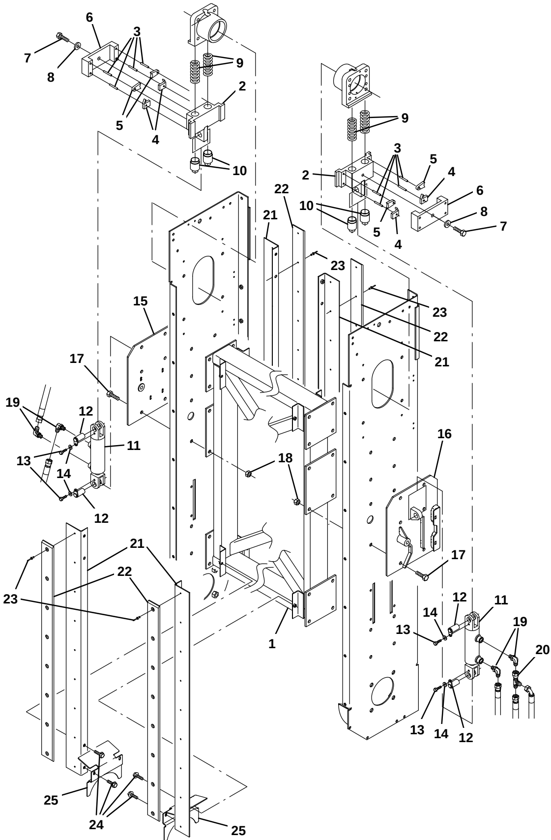
Fig. 31 – Conveyor Tension Group
