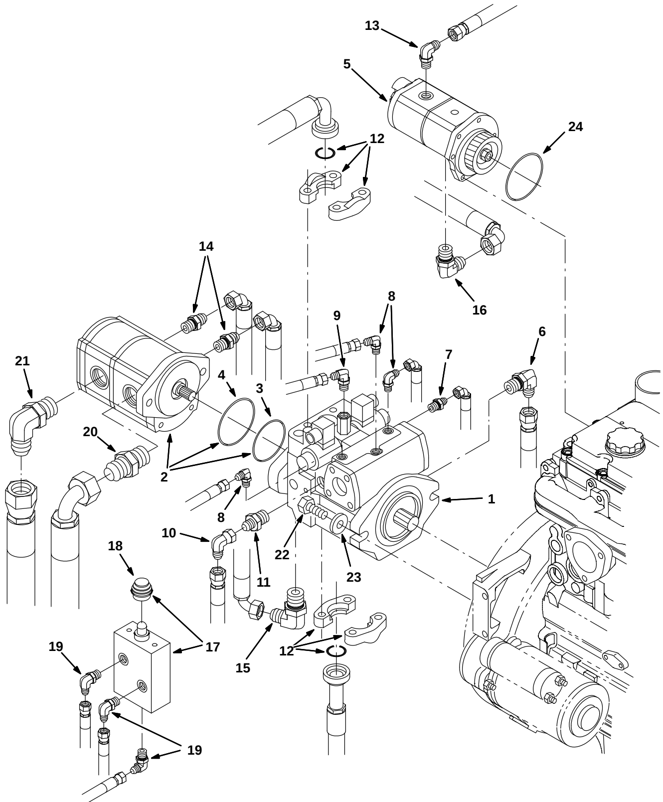
Fig. 65 – Hydraulic Pumps Group
