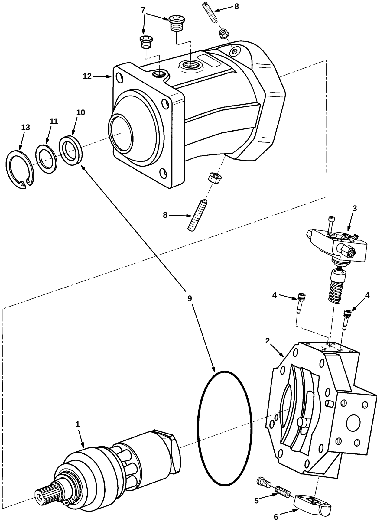
Fig. 3 – Hydraulic Piston Motor Breakdown, 762136
