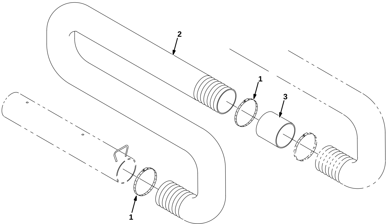
Fig. 24 – Vacuum Wand Extension Group
