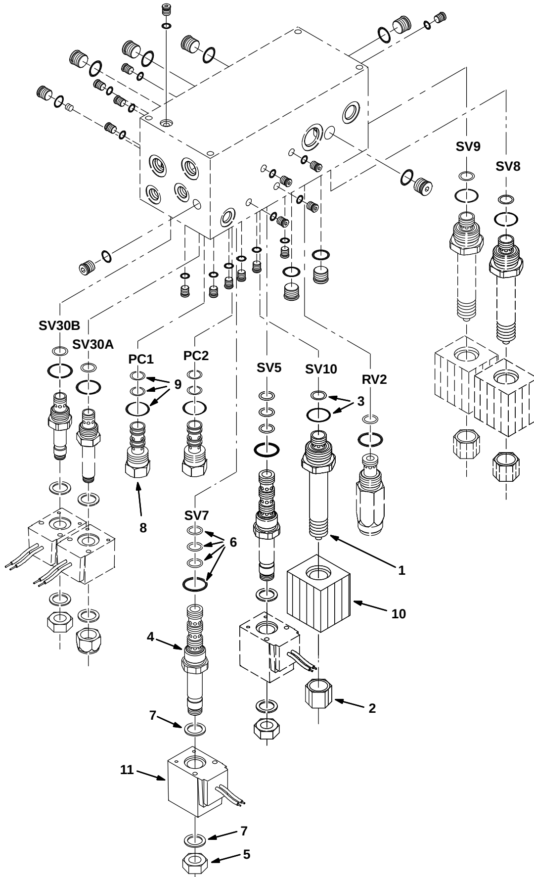
Fig. 20 – Hydraulic Solenoid Valve Breakdown, 771010 (For Left Hand Side Brush Option)
