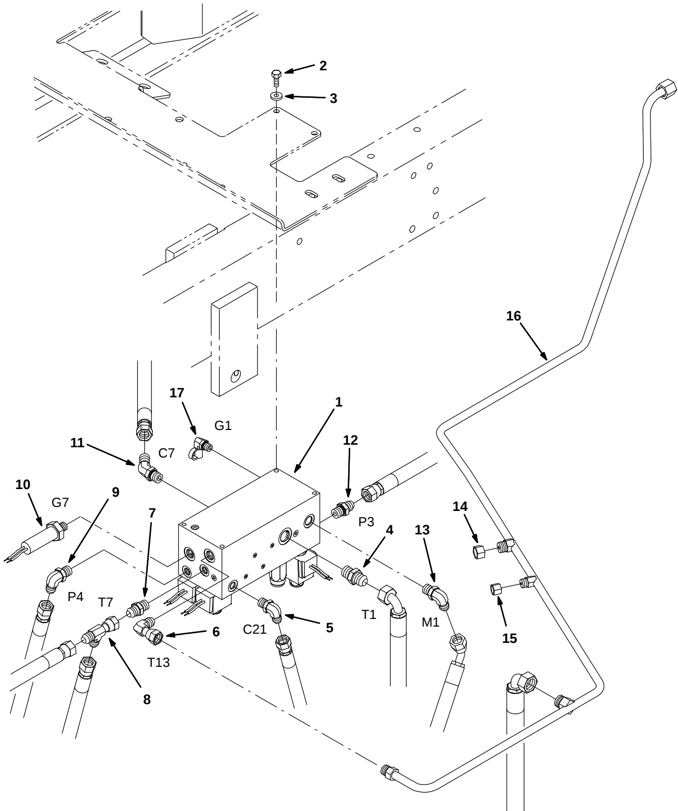
Fig. 69 – Hydraulic Side Brush Valve Group
