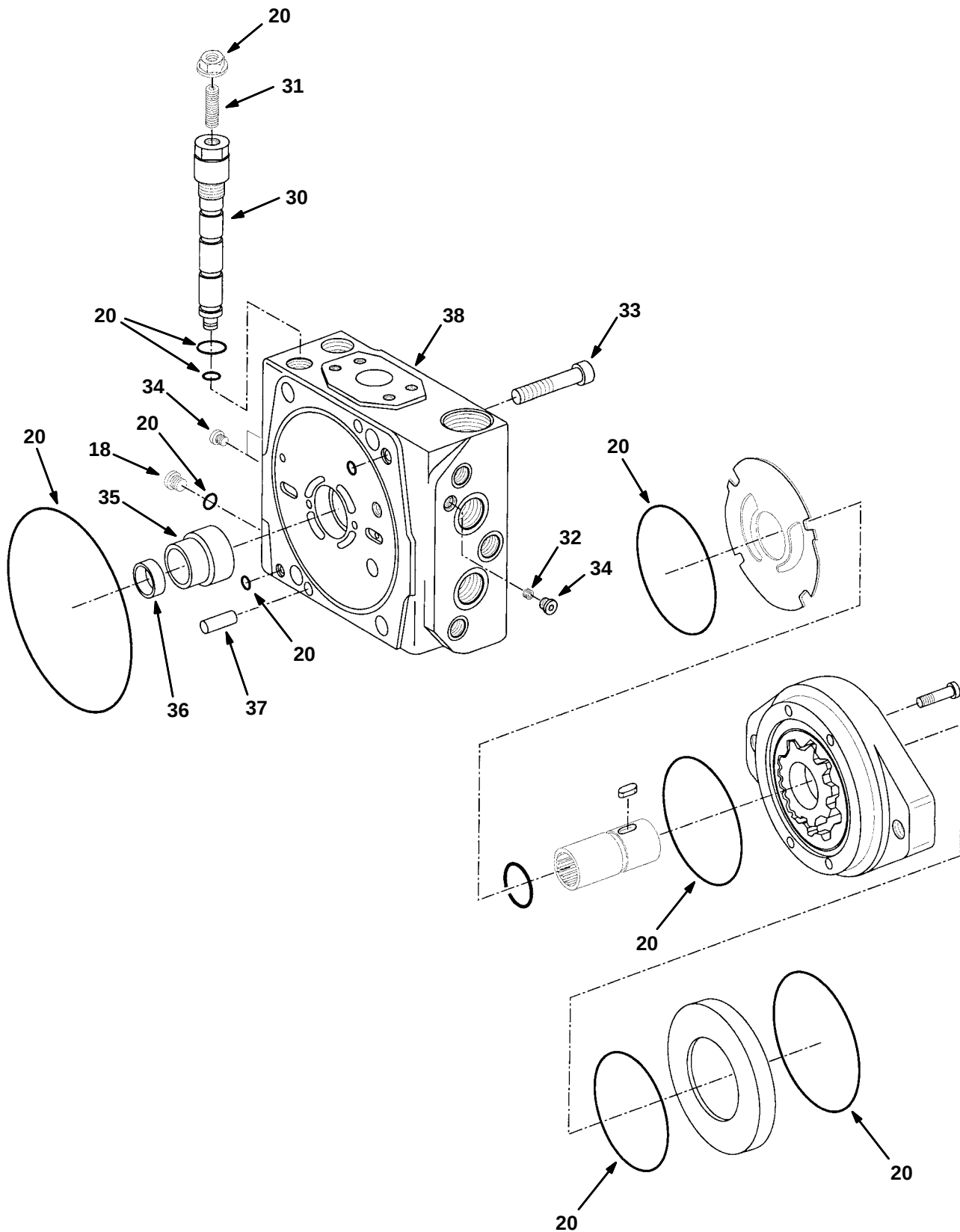
Fig. 2 – Hydraulic Piston Pump Breakdown, 1066392
