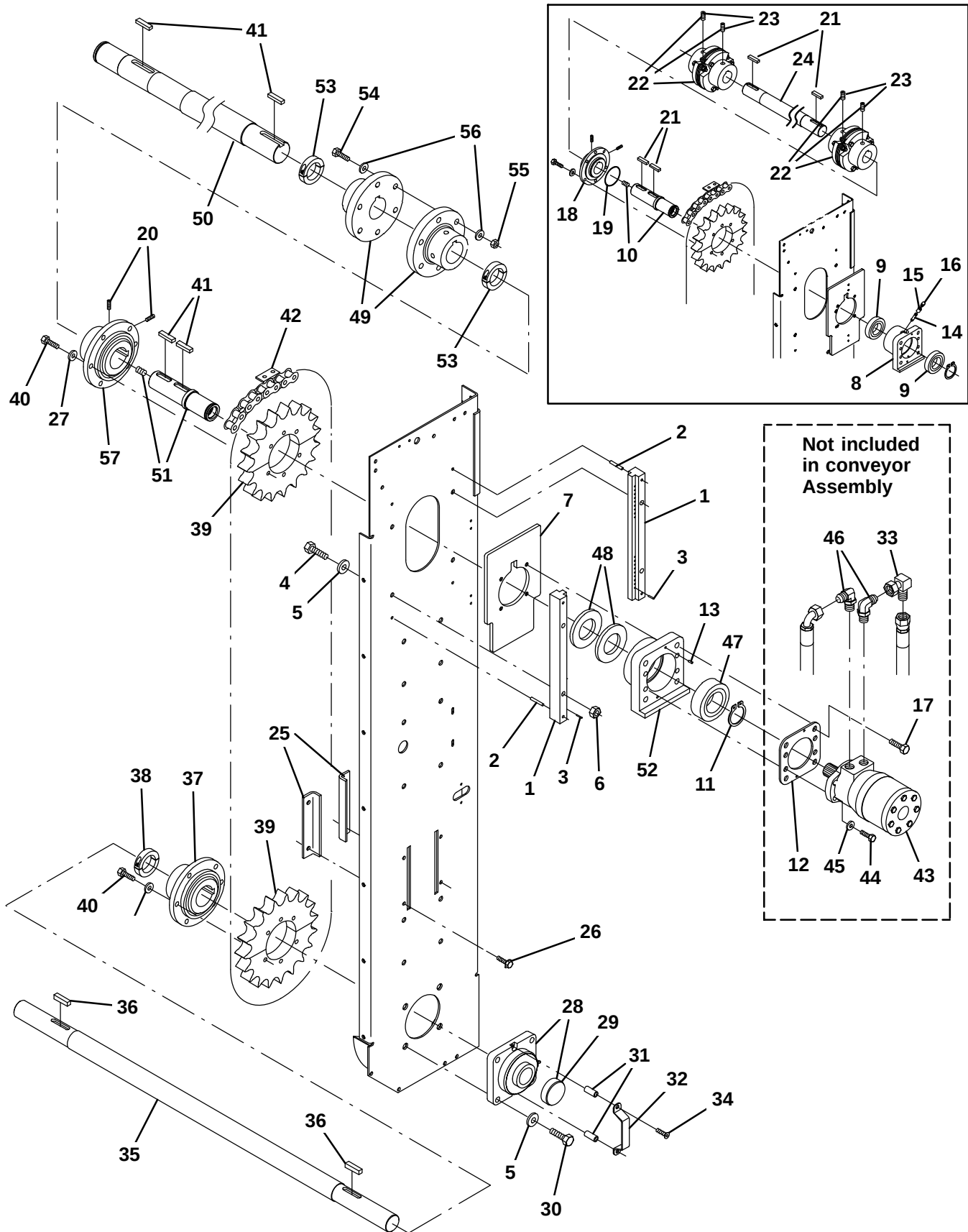
Fig. 29 – Conveyor Drive Group
