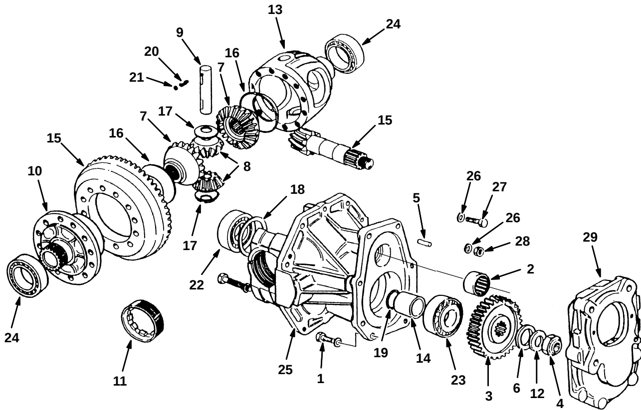
Fig. 8 – Axle Differential Breakdown, Front
