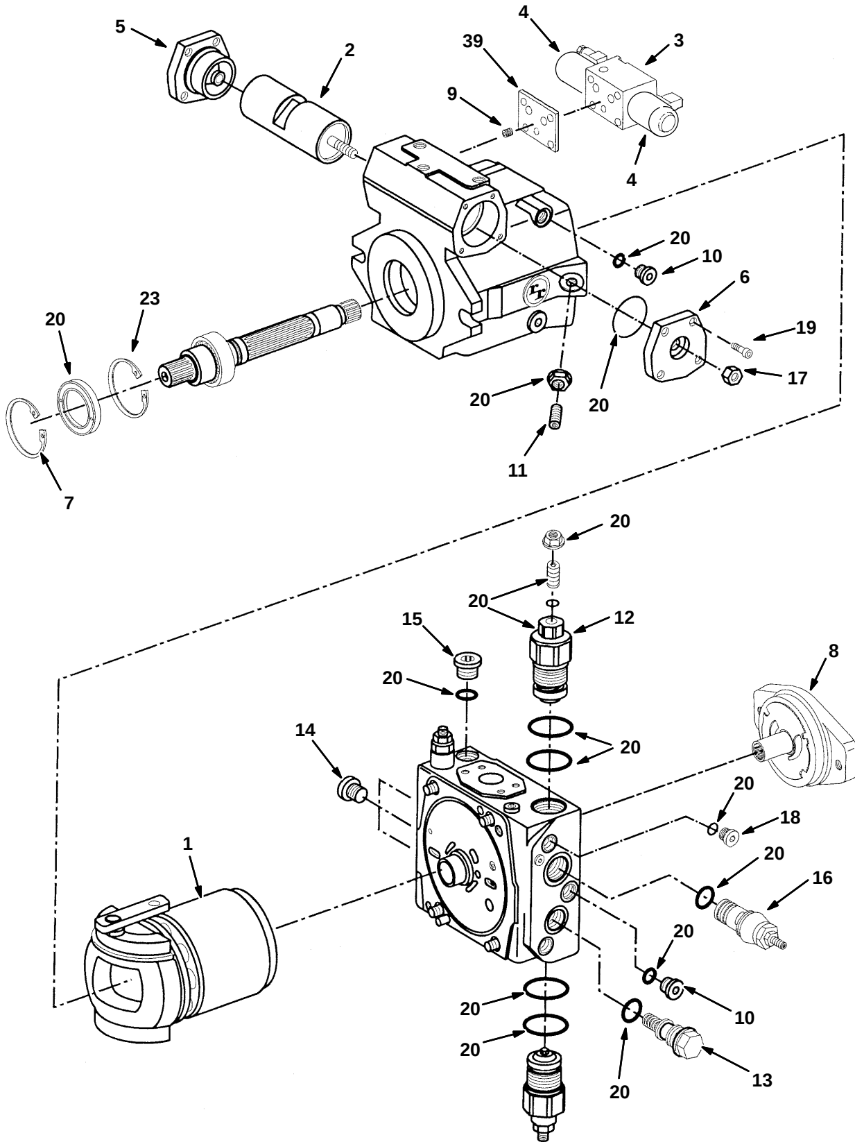
Fig. 2 – Hydraulic Piston Pump Breakdown, 1066392
