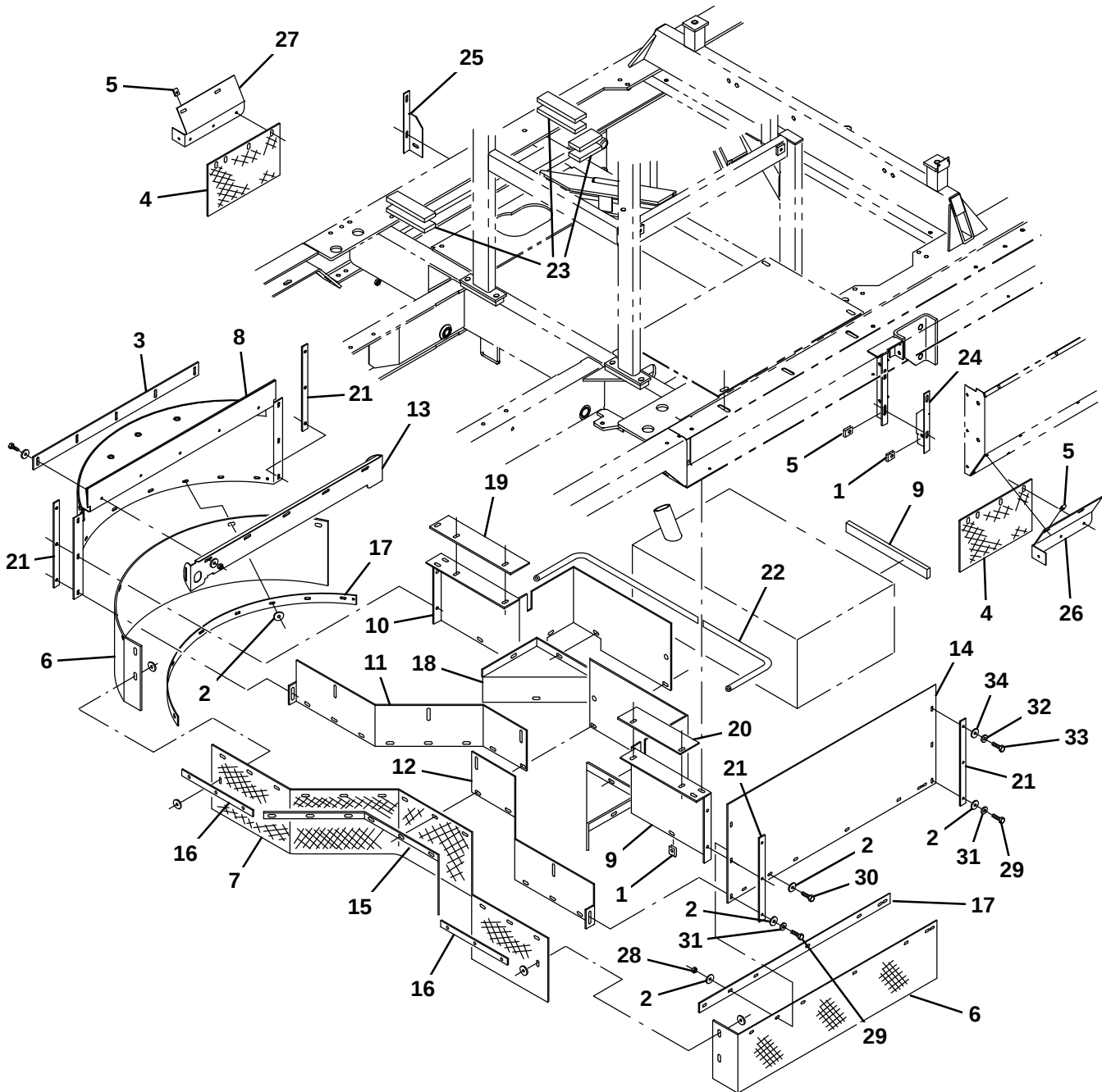
Fig. 73 – Dry Dust Control Group
