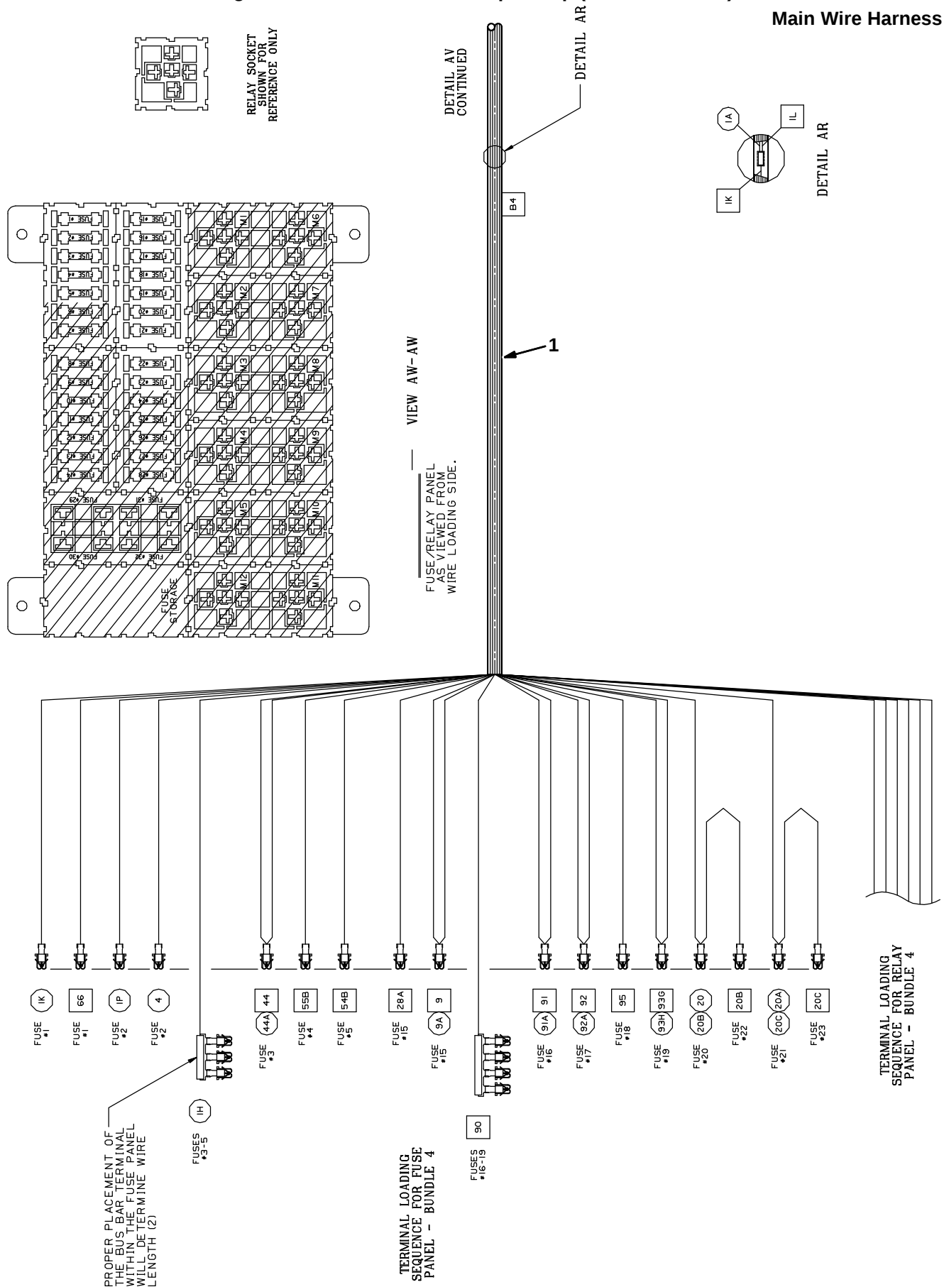
Fig. 77 – Wire Harnesses Group Group (000000–008499)
