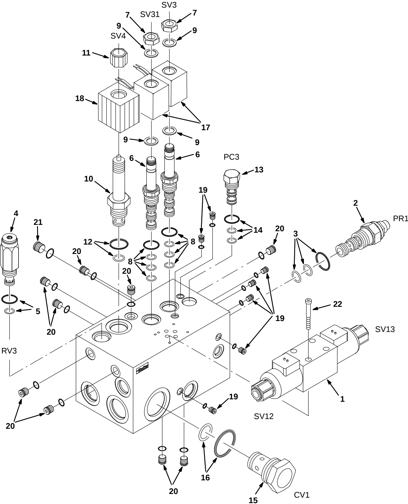
Fig. 21 – Hydraulic Solenoid Valve Breakdown, 771019
