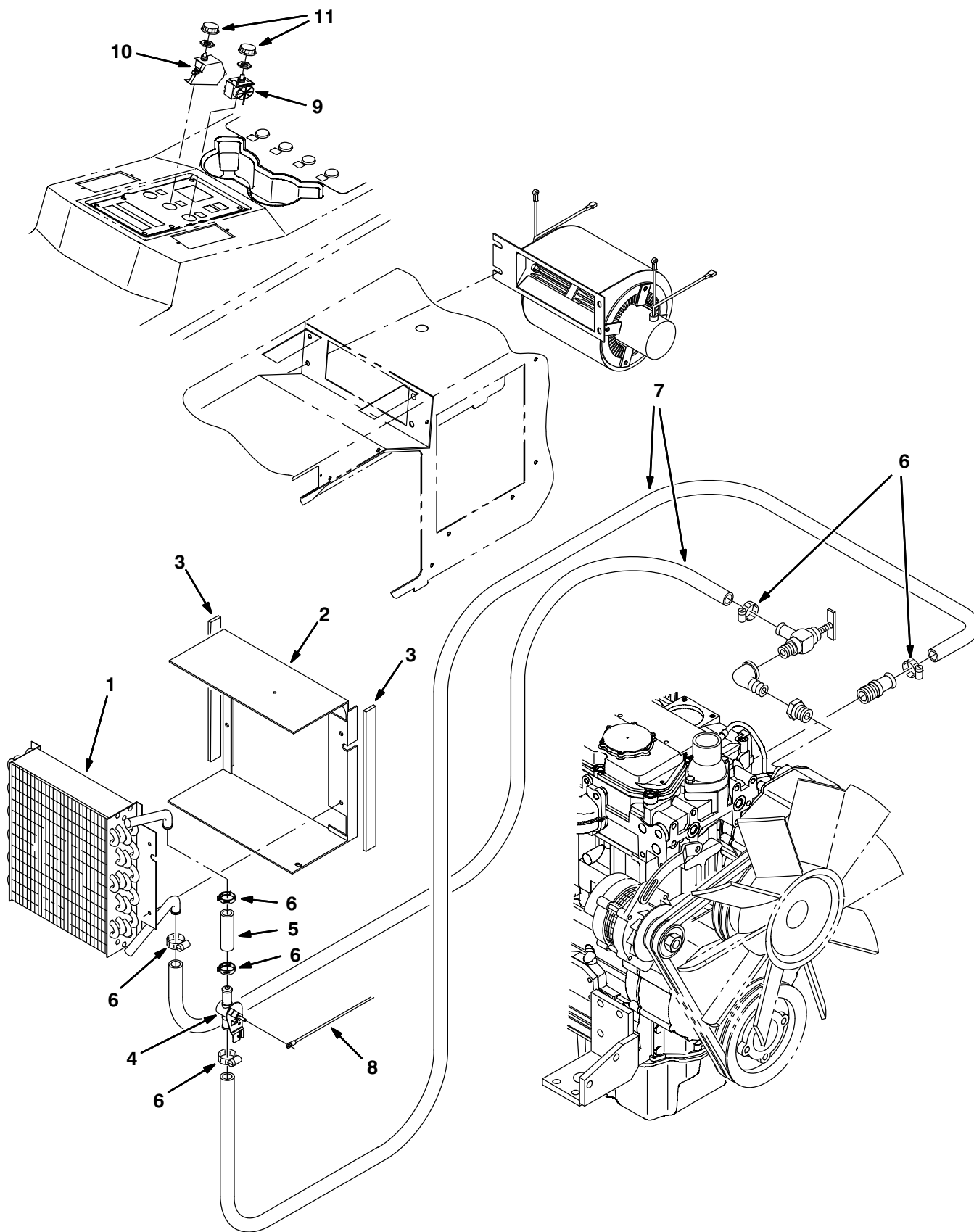
Fig. 49 – Cab Heater Group
