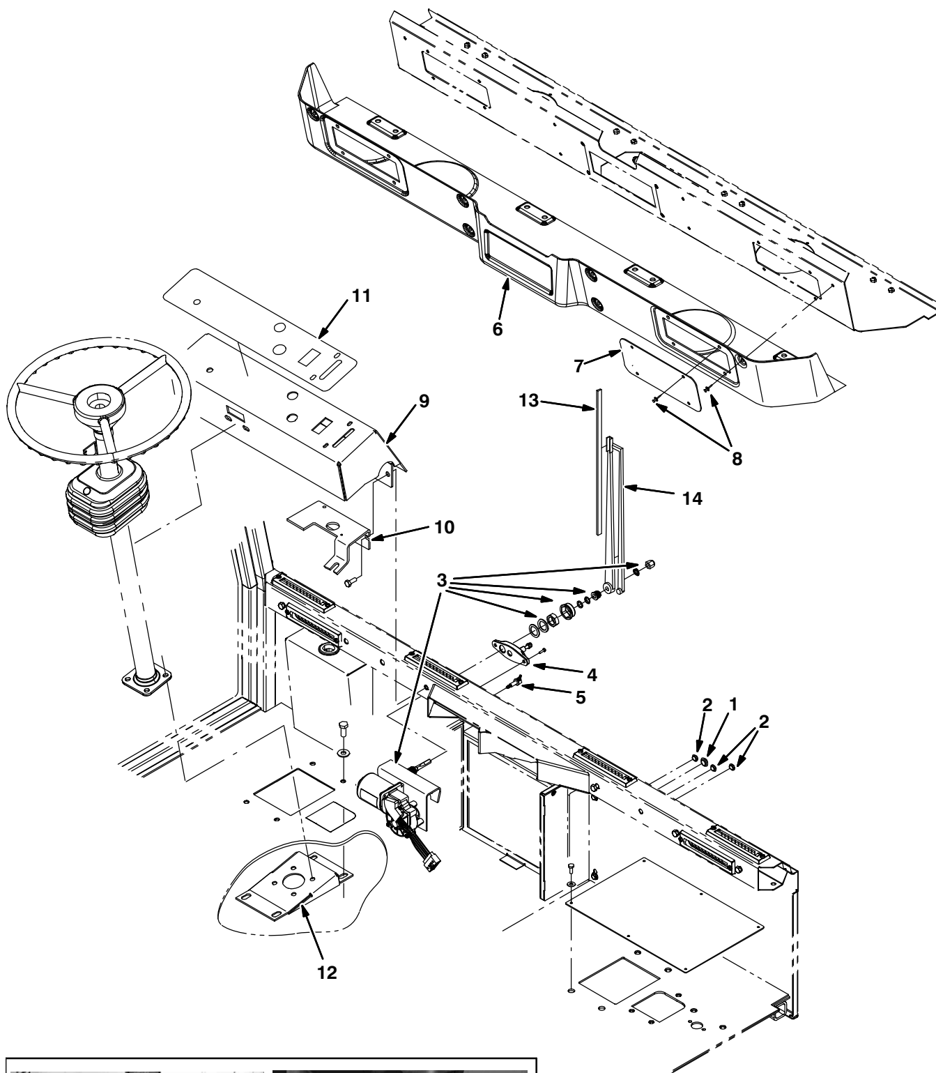
Fig. 19 – Left Hand Operator Group
