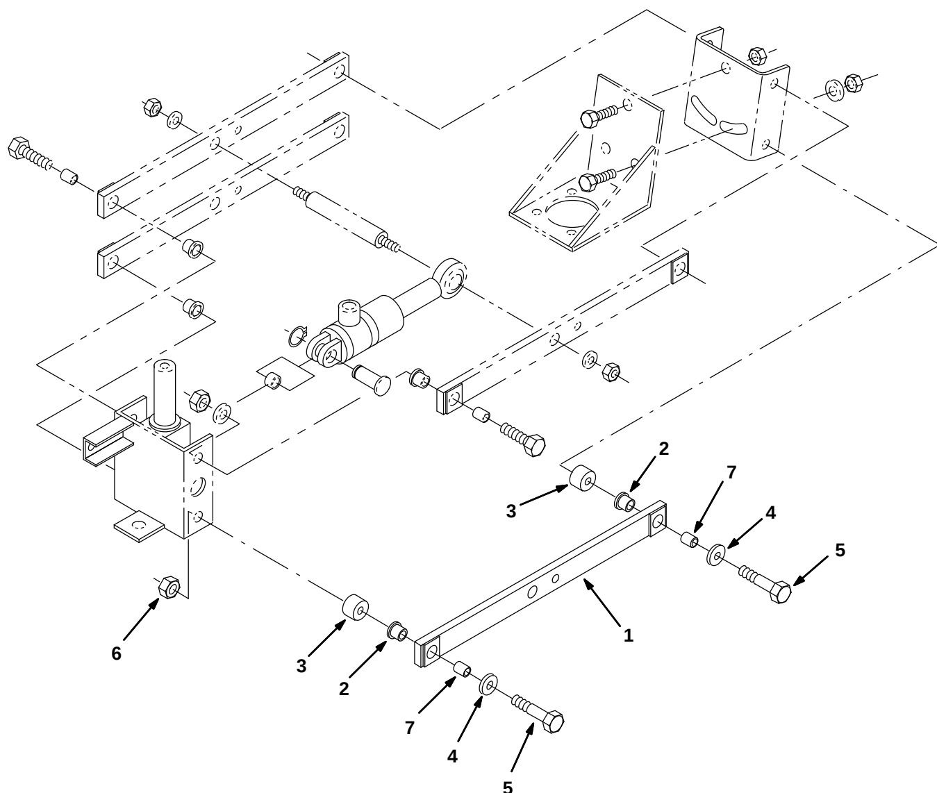
Fig. 44 – Side Brush Fourth Bar Linkage Kit (000000-009837)
