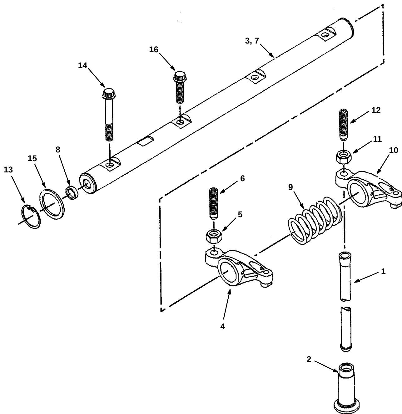
Fig. 26 – Valve Mechanism Group
