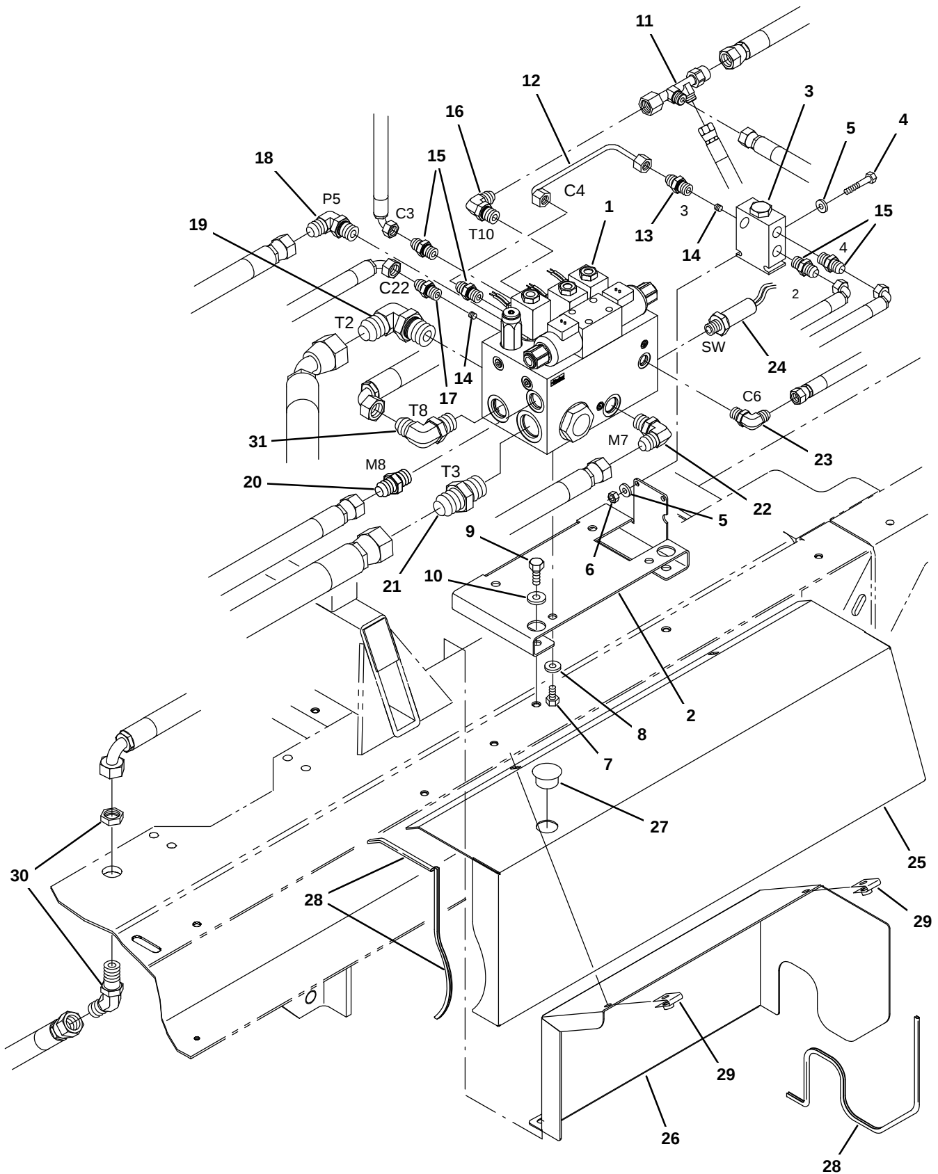
Fig. 66 – Hydraulic Main Brush/Conveyor Lift Valve Group (000000–008742)
