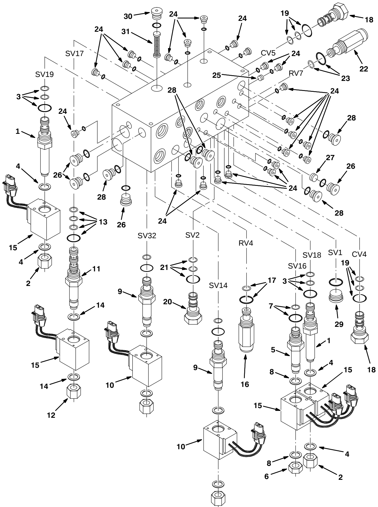
Fig. 14 – Hydraulic Solenoid Valve Breakdown, 768899
