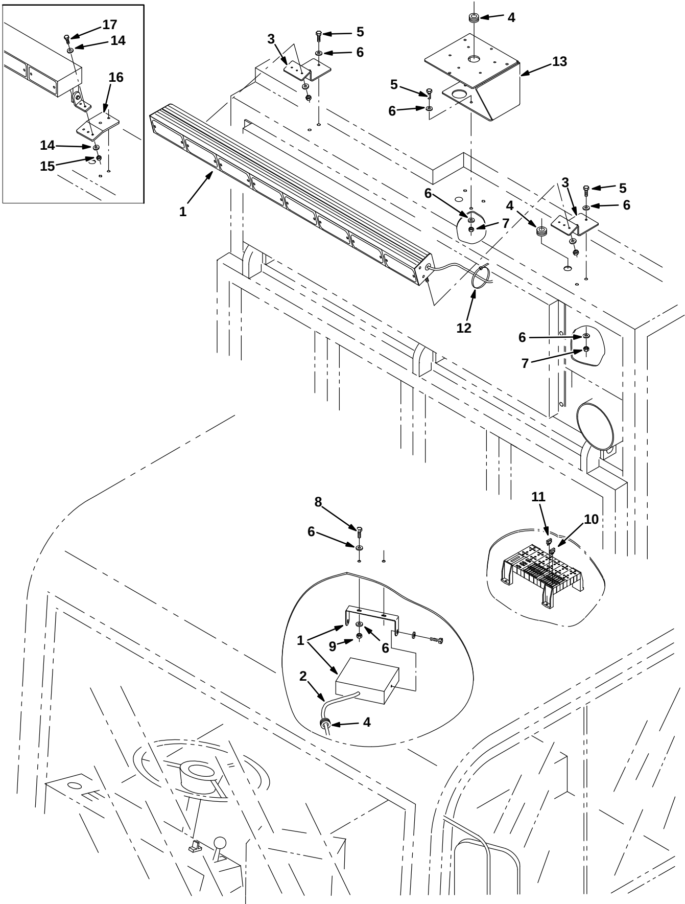
Fig. 38 – Light Kit, Arrow Stick, With Revolving Light
