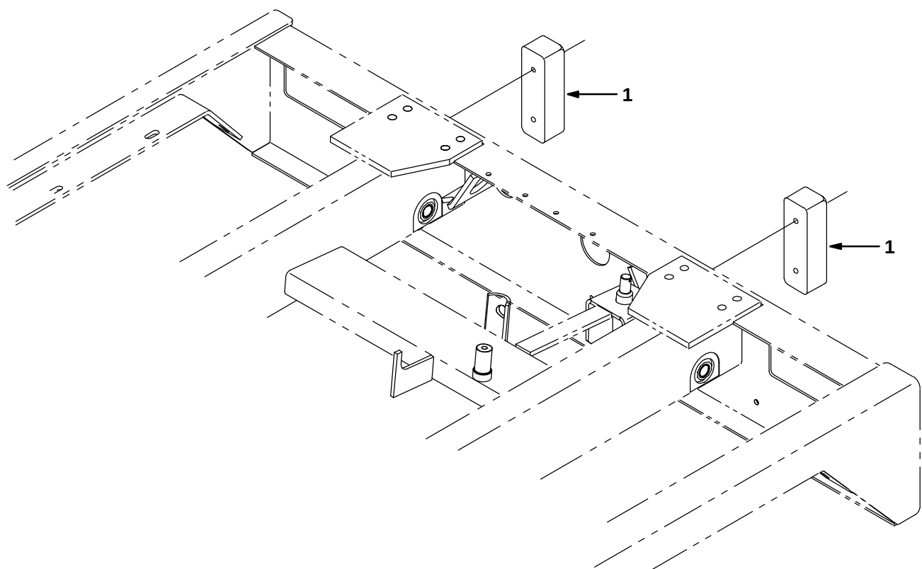
Fig. 28 – Rear Rubber Bumper Kit
