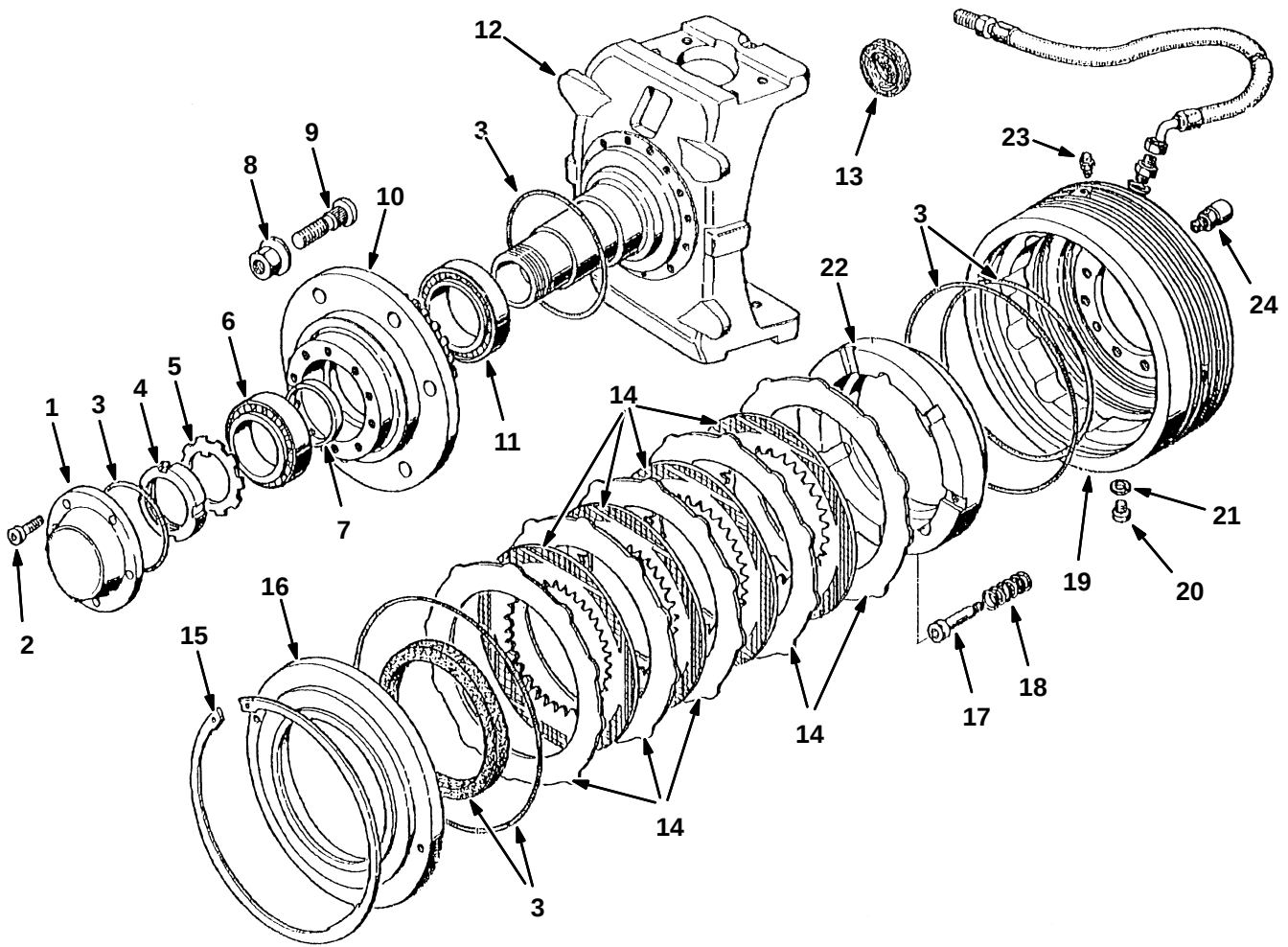
Fig. 12 – Axle Wheel Hub and Brake Breakdown, Rear
