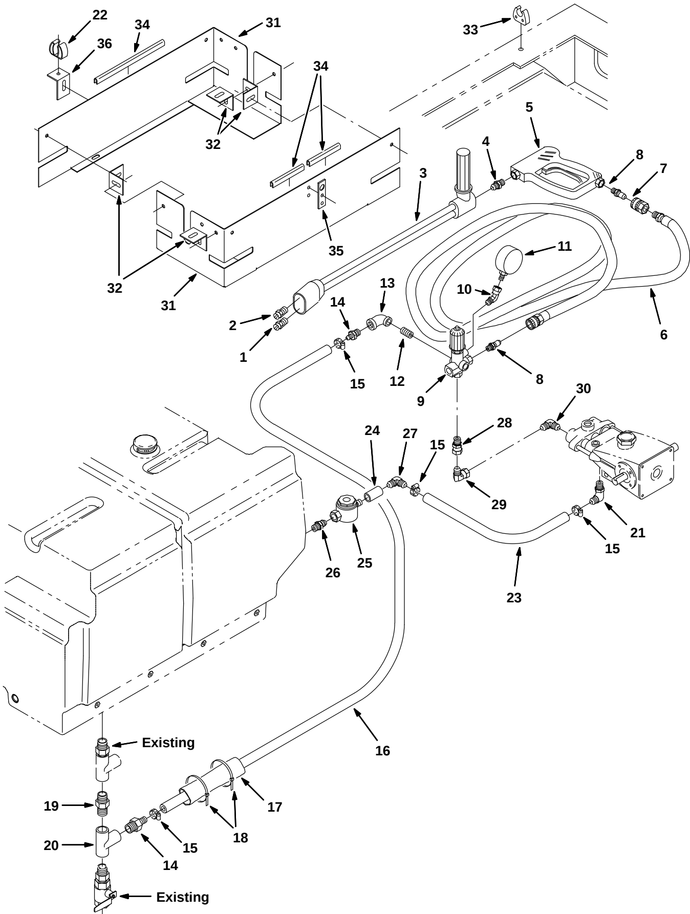
Fig. 15 – High Pressure Sprayer Wand Group
