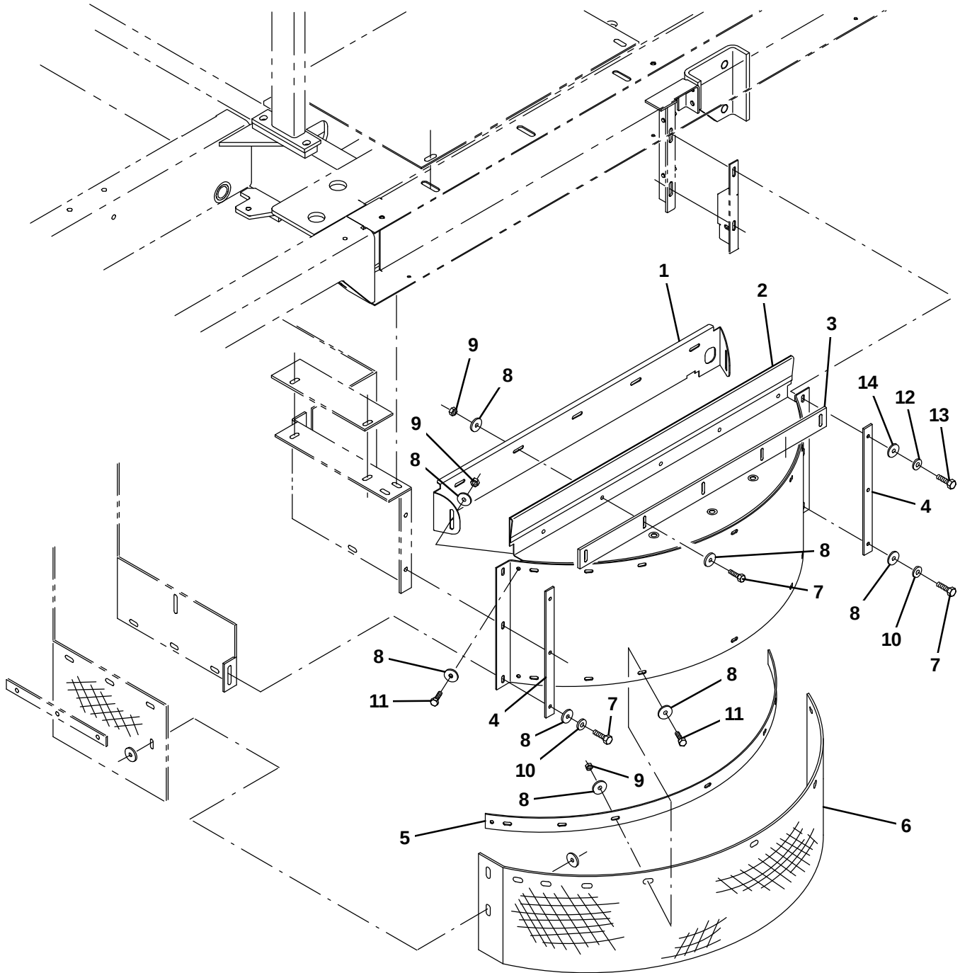
Fig. 74 – Dry Dust Control Group, Left Side Brush
