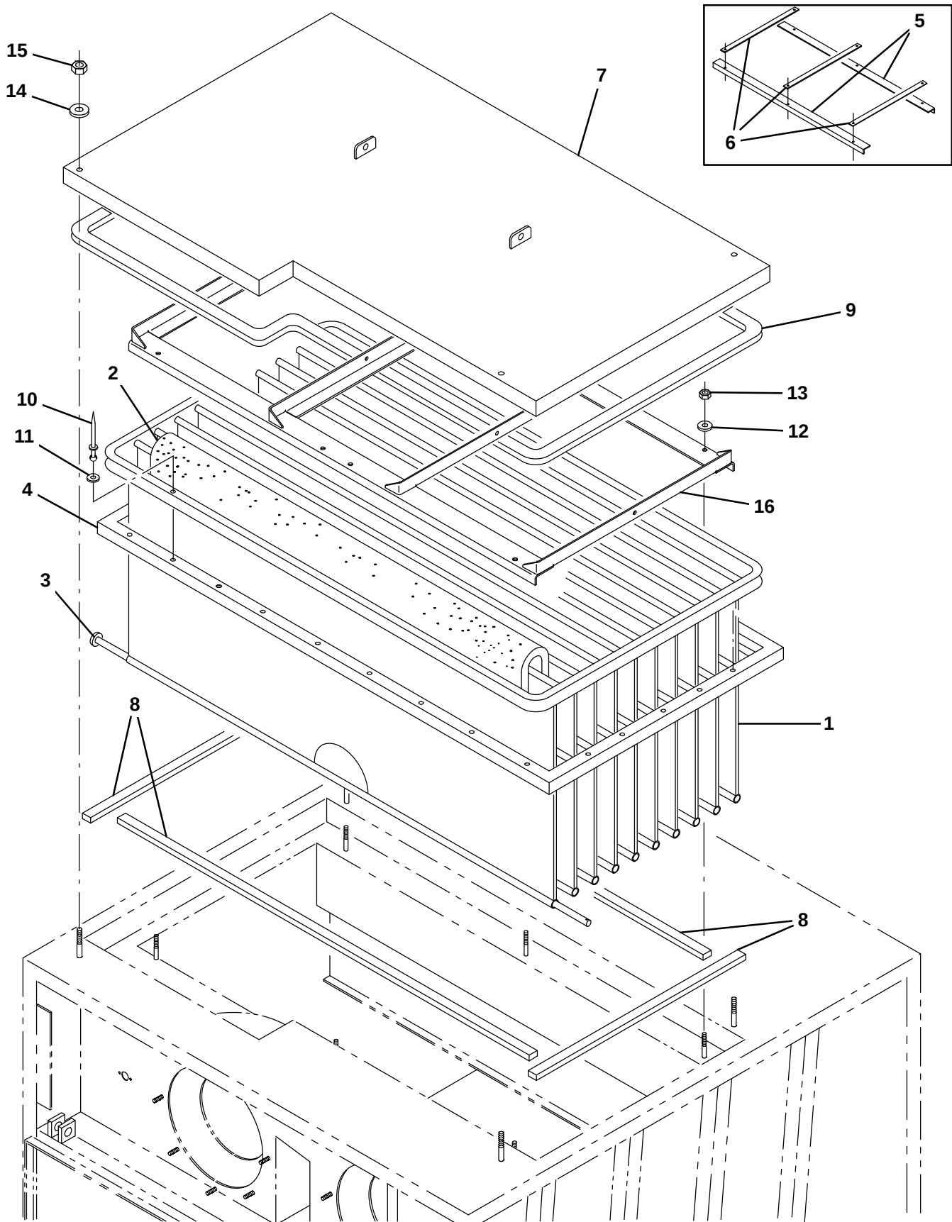
Fig. 35 – Hopper Filter Bags Group
