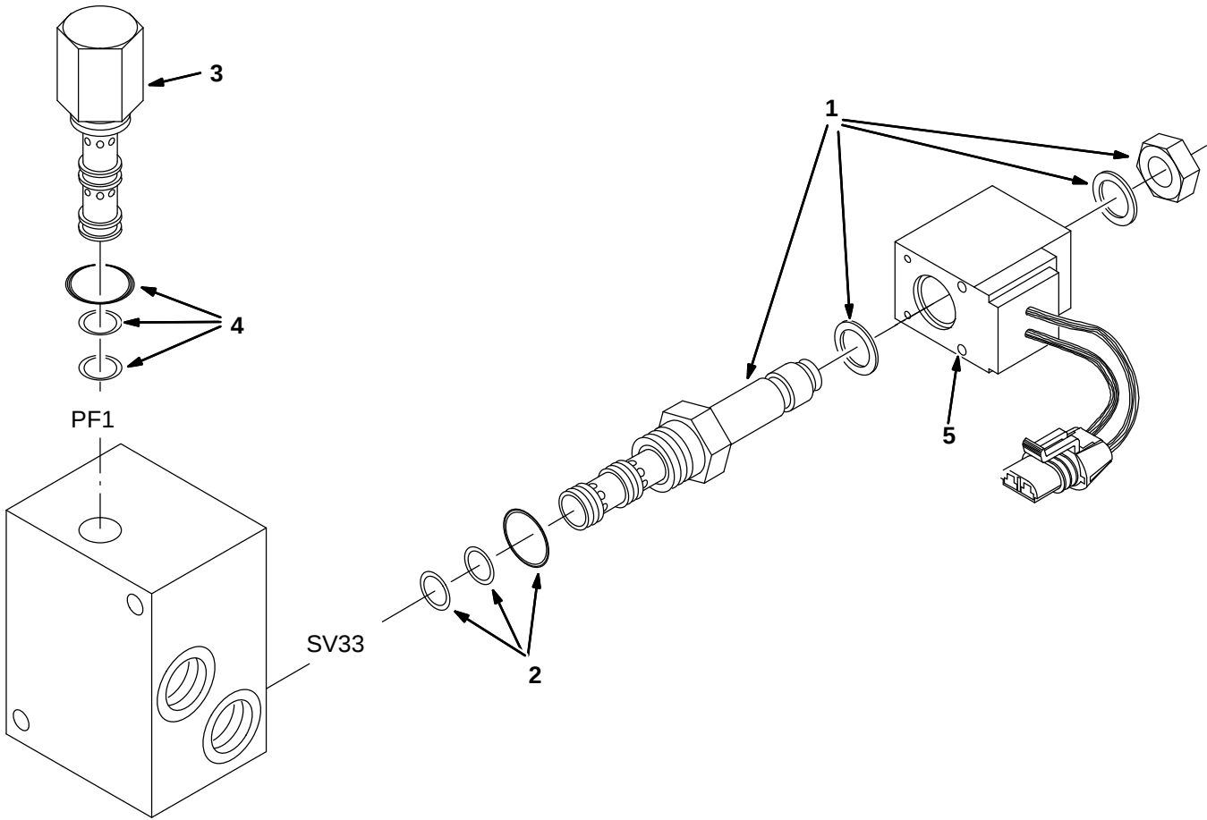
Fig. 17 – Hydraulic Solenoid Valve Breakdown, 1064633
