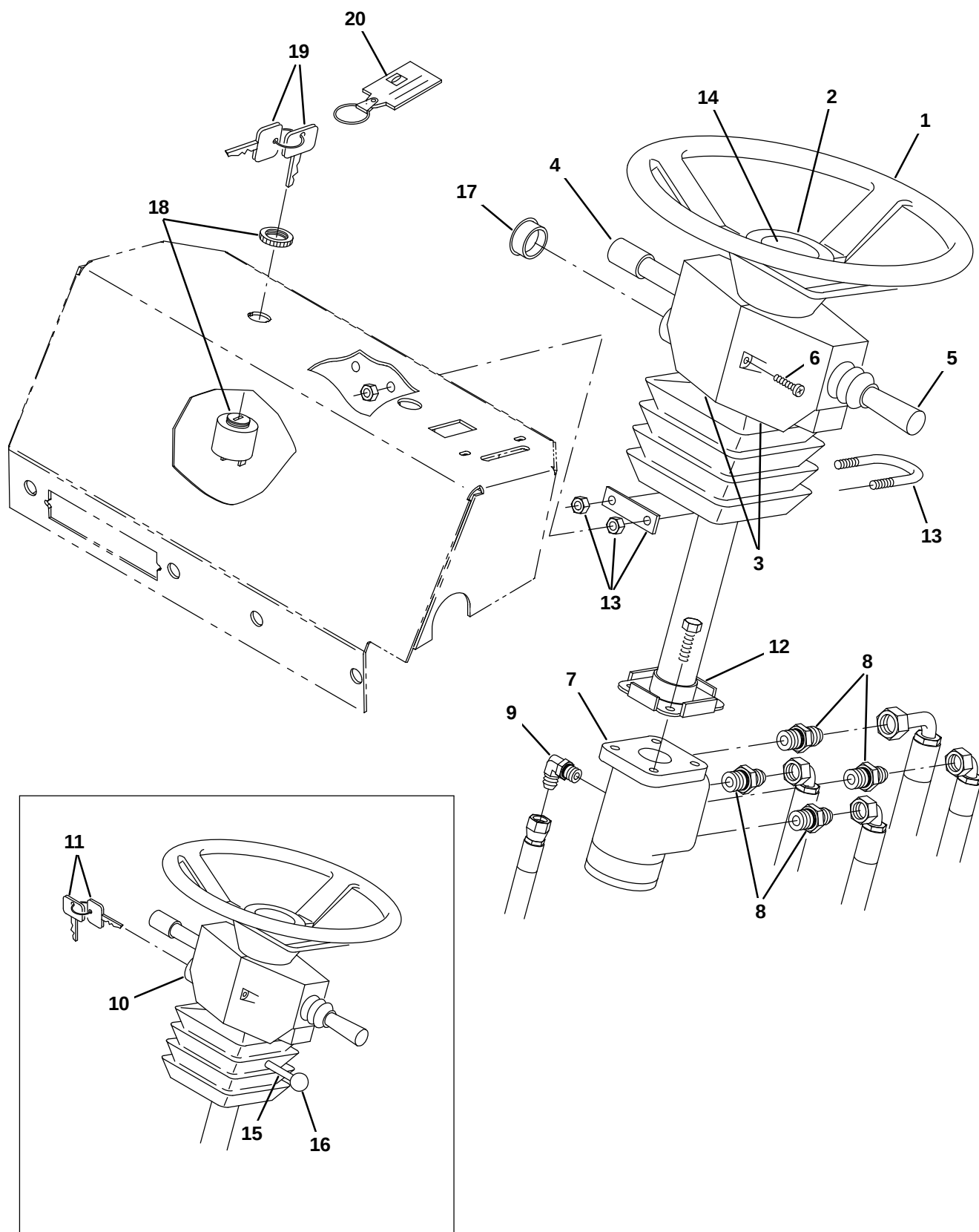
Fig. 52 – Steering Wheel Group
