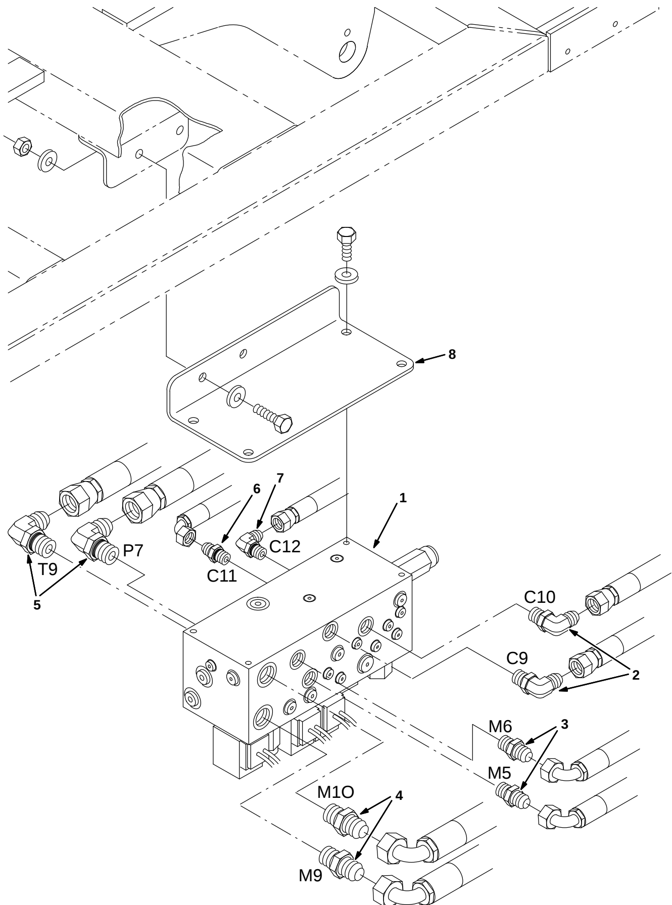
Fig. 68 – Hydraulic Hopper Control Valve Group
