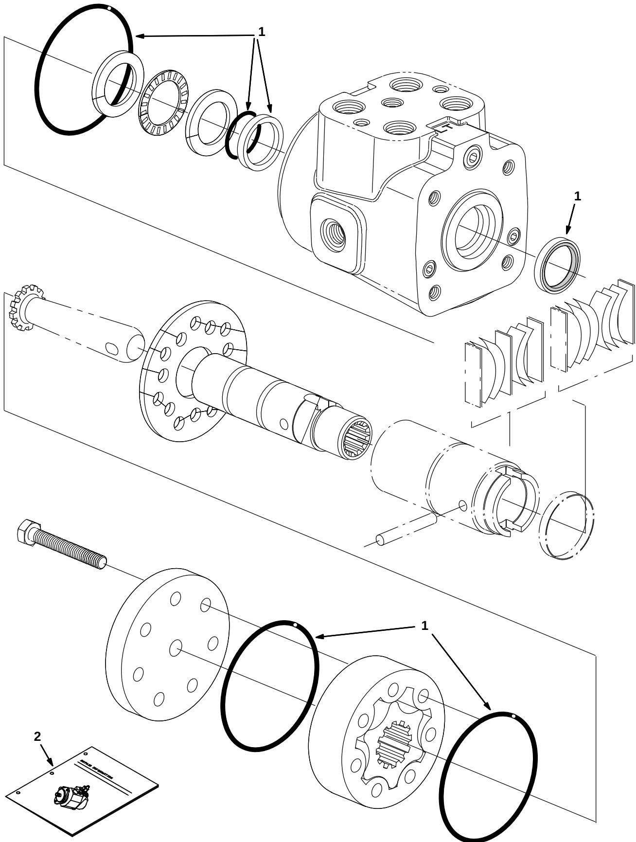
Fig. 18 – Hydraulic Steering Valve Breakdown, 771014
