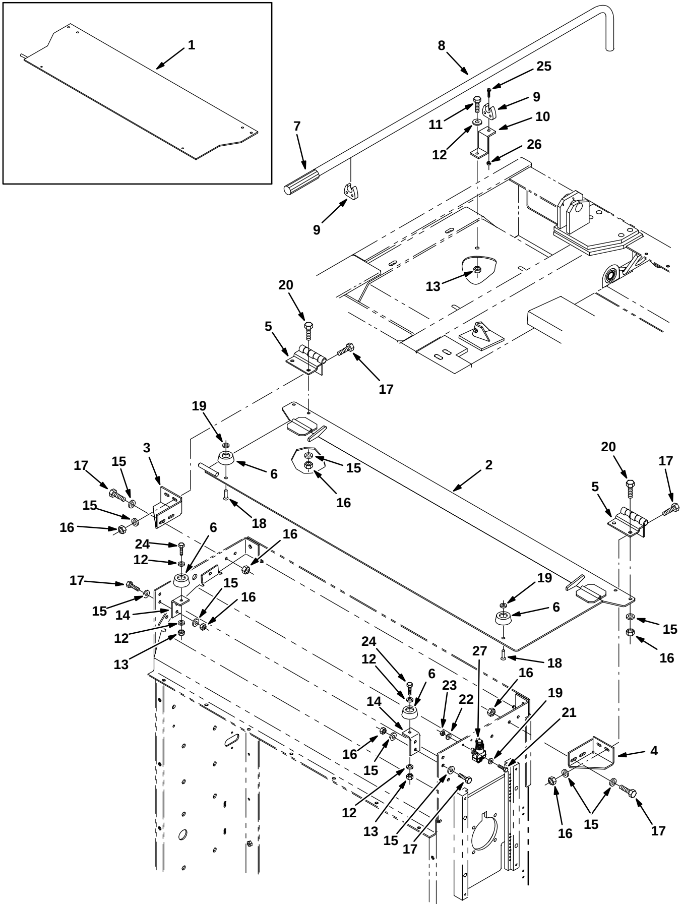
Fig. 23 – Vacuum Wand Door Group
