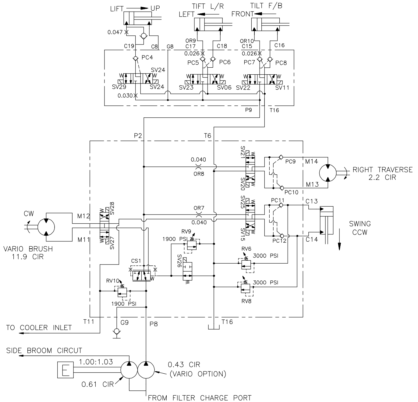
Fig. 55 – Hydraulic Schematic (000000-008742)
