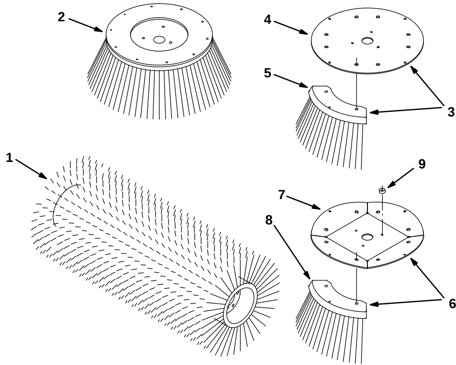
Fig. 2 – Brushes, Replacement
