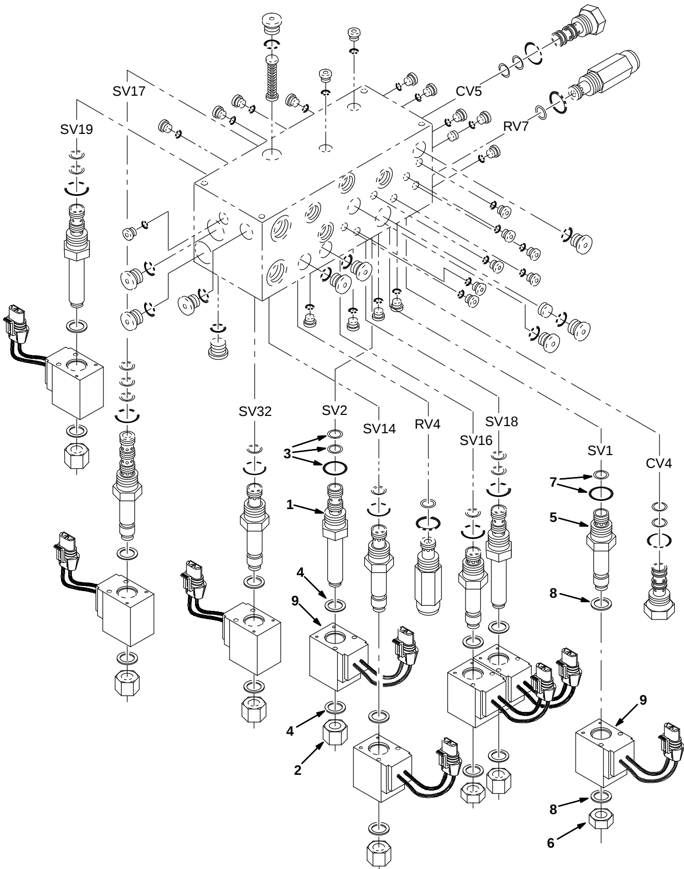
Fig. 15 – Hydraulic Solenoid Valve Breakdown, 768899 (For High Dump Hopper Lift Option)
