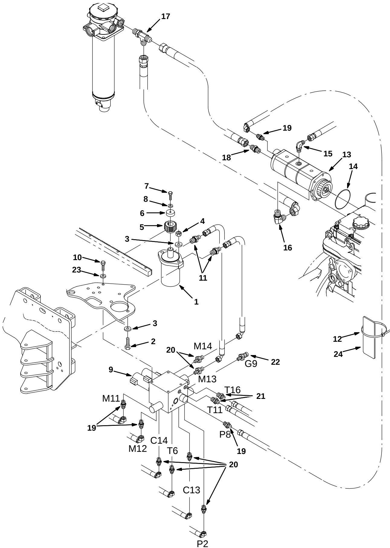
Fig. 8 – Vario Brush Dolly Hydraulics Group
