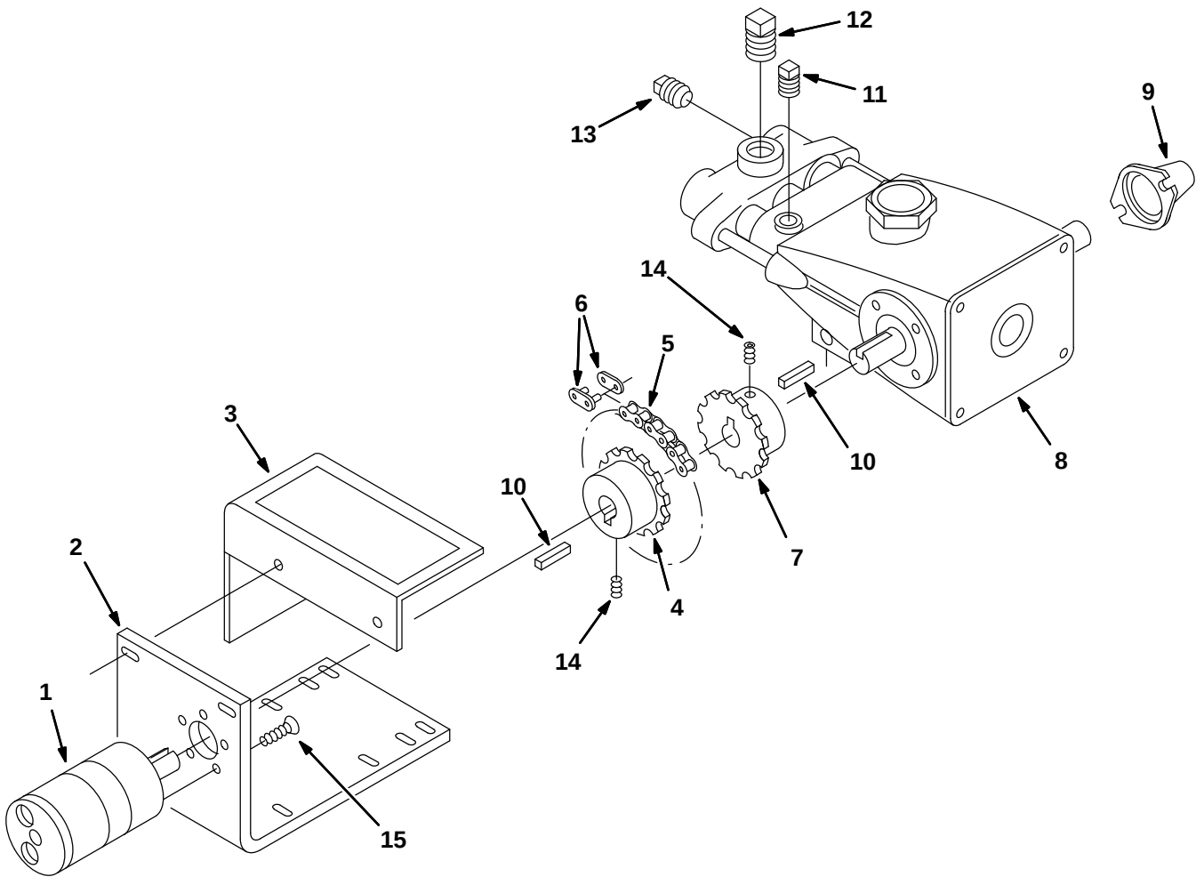
Fig. 16 – High Pressure Sprayer Pump Group
