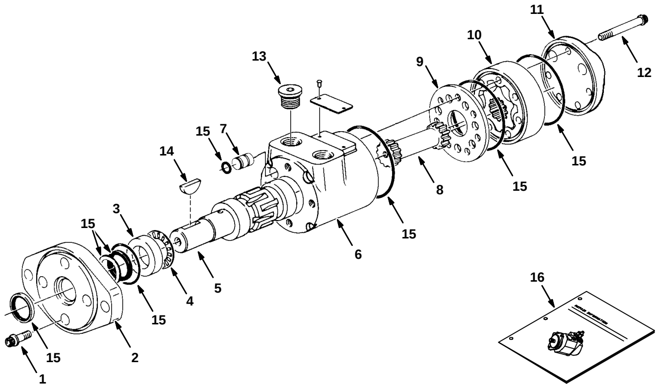
Fig. 4 – Hydraulic Motor Breakdown, 762035
