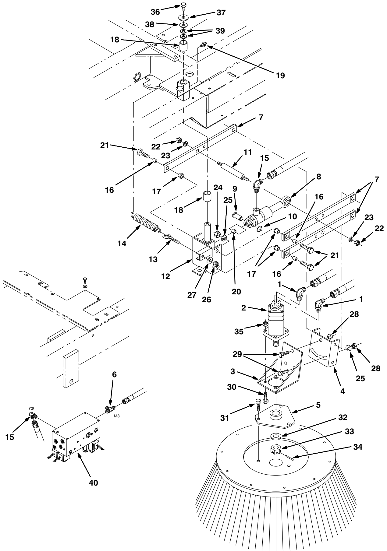
Fig. 4 – Left Side Brush Group (000000-009837)
