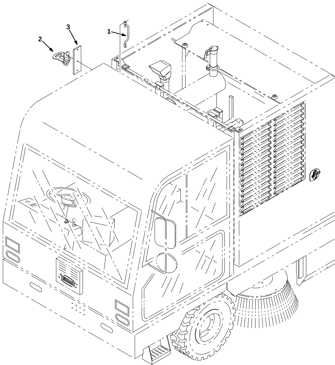
Fig. 33 – Engine Access Step Kit
