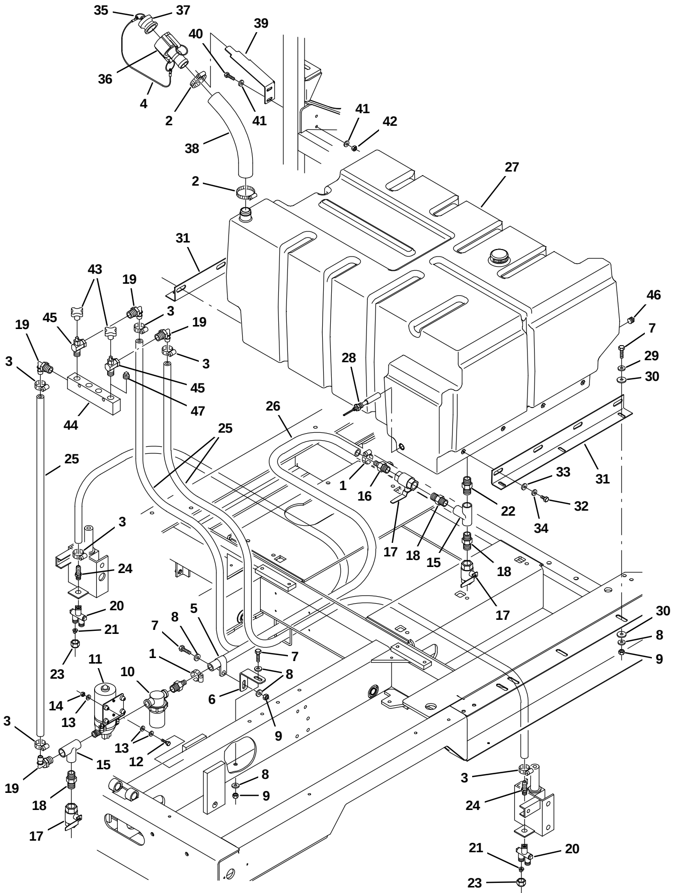
Fig. 71 – Water Tank Group
