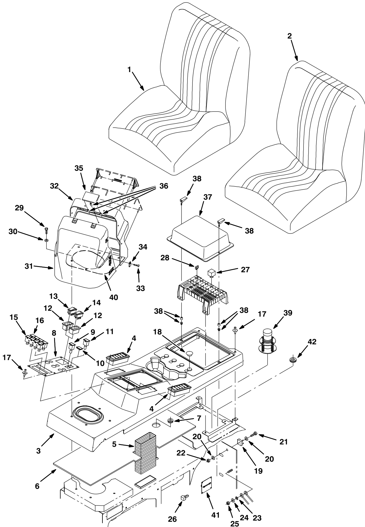
Fig. 47 – Cab Center Console and Seat Group
