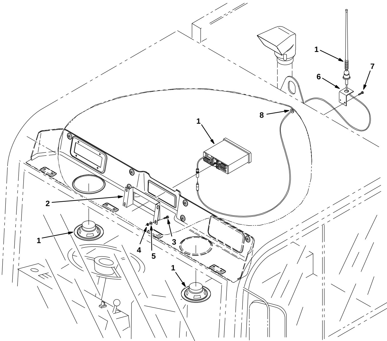
Fig. 40 – Radio Kit
