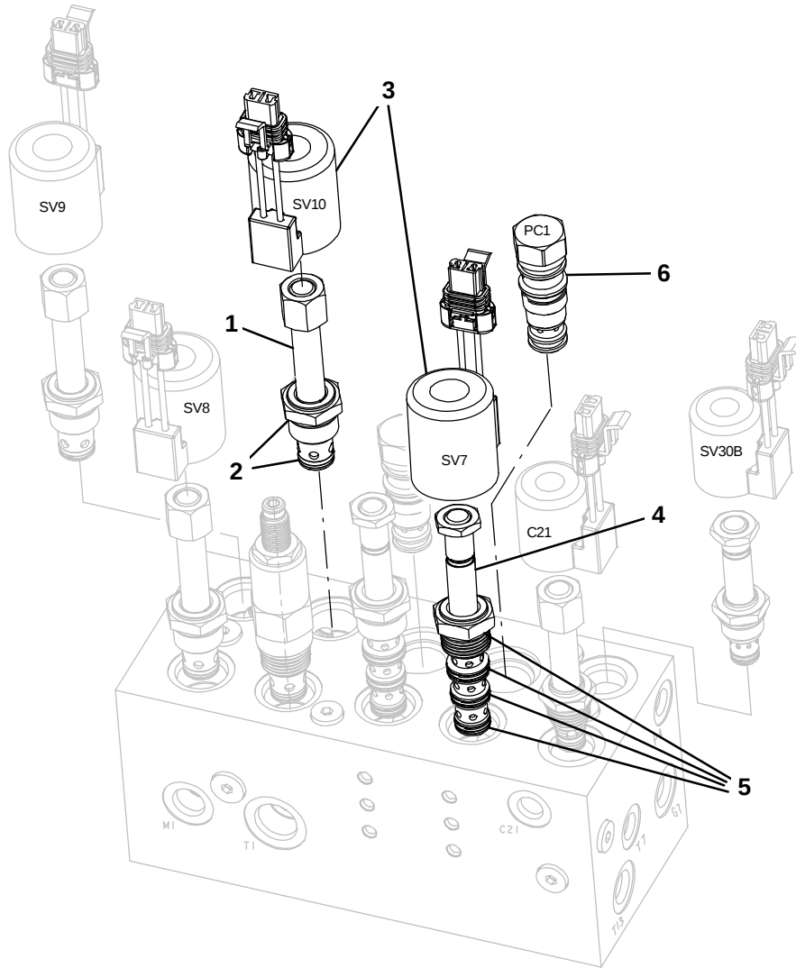
Fig. 28 – Hydraulic Solenoid Valve Breakdown, 1048792 (For Left Hand Side Brush Option)
