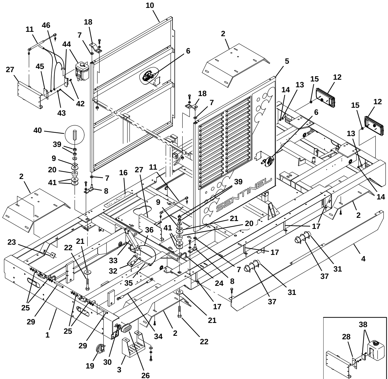
Fig. 4 – Main Frame Group (008500– )
