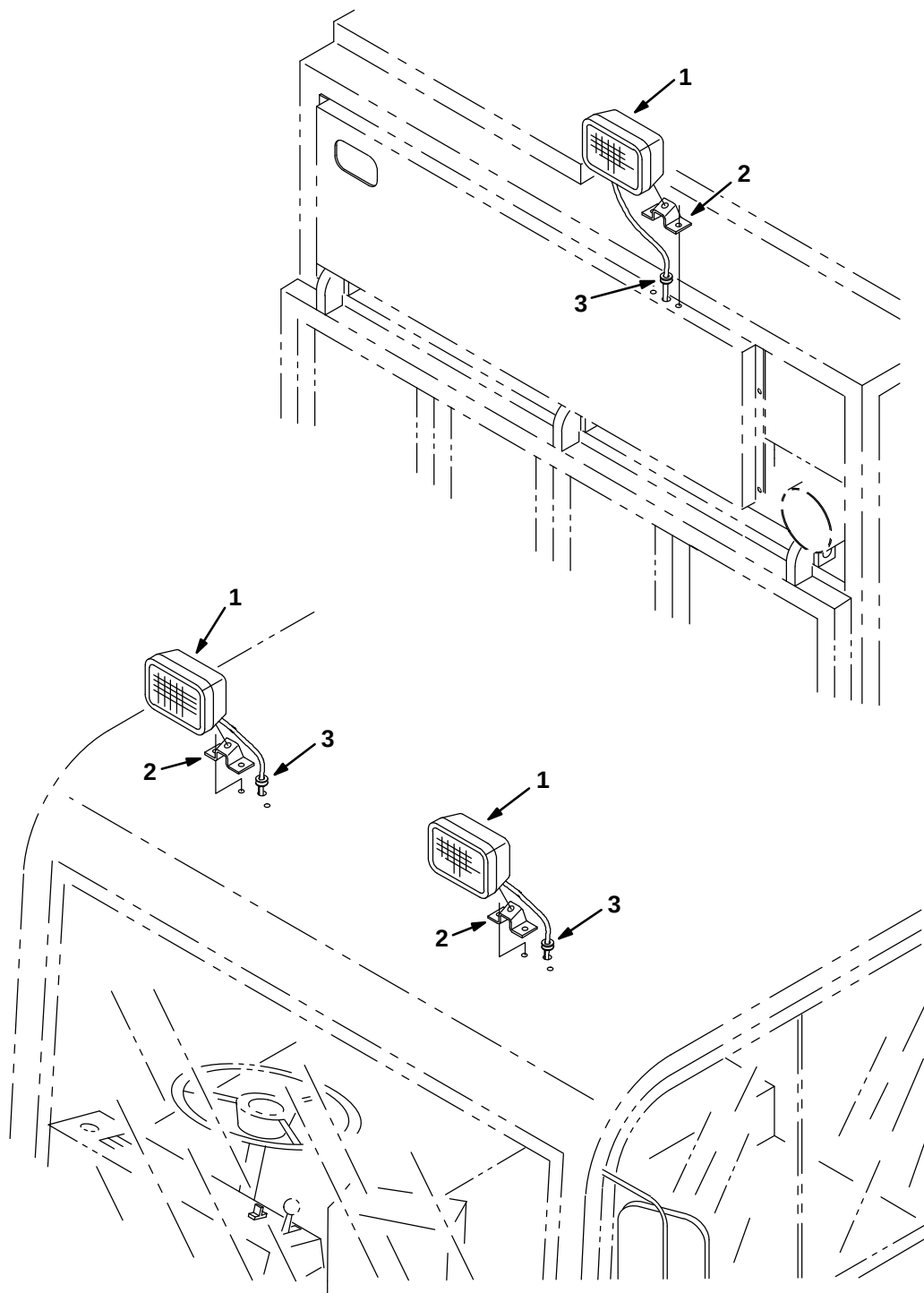
Fig. 34 – Light Kit, Night
