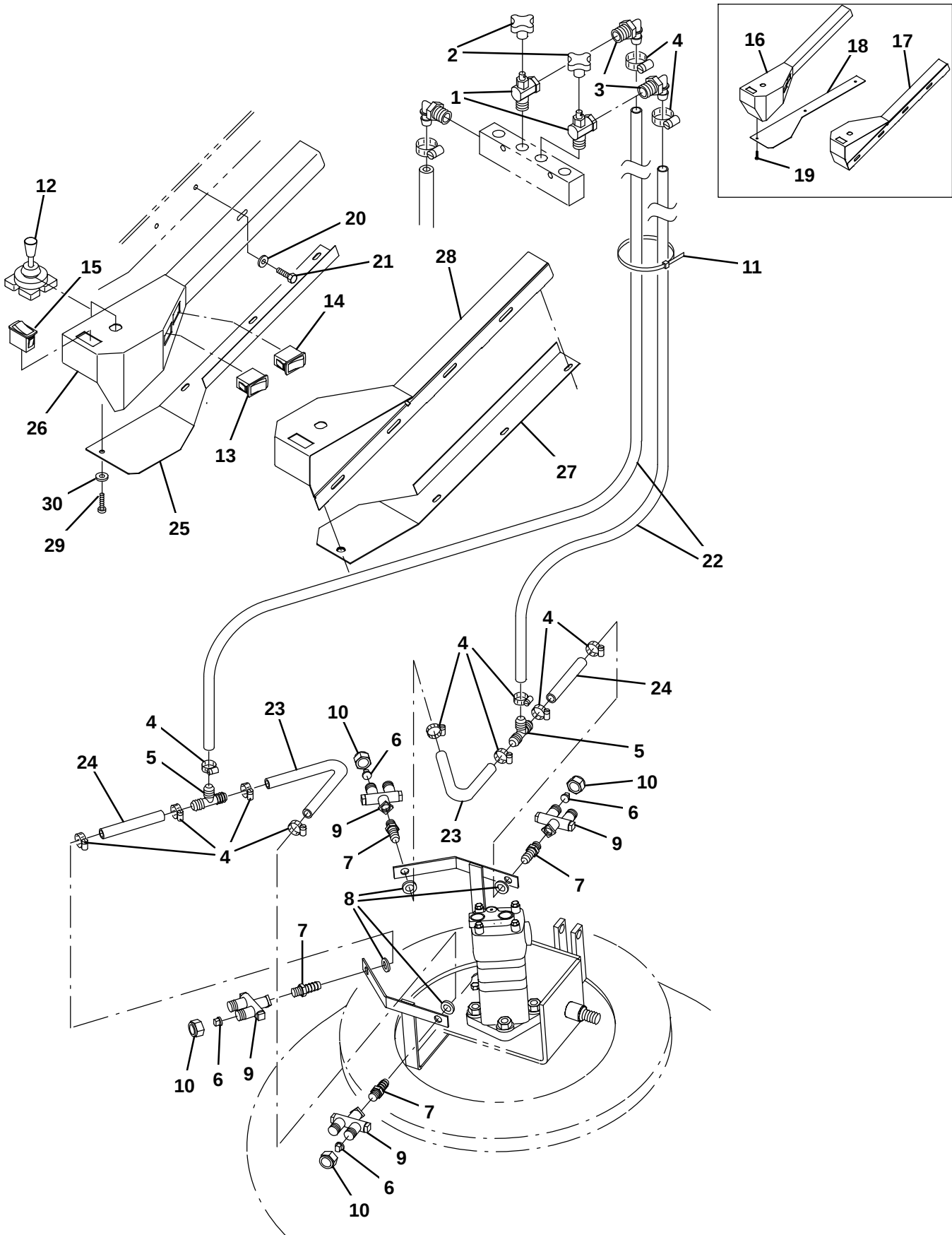
Fig. 12 – Vario Brush Cab Controls and Water Supply Group
