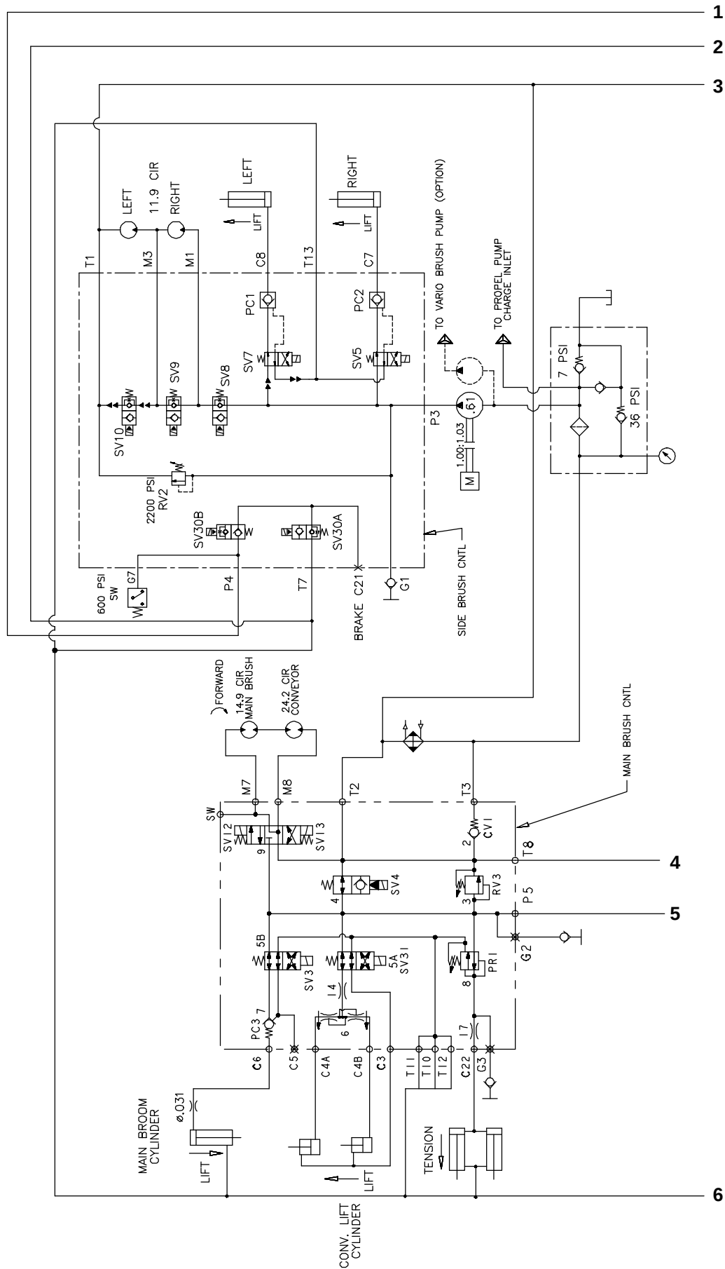
Fig. 56 – Hydraulic Schematic (008743– )
