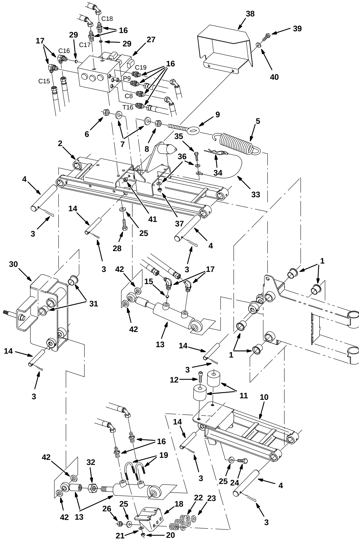
Fig. 10 – Vario Brush Lift Group
