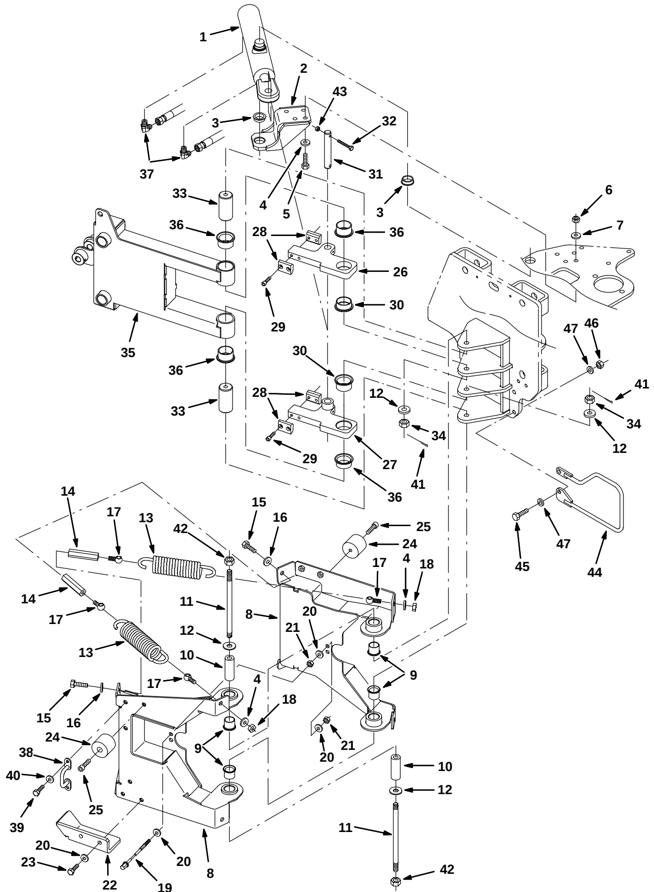
Fig. 9 – Vario Brush Pivot Group
