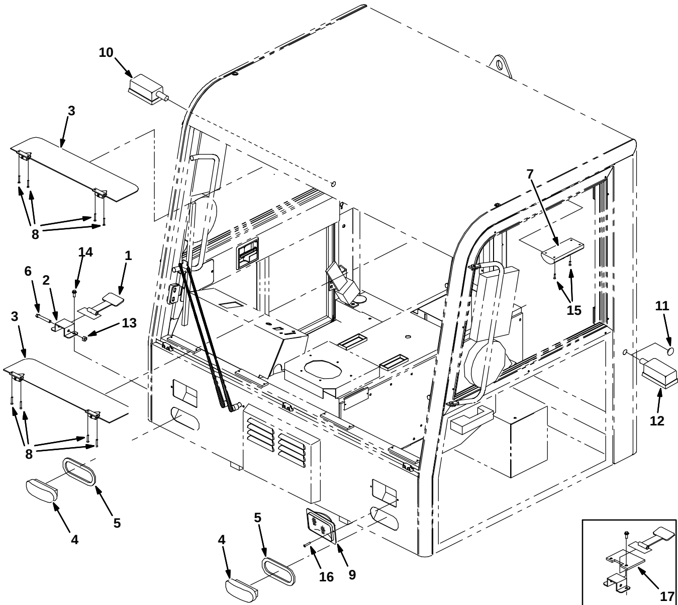
Fig. 48 – Cab Lights, Visor, and Pedal Group
