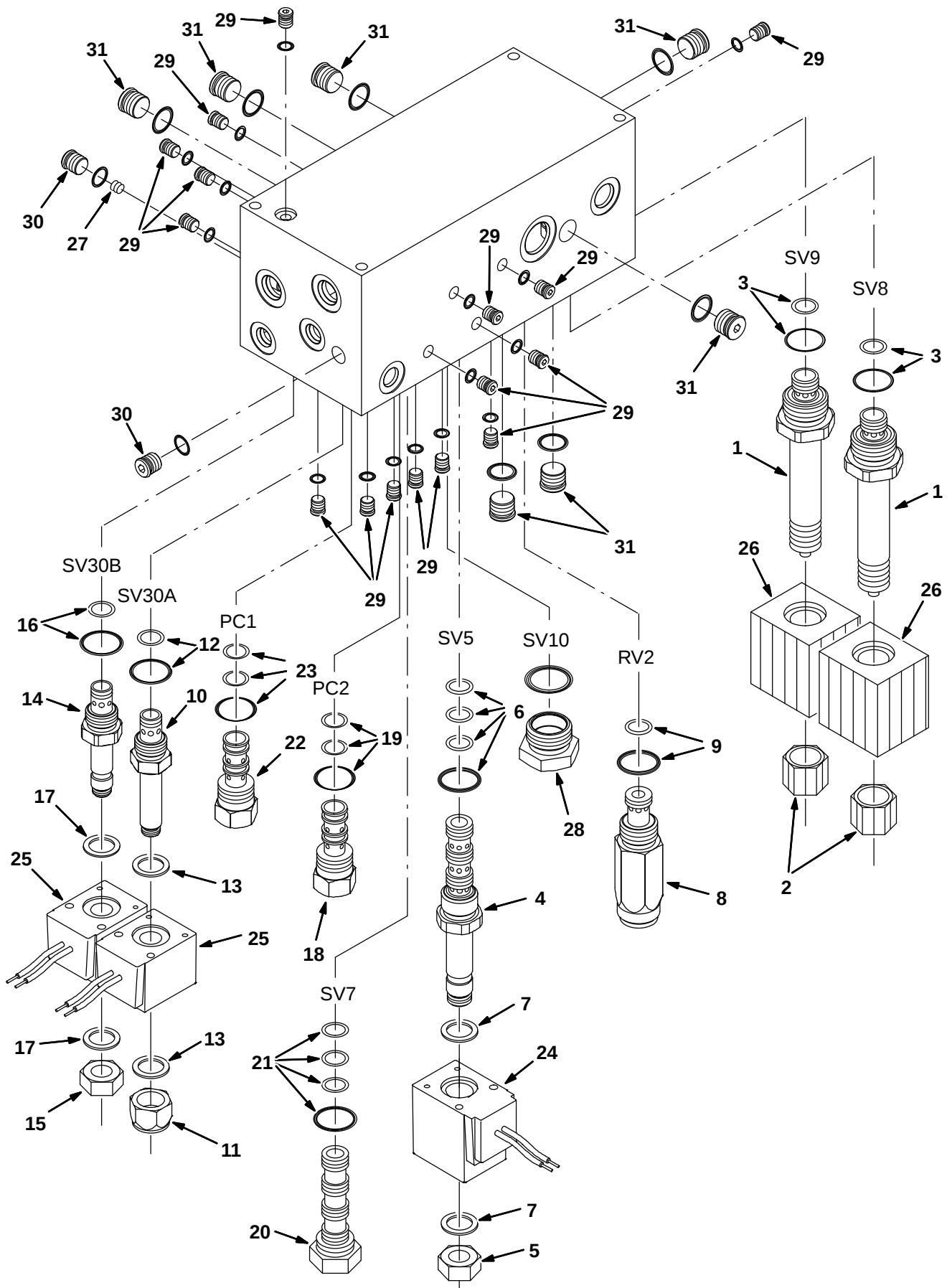
Fig. 19 - Hydraulic Solenoid Valve Breakdown, 771010
