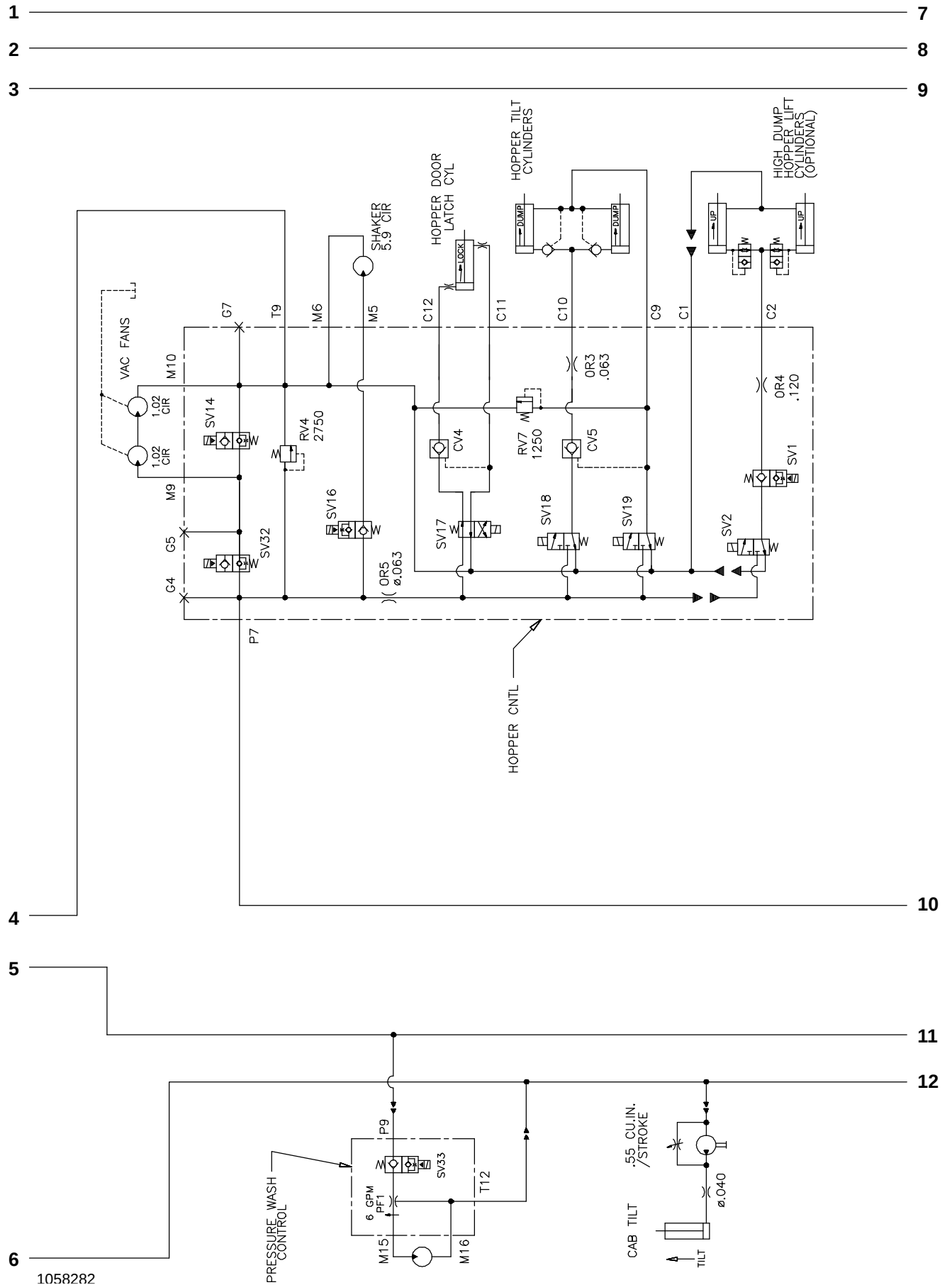
Fig. 56 – Hydraulic Schematic (008743– )
