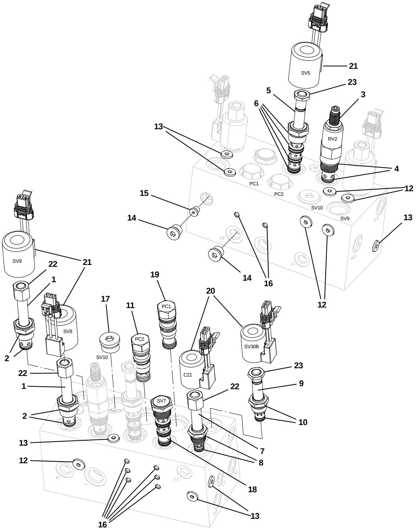
Fig. 27 – Hydraulic Solenoid Valve Breakdown, 1048792
