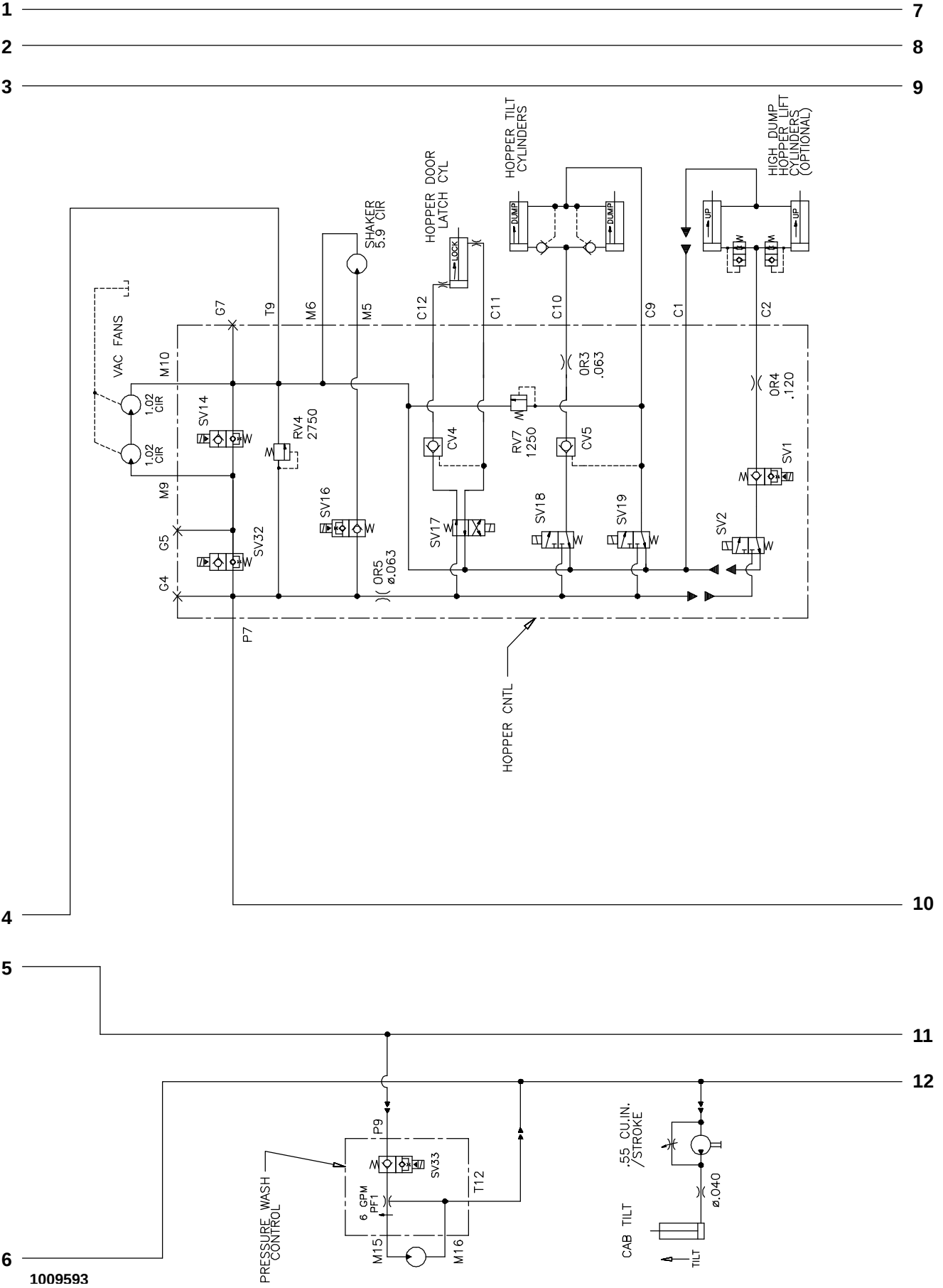
Fig. 55 – Hydraulic Schematic (000000-008742)
