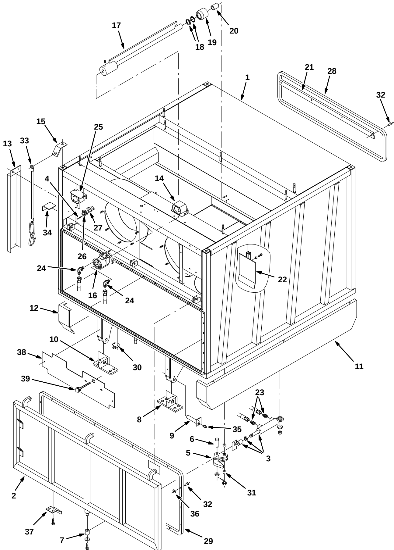
Fig. 34 – Hopper Group
