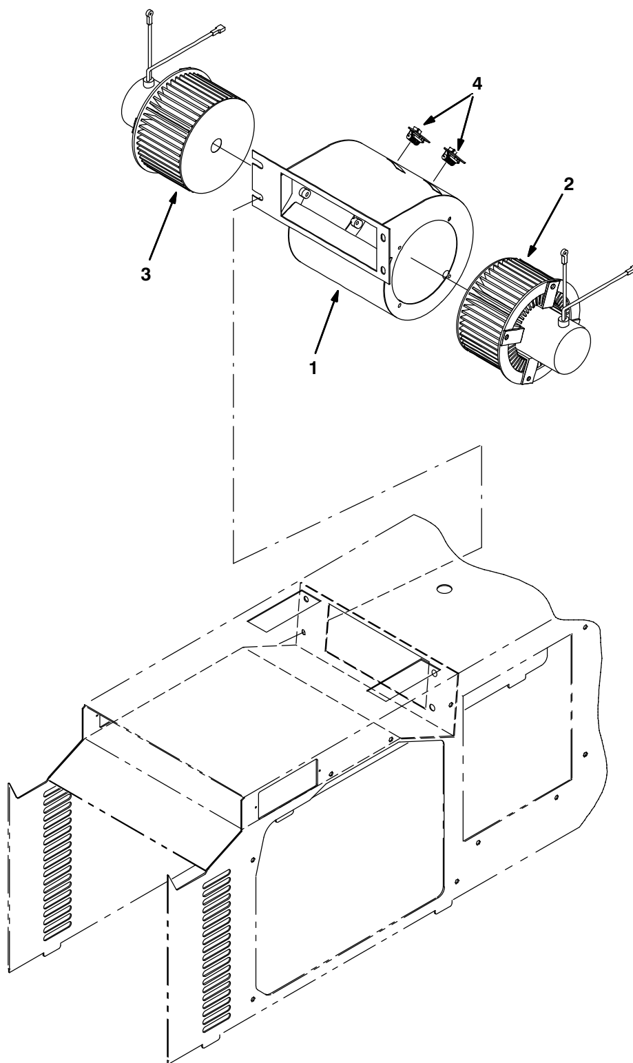
Fig. 50 – Cab Blower Assembly
