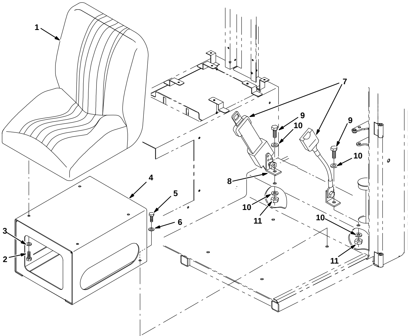
Fig. 39 – Passenger Seat Kit
