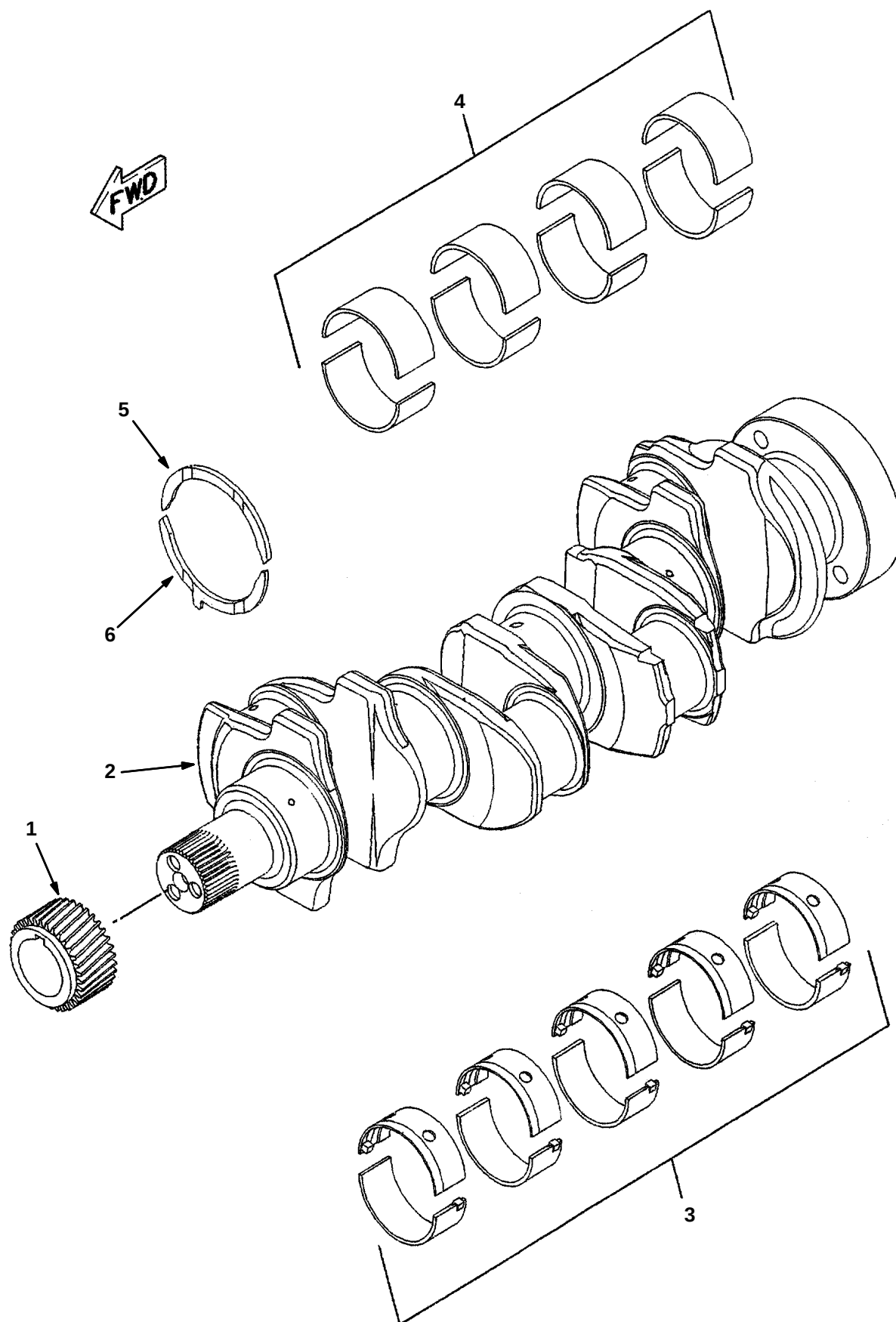
Fig. 17 – Crankshaft Group
