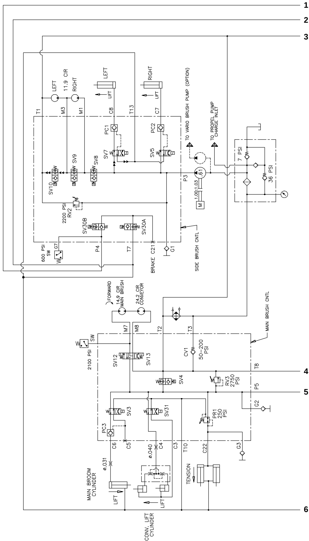
Fig. 55 – Hydraulic Schematic (000000-008742)
