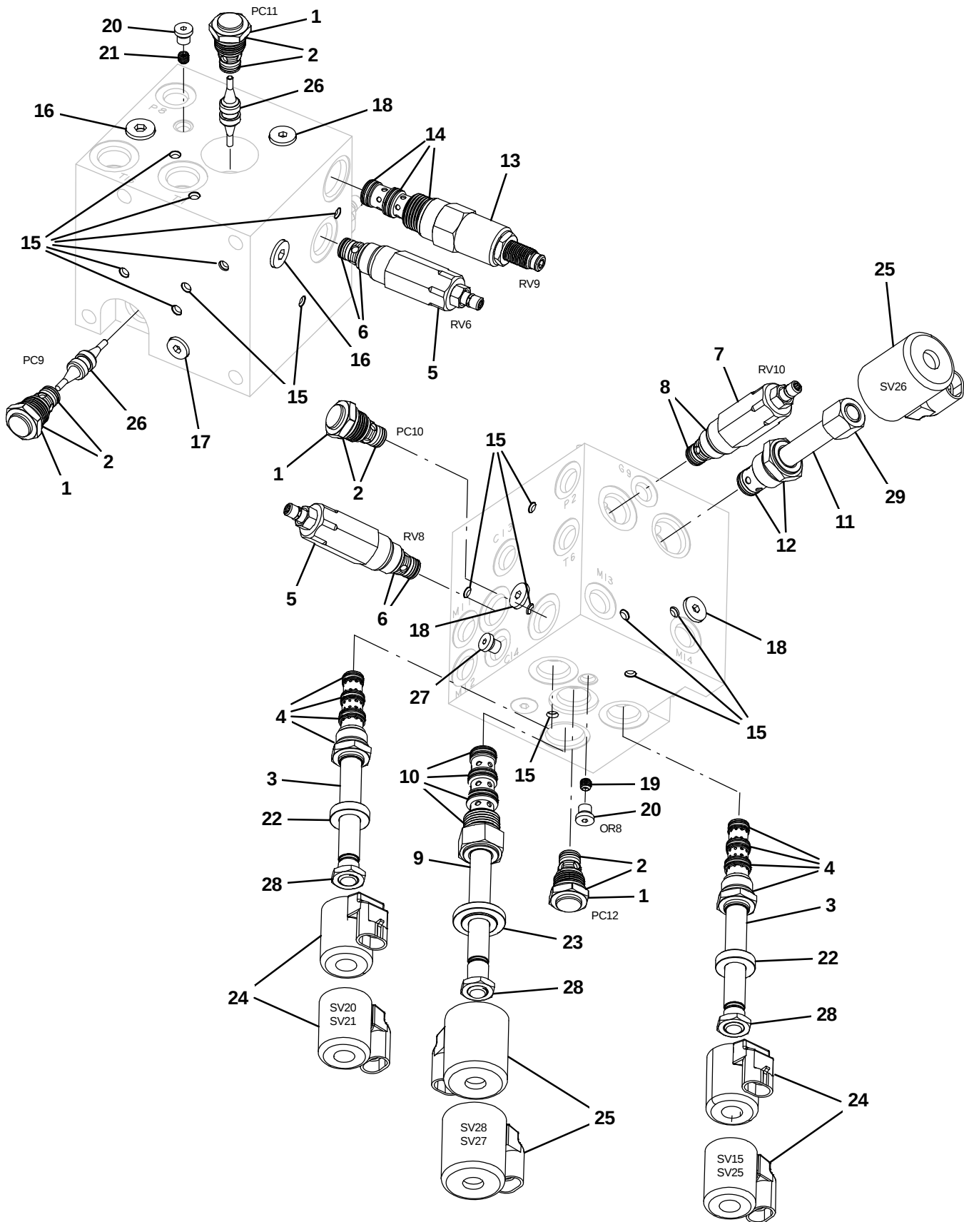
Fig. 29 – Hydraulic Solenoid Valve Breakdown, 1053645
