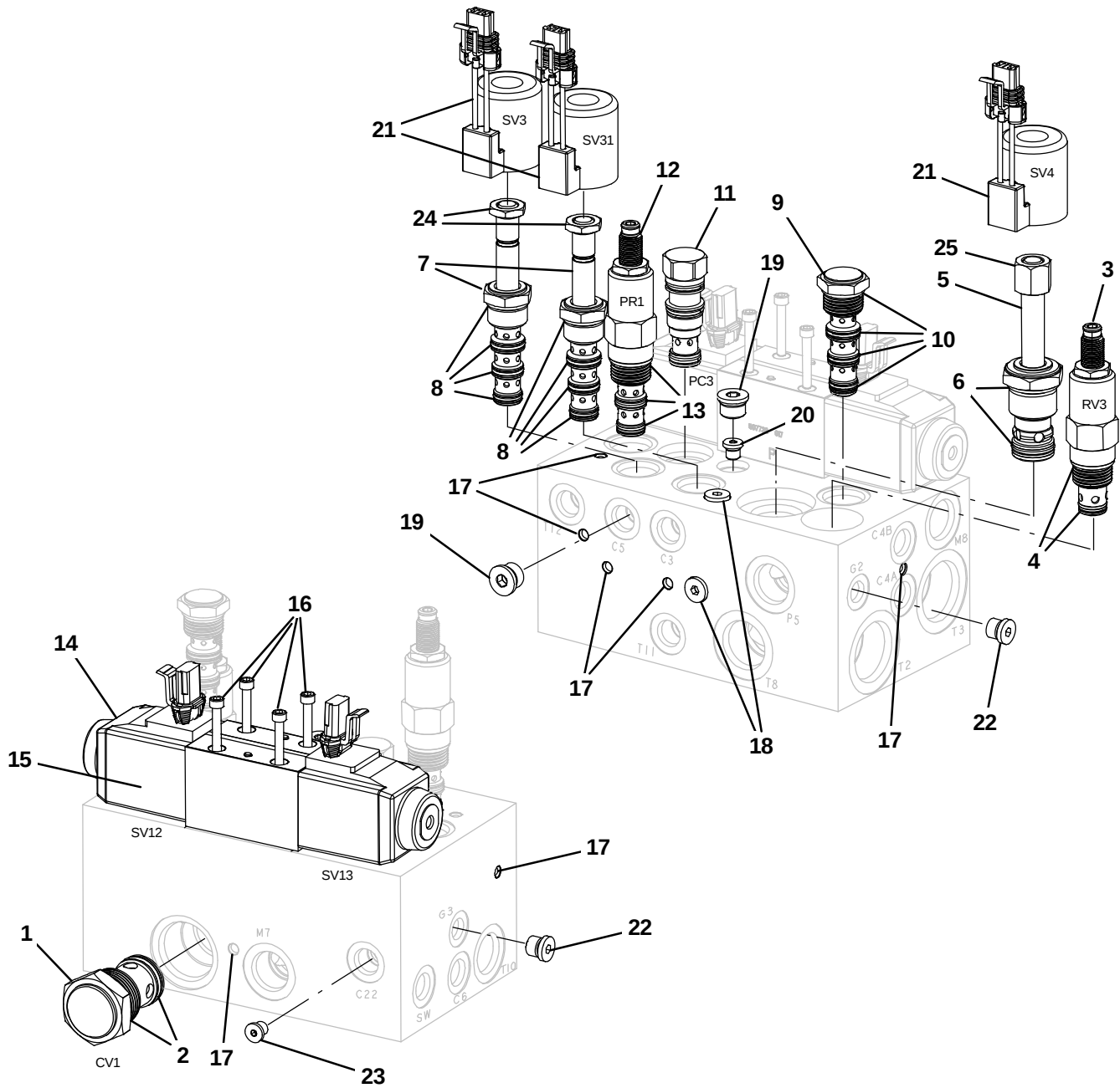
Fig. 26 – Hydraulic Solenoid Valve Breakdown, 1053650
