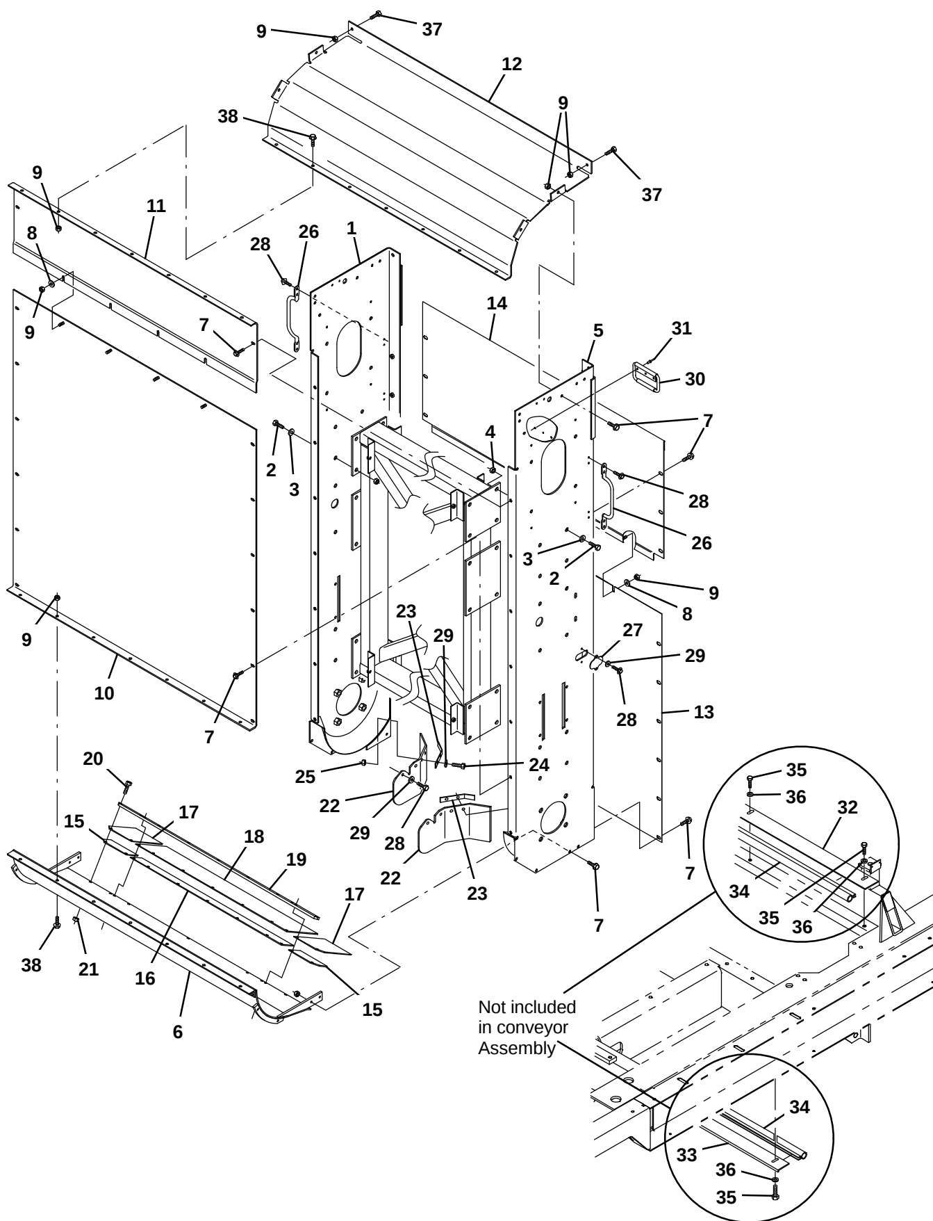
Fig. 28 – Conveyor and Covers Group
