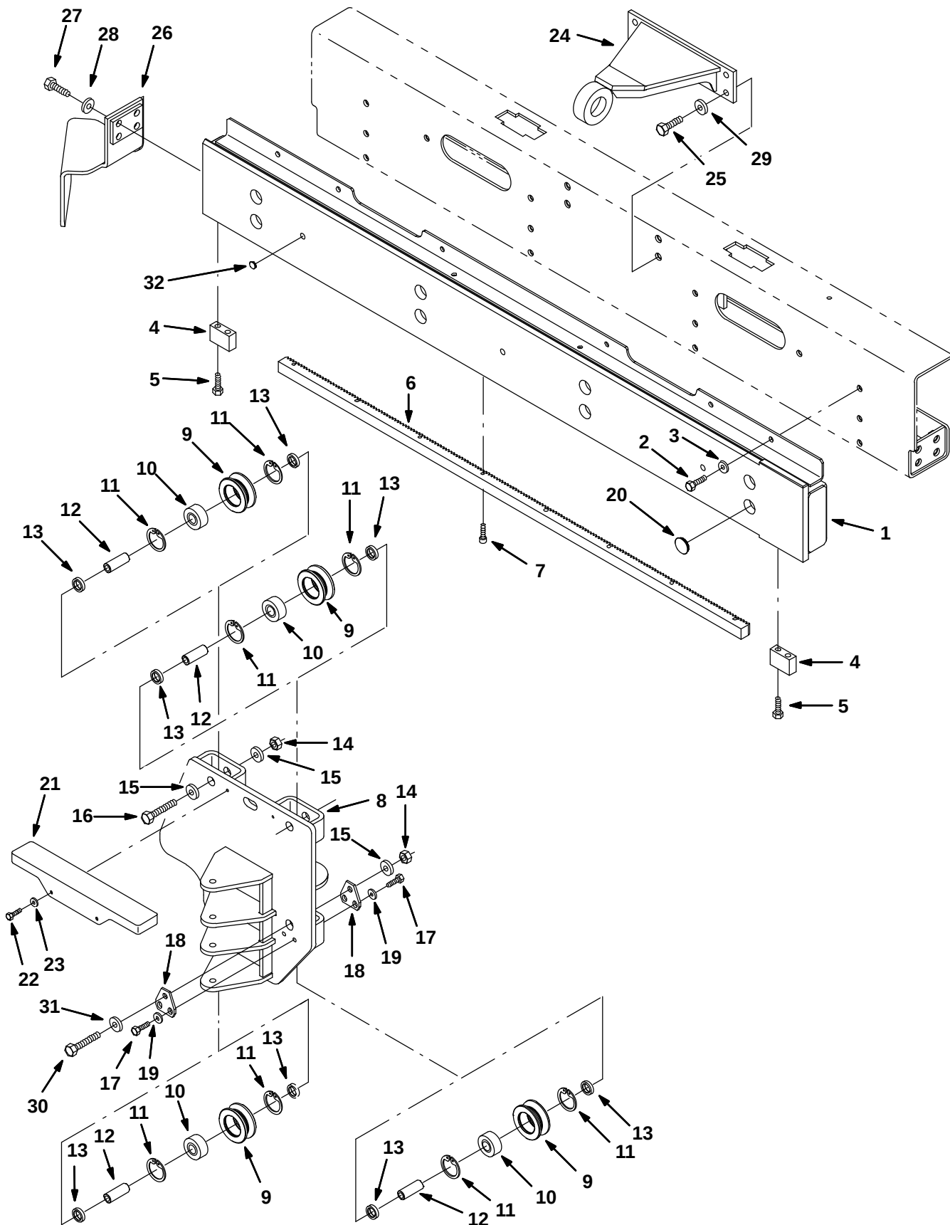
Fig. 7 – Vario Brush Dolly Group
