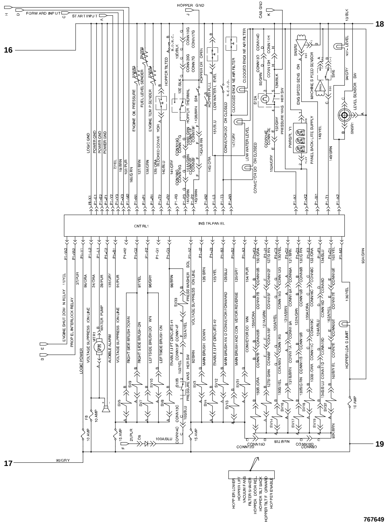
Fig. 75 – Electrical Schematic (000000-008499)
