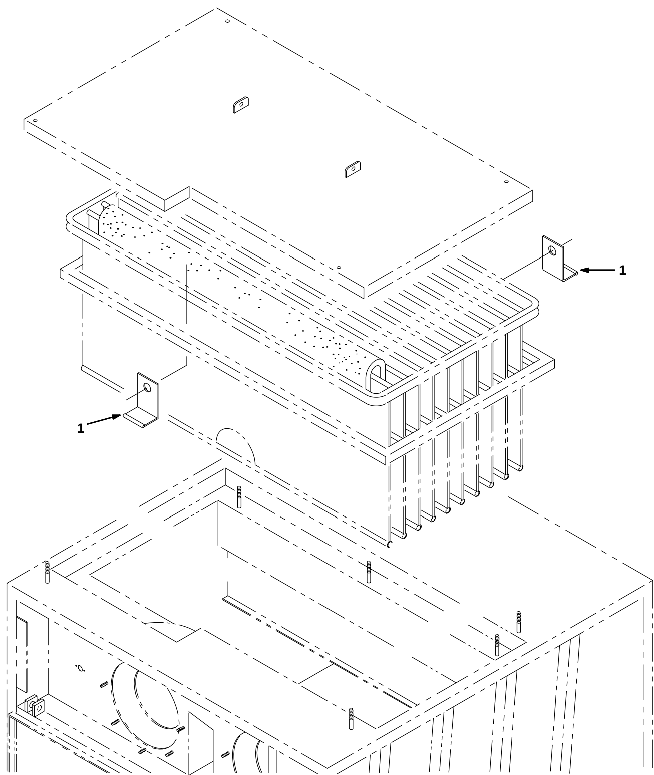
Fig. 30 – Filter Bag Lift Kit
