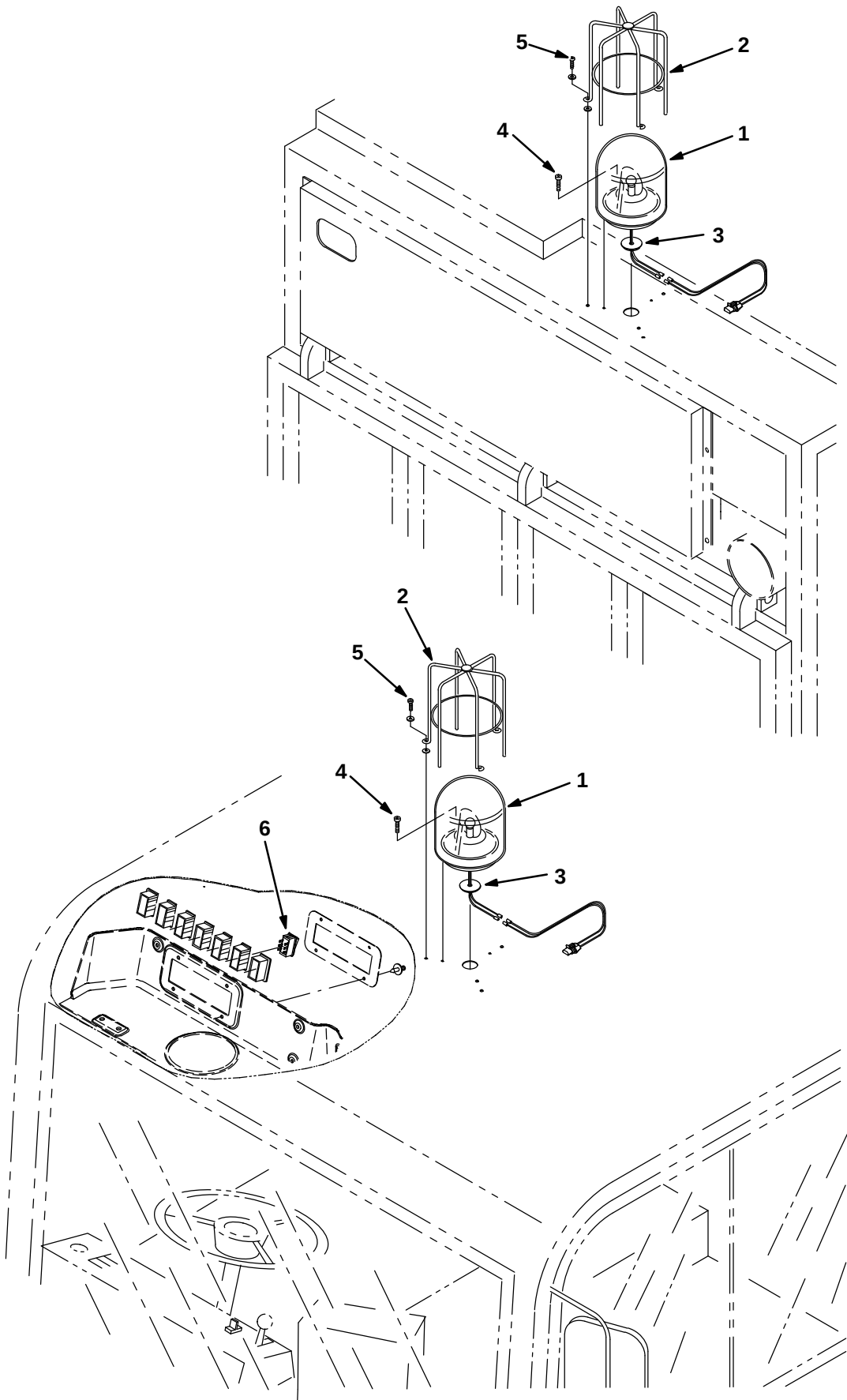
Fig. 35 – Light Kit, Revolving
