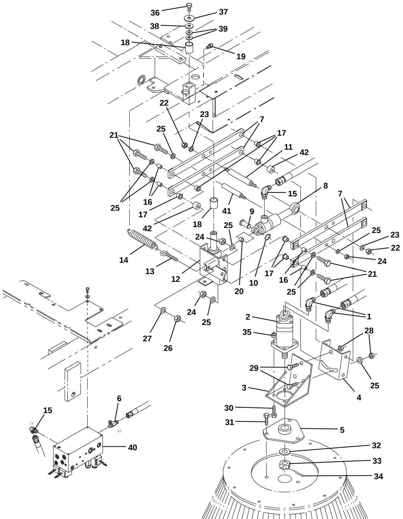
Fig. 5 – Left Side Brush Group (009838- )
