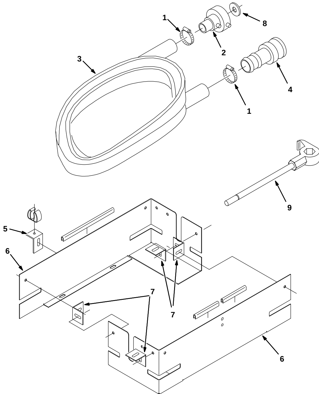
Fig. 32 – Hydrant Hose Group
