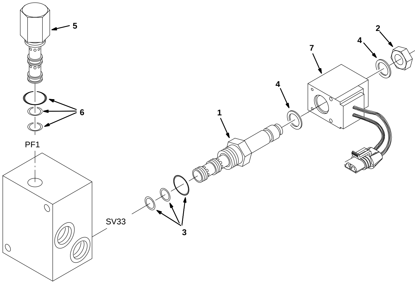
Fig. 16 – Hydraulic Solenoid Valve Breakdown, 767009
