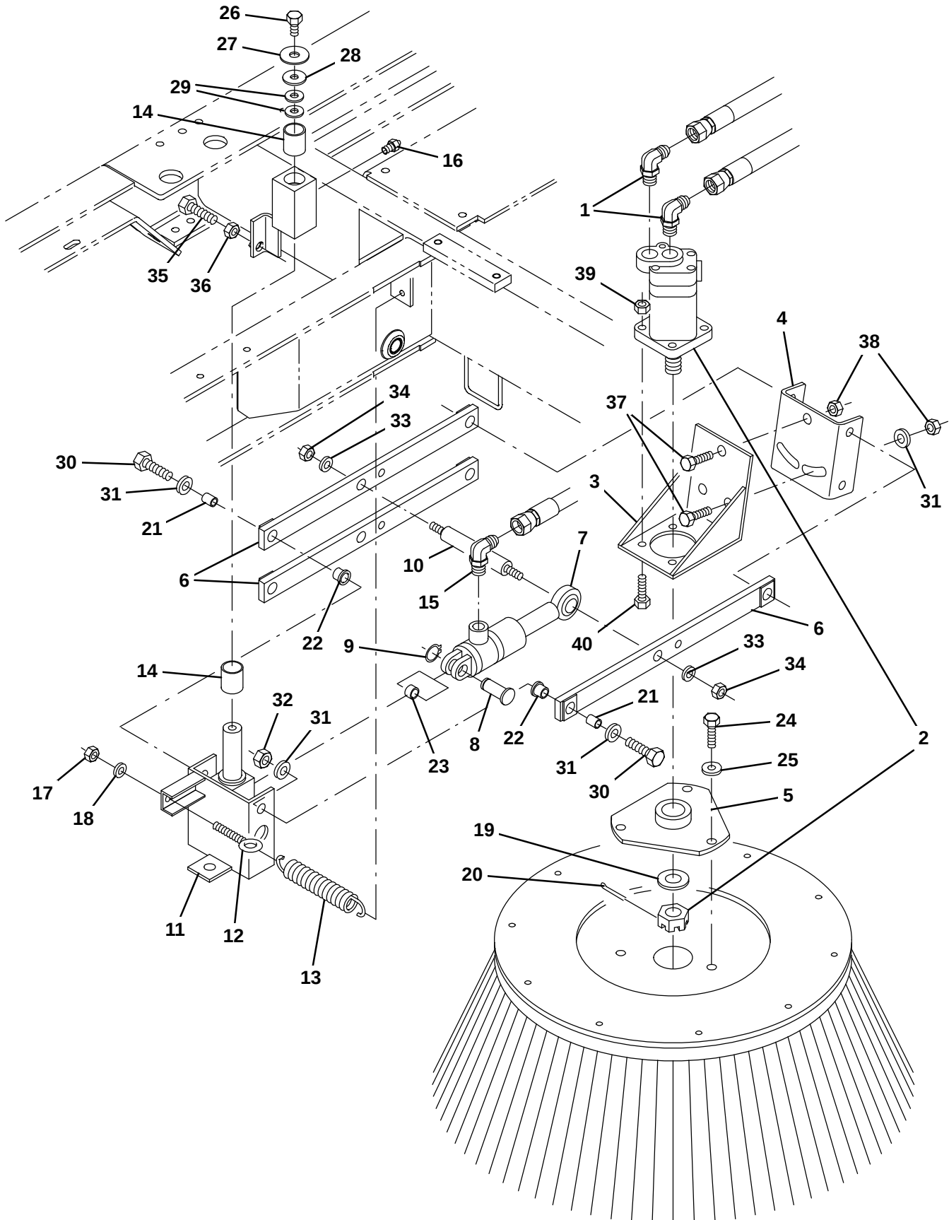
Fig. 53 – Brush Group, Right Side (000000–009837)
