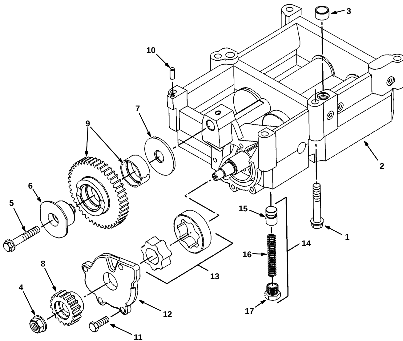
Fig. 1 – Balancer Group
