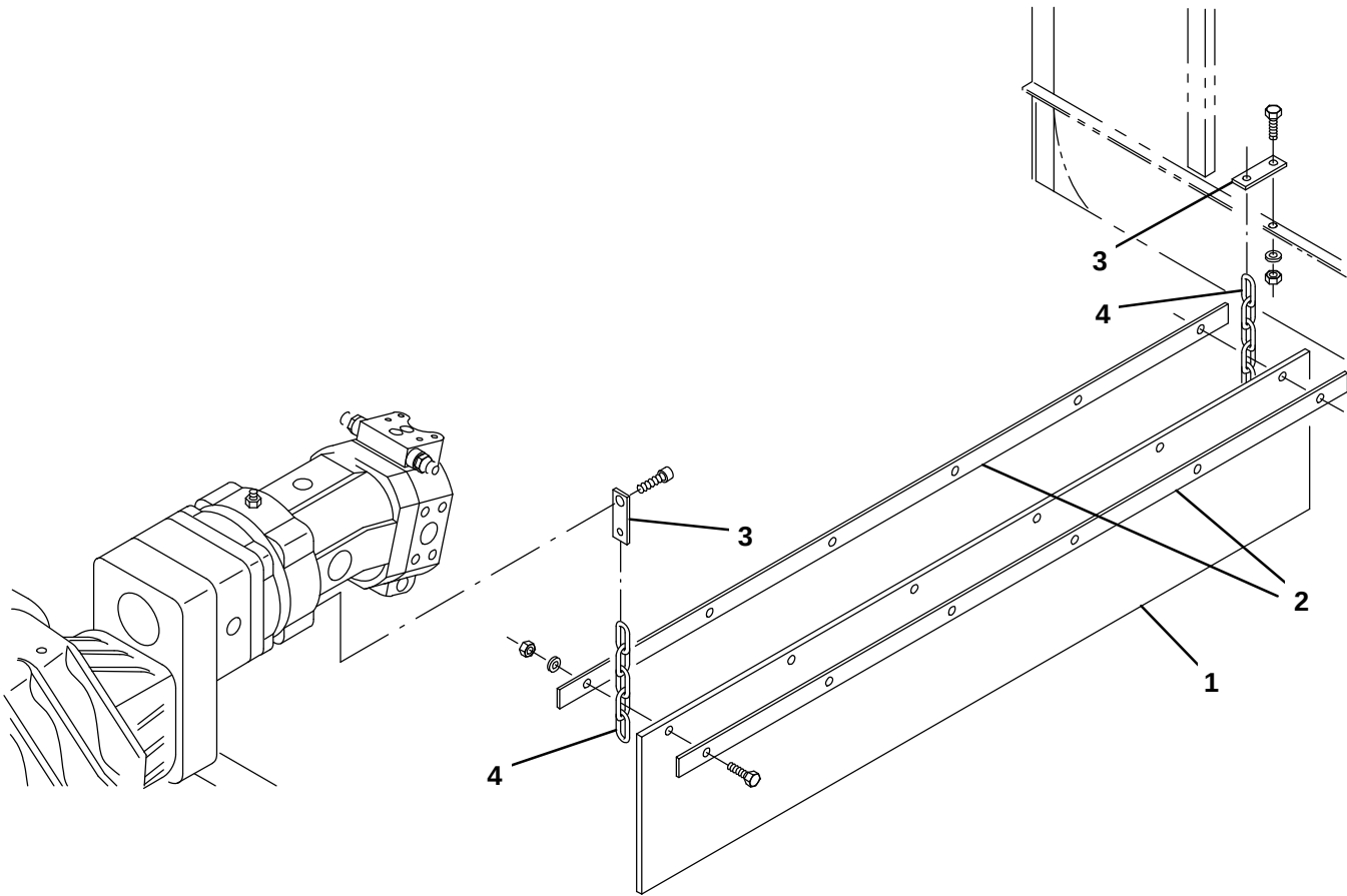
Fig. 72 – Wet Dust Control Skirt Group
