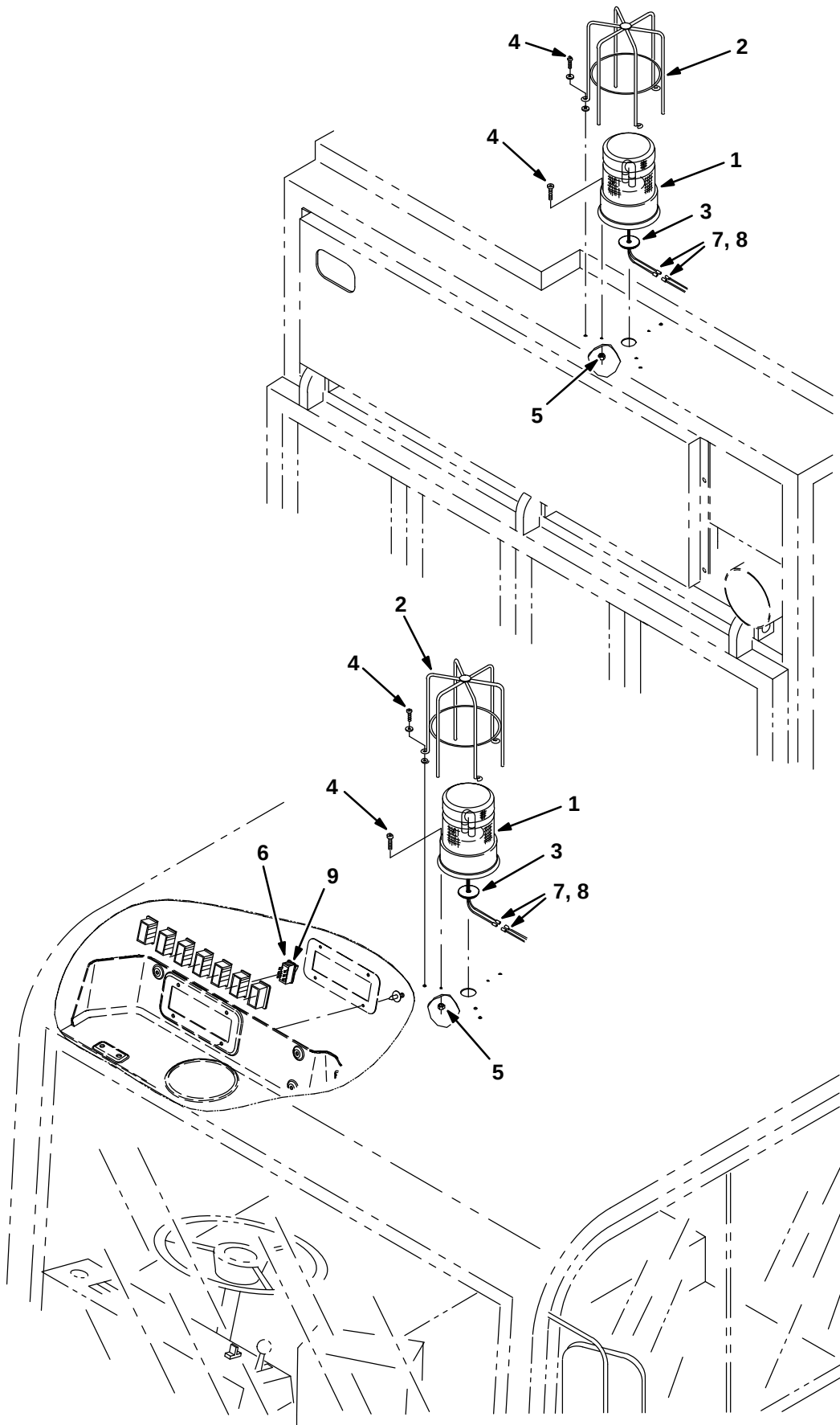
Fig. 36 – Light Kit, Strobe
