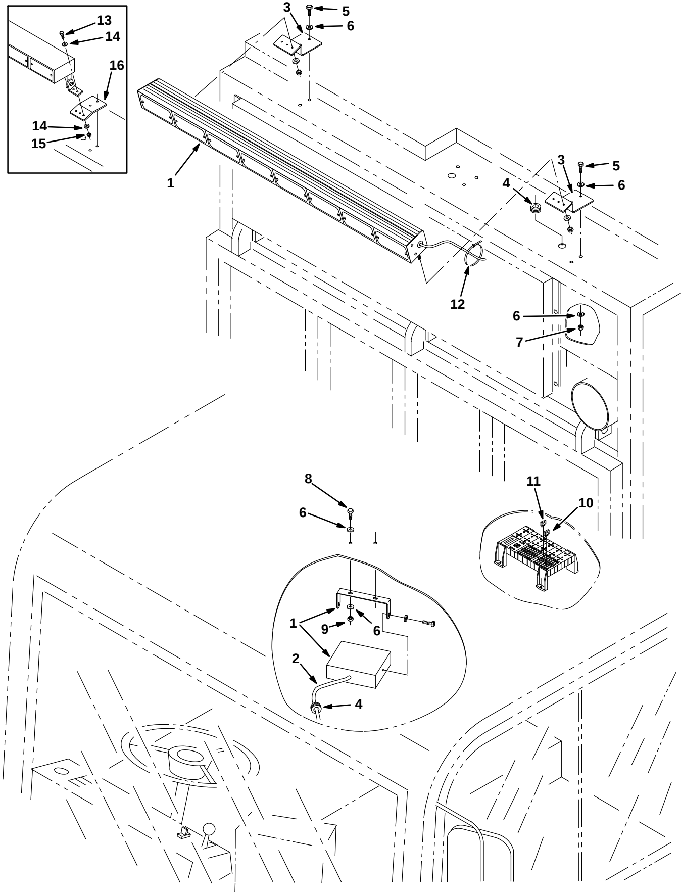
Fig. 37 – Light Kit, Arrow Stick, Without Revolving Light
