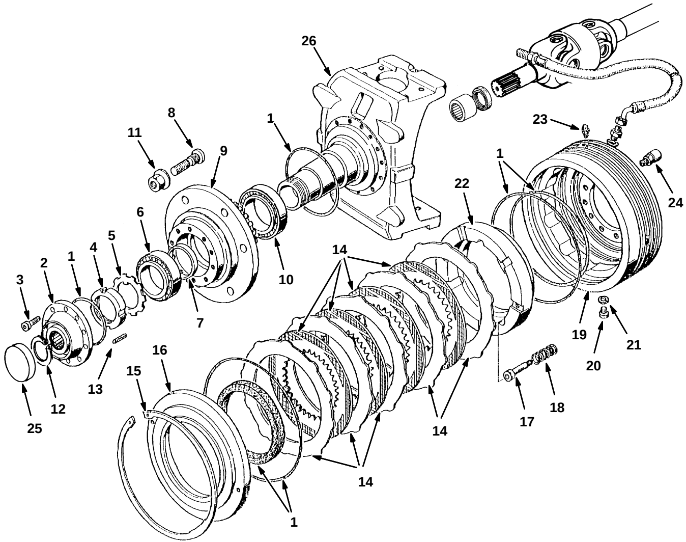
Fig. 7 – Axle Wheel Hub and Brake Breakdown, Front
