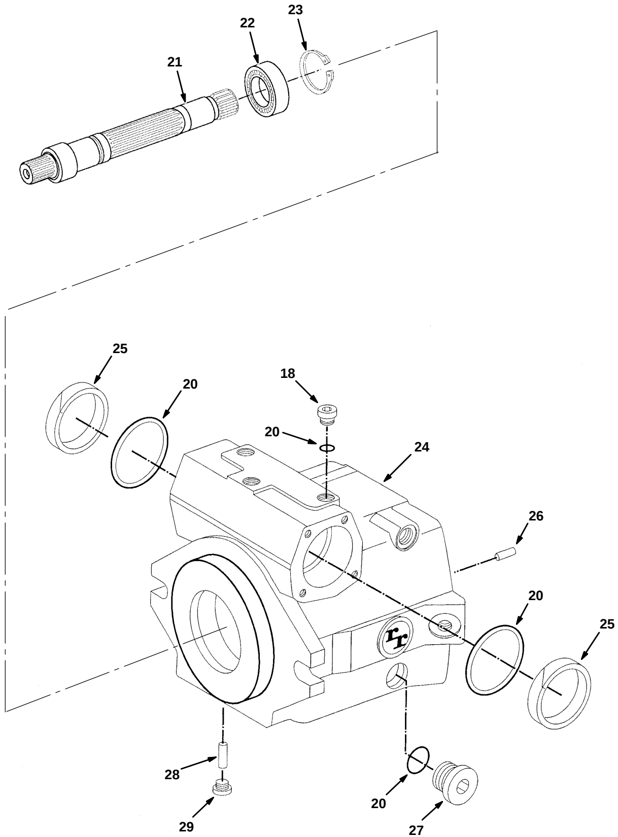
Fig. 2 – Hydraulic Piston Pump Breakdown, 1066392
