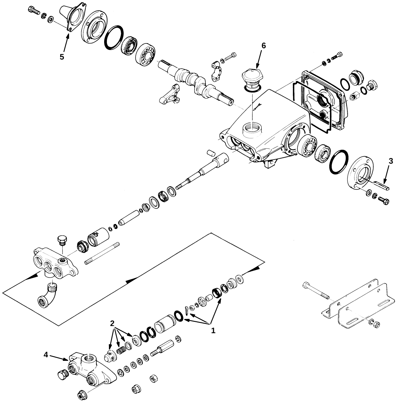
Fig. 13 – Cat Pump Breakdown, 762260
