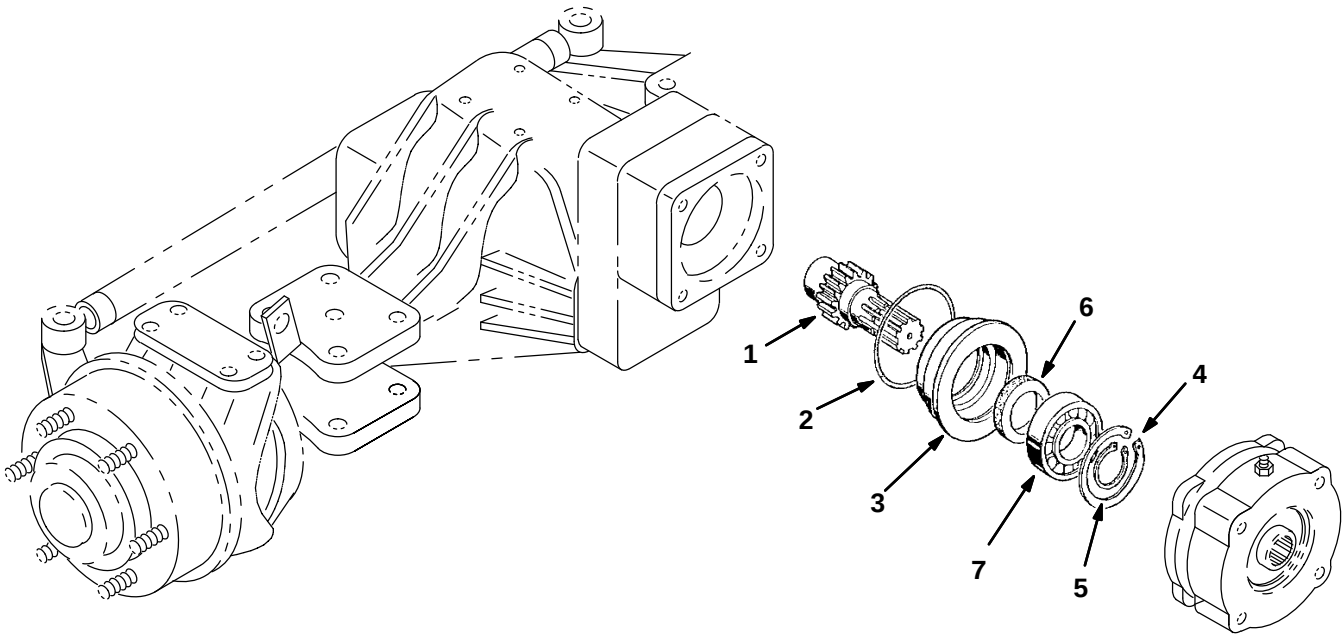
Fig. 9 – Axle Input Breakdown, Front
