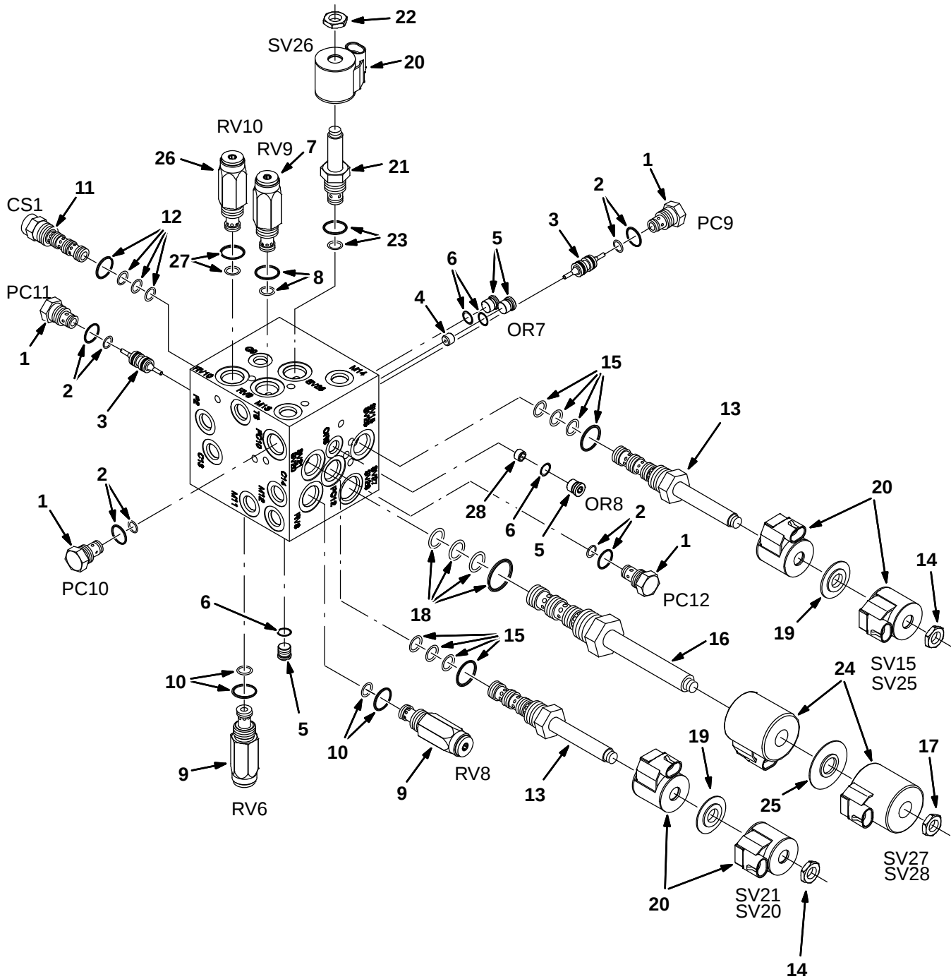
Fig. 22 – Hydraulic Solenoid Valve Breakdown, 771011
