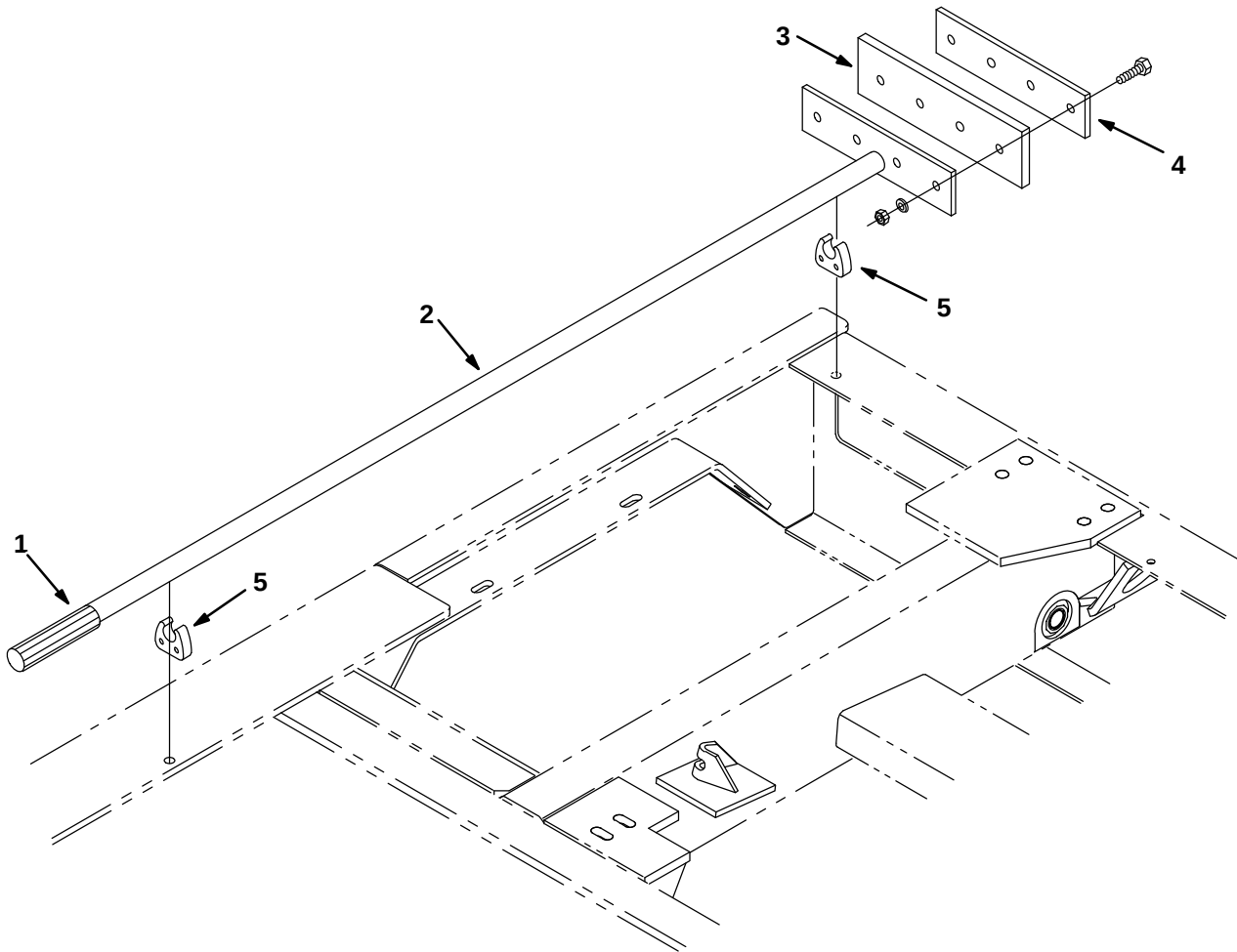
Fig. 25 – Hopper Cleanout Tool Kit
