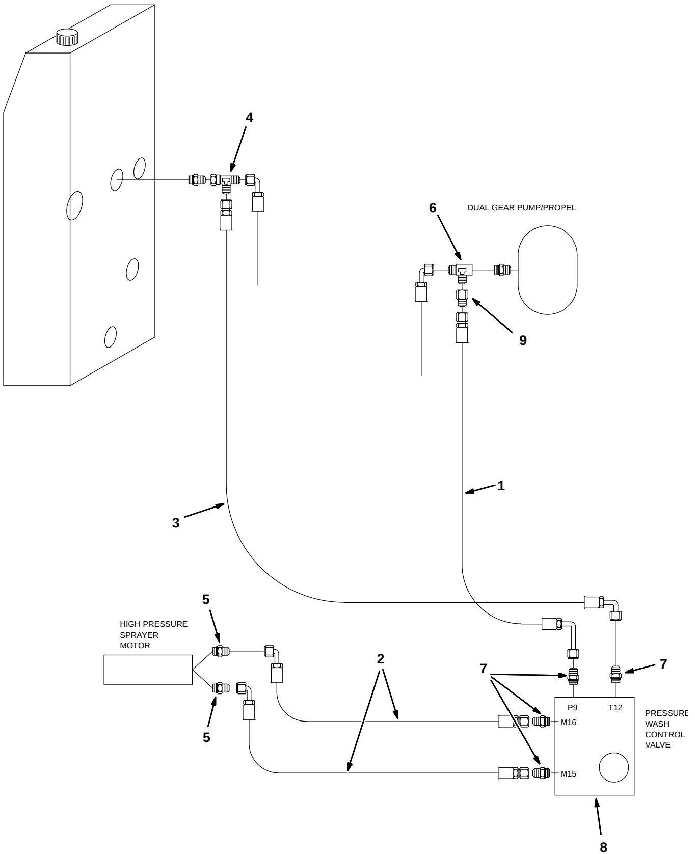
Fig. 17 – High Pressure Sprayer Hydraulic Hose Group
