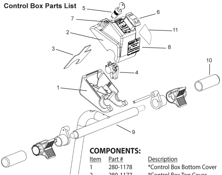
Control Box Parts List
