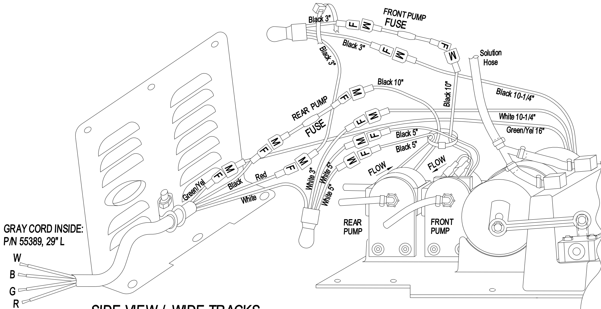
SIDE VIEW / WIDE TRACKS BOTTOM PAN ASSY - 120V JLT PUMPS INSTALLED 2 FUSES
